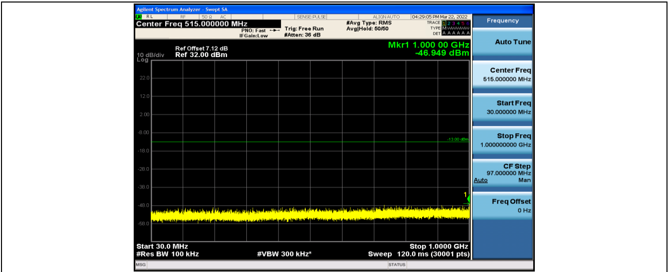
Band2-1.4MHz-QPSK-18607-1RB#0-30~1000MHz
