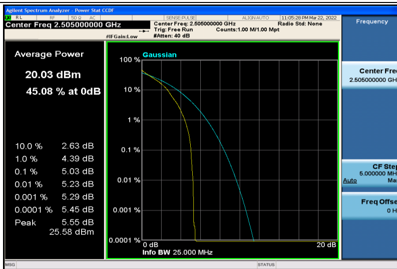
Band7-10MHz-QPSK-20800-1RB#0
