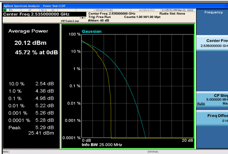
Band7-10MHz-QPSK-21100-1RB#0
