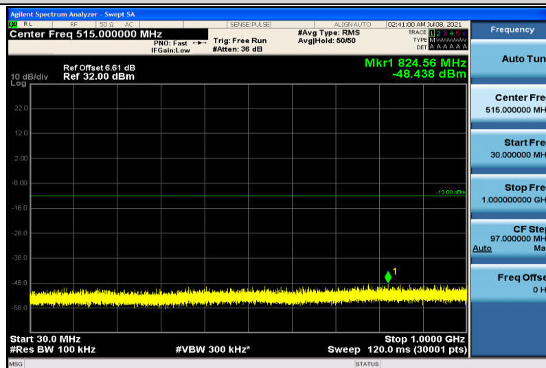
Band4-3MHz-16QAM-20175-1RB#0-30~1000MHz
