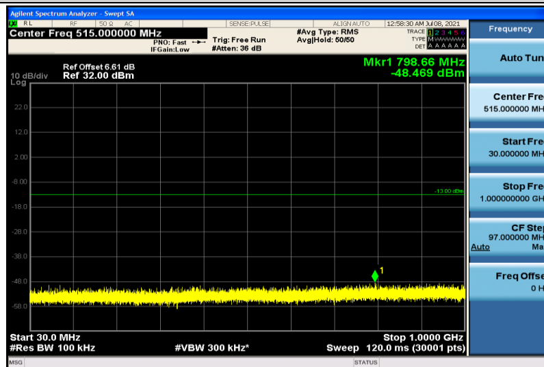
Band2-10MHz-16QAM-19150-1RB#0-30~1000MHz
