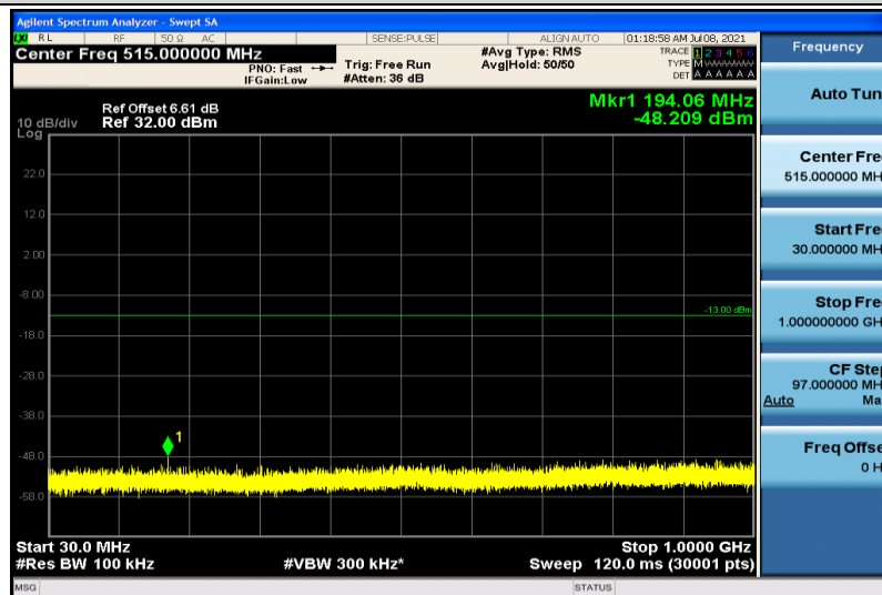
Band2-15MHz-16QAM-19125-1RB#0-30~1000MHz
