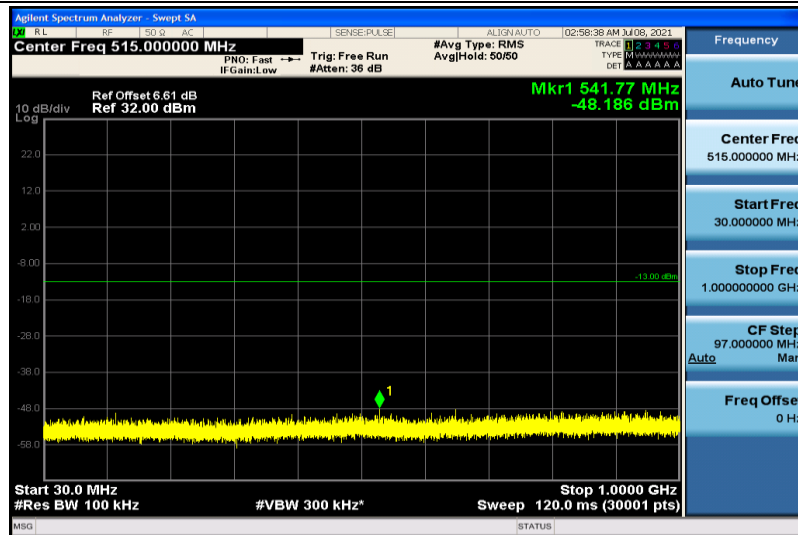
Band4-5MHz-16QAM-19975-1RB#0-30~1000MHz
