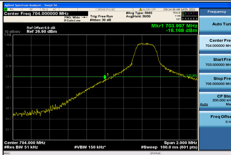
Band17-5MHz-QPSK-23755-1RB#0
