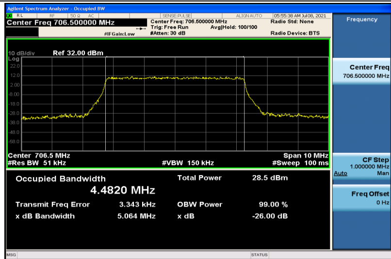
Band17-5MHz-16QAM-23755-25RB#0-4.4820
