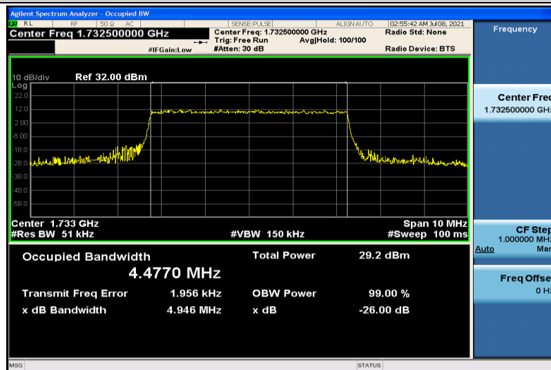
Band4-5MHz-16QAM-20175-25RB#0-4.4770
