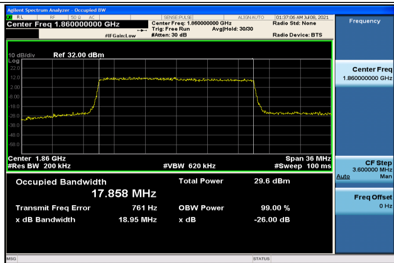
Band2-20MHz-16QAM-18700-100RB#0-17.858
