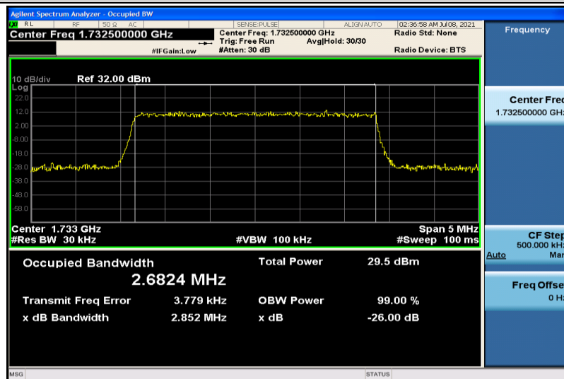
Band4-3MHz-QPSK-20175-15RB#0-2.6824
