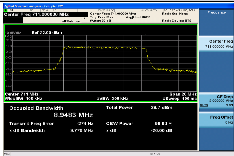
Band17-10MHz-16QAM-23800-50RB#0-8.9483
