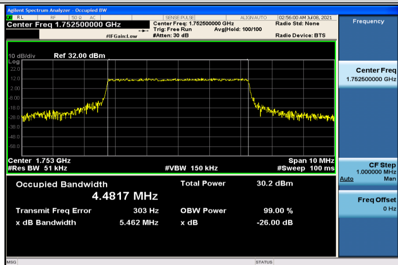
Band4-5MHz-QPSK-17525-25RB#0-4.4817
