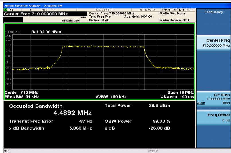
Band17-5MHz-16QAM-23790-25RB#0-4.4892
