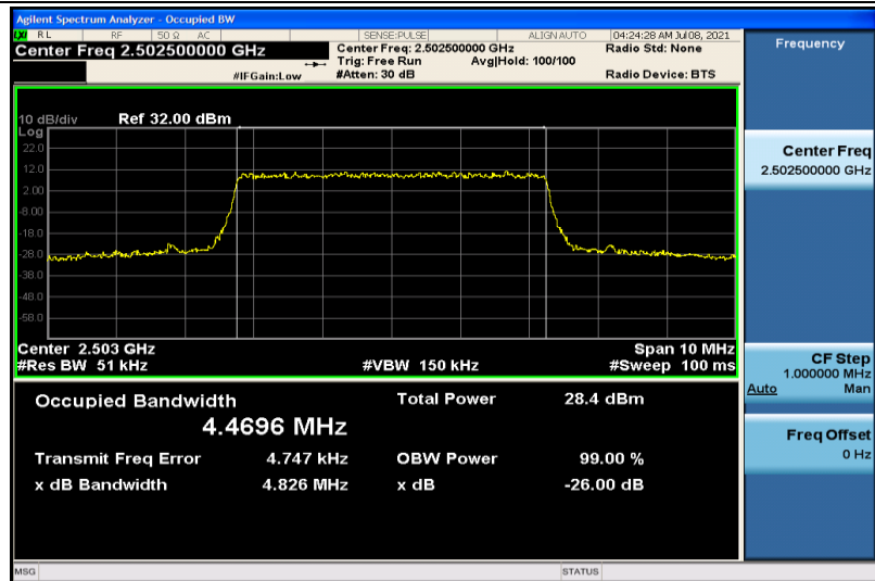
Band7-5MHz-16QAM-20775-25RB#0-4.4696
