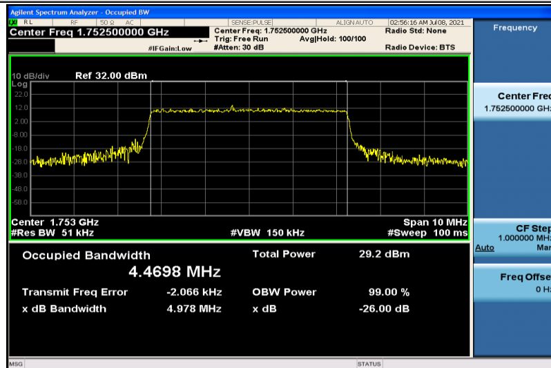
Band4-5MHz-16QAM-20375-25RB#0-4.4698
