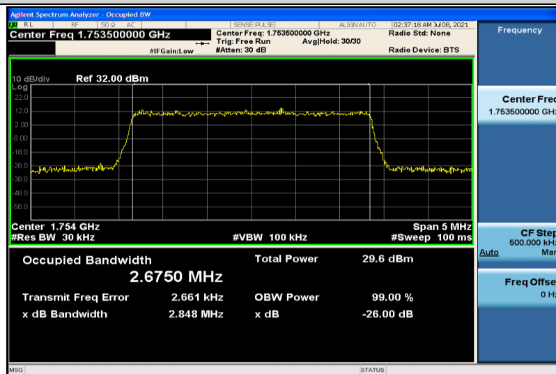
Band4-3MHz-QPSK-20385-15RB#0-2.6750
