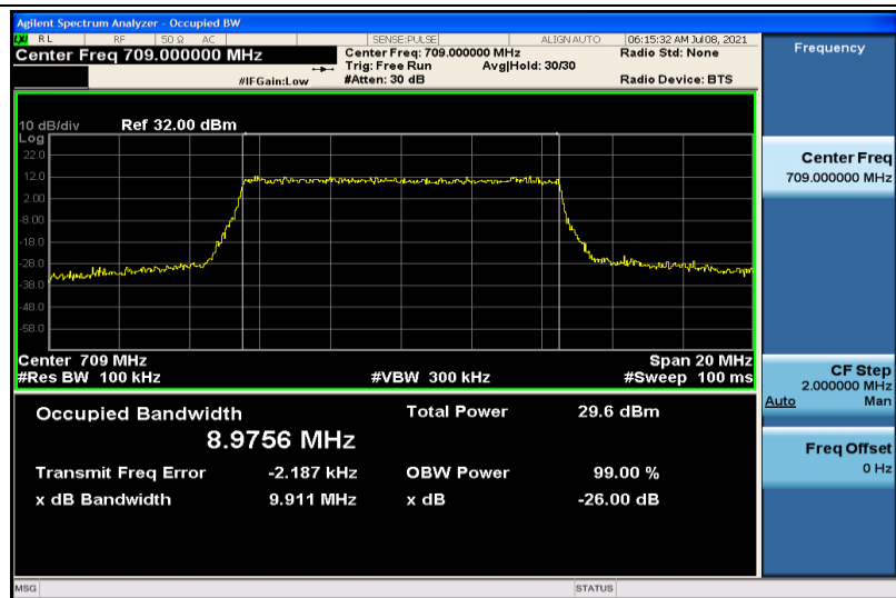
Band17-10MHz-QPSK-23780-50RB#0-8.9756
