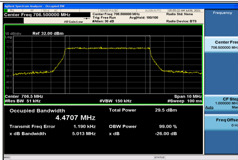
Band17-5MHz-QPSK-23755-25RB#0-4.4707
