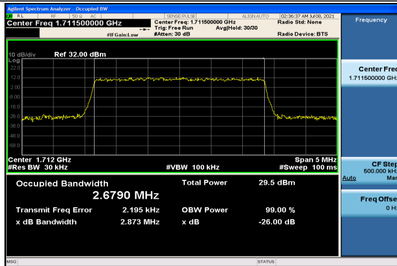
Band4-3MHz-QPSK-19965-15RB#0-2.6790
