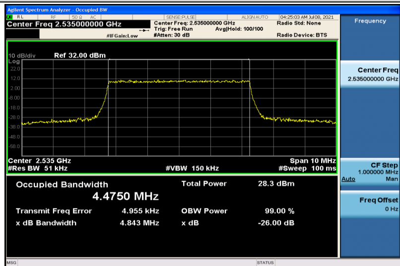
Band7-5MHz-16QAM-21100-25RB#0-4.4750
