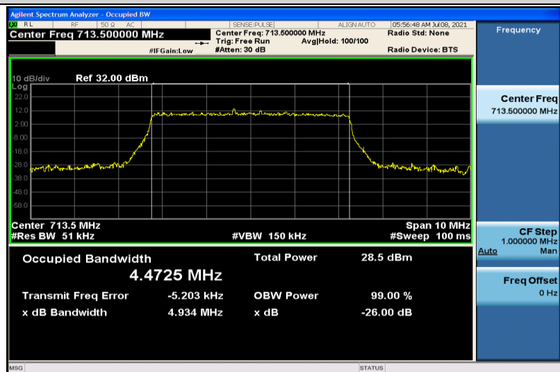
Band17-5MHz-16QAM-23825-25RB#0-4.4725
