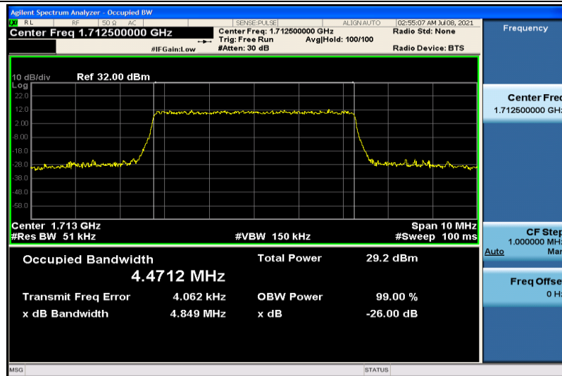
Band4-5MHz-16QAM-19975-25RB#0-4.4712
