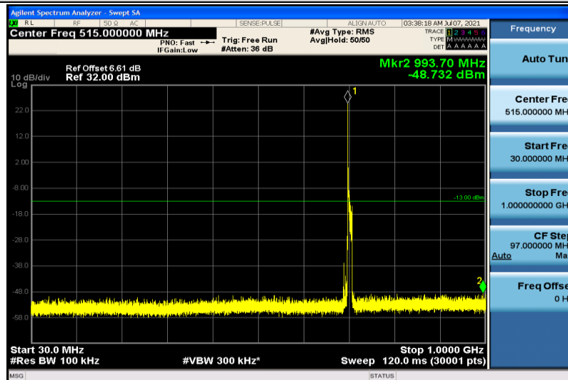
Band17-10MHz-QPSK-23790-1RB#0-30~1000MHz
