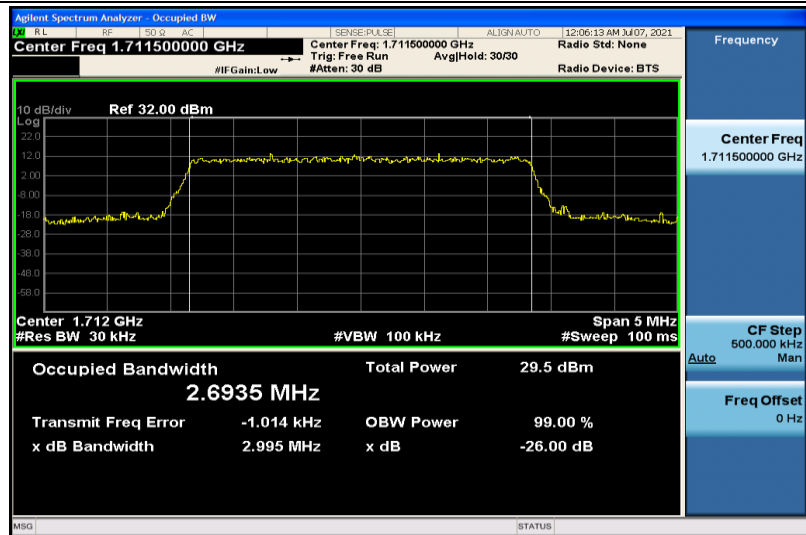
Band4-3MHz-16QAM-19965-15RB#0-2.6935
