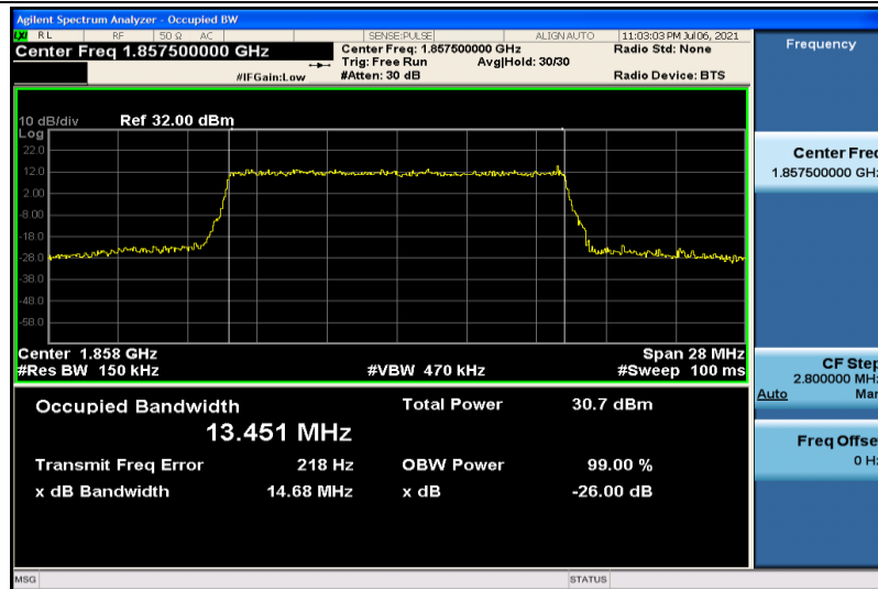
Band2-15MHz-16QAM-18675-75RB#0-13.451
