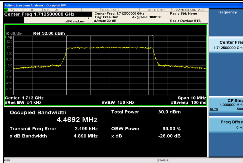
Band4-5MHz-QPSK-19975-25RB#0-4.4692
