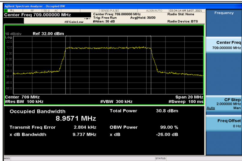
Band17-10MHz-QPSK-23780-50RB#0-8.9571
