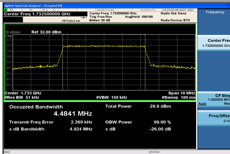
Band4-5MHz-16QAM-20175-25RB#0-4.4841
