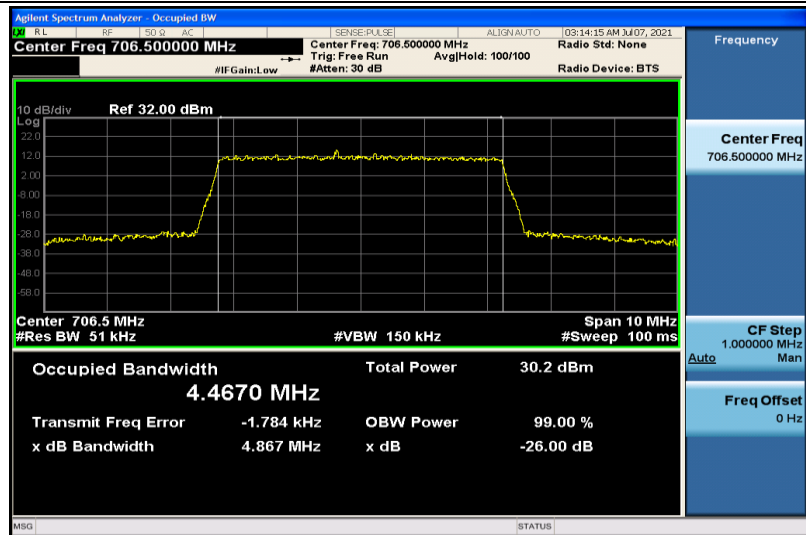
Band17-5MHz-16QAM-23755-25RB#0-4.4670
