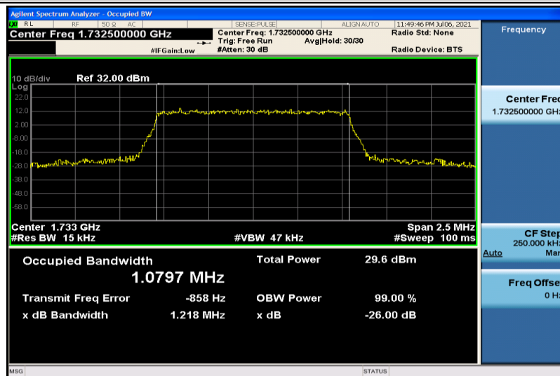
Band4-1.4MHz-QPSK-20175-6RB#0-1.0797
