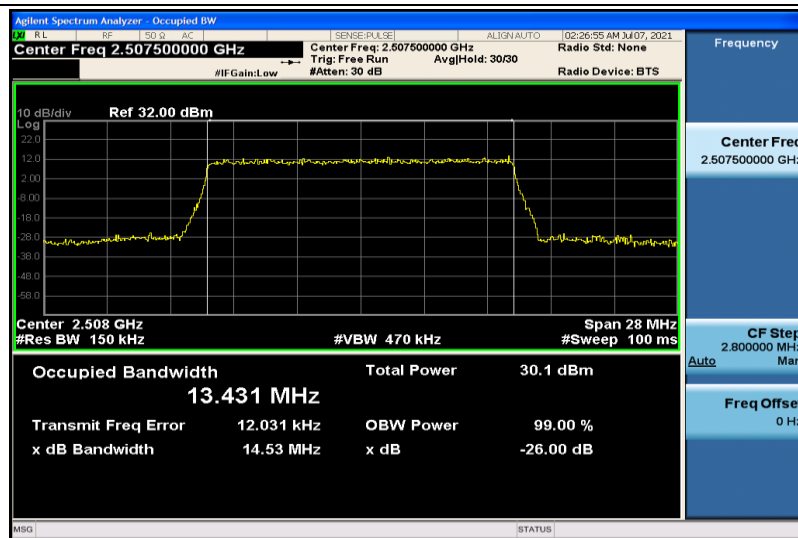
Band7-15MHz-16QAM-20825-75RB#0-13.431
