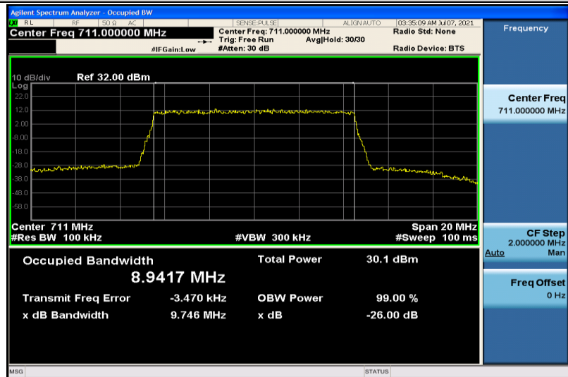
Band17-10MHz-16QAM-23800-50RB#0-8.9417
