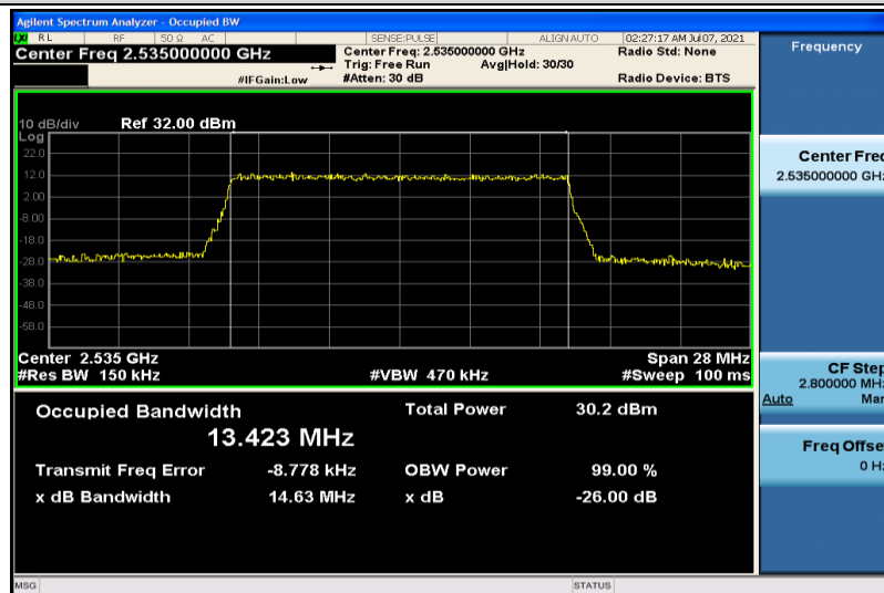
Band7-15MHz-16QAM-21100-75RB#0-13.423
