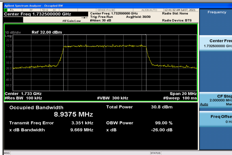
Band4-10MHz-QPSK-20175-50RB#0-8.9375
