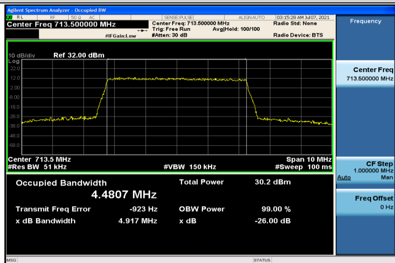
Band17-5MHz-16QAM-23825-25RB#0-4.4807
