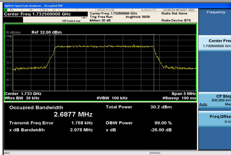
Band4-3MHz-QPSK-1732500000-15RB#0-2.6877
