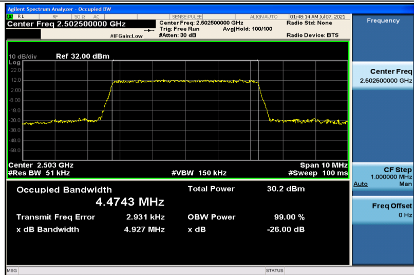
Band7-5MHz-16QAM-20775-25RB#0-4.4743
