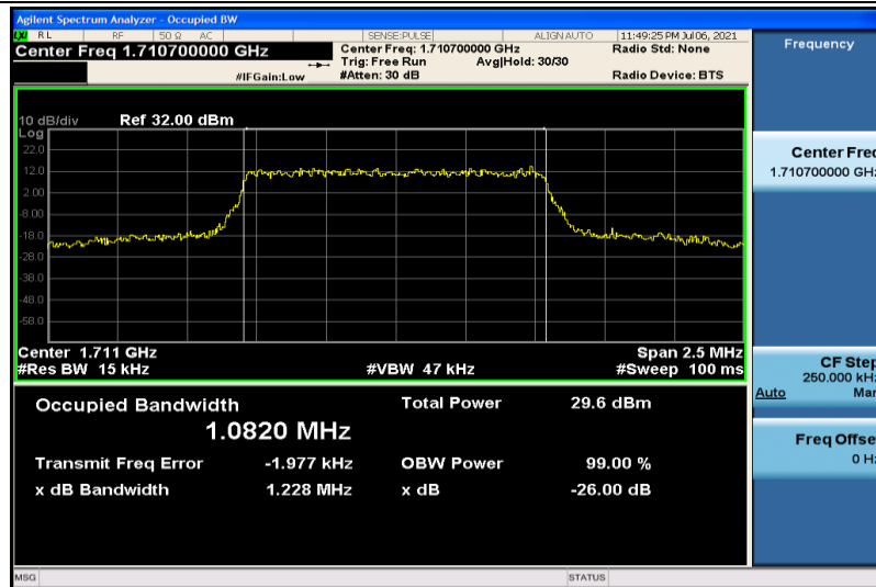
Band4-1.4MHz-QPSK-19957-6RB#0-1.0820
