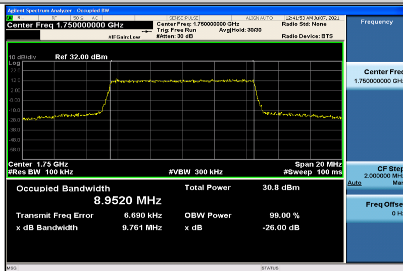
Band4-10MHz-QPSK-20350-50RB#0-8.9520
