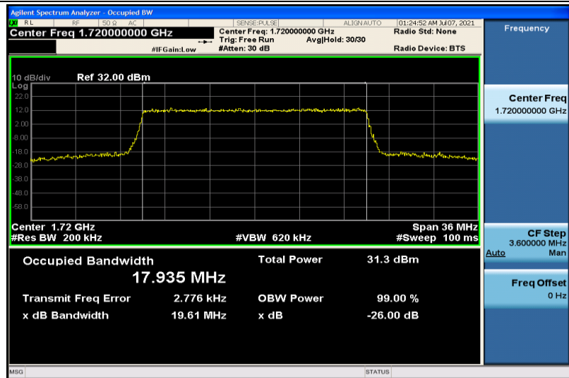
Band4-20MHz-QPSK-20050-100RB#0-17.935
