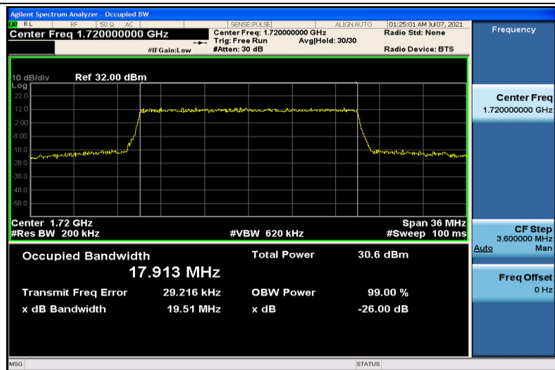
Band4-20MHz-16QAM-20050-100RB#0-17.913
