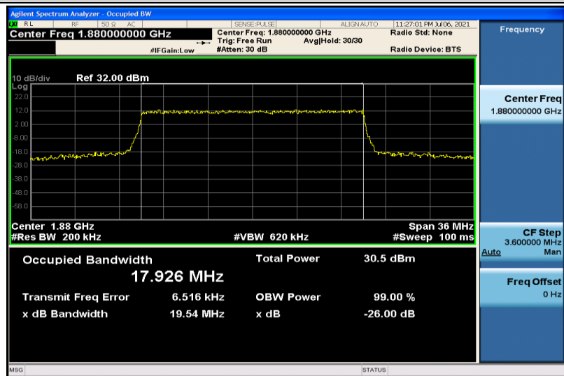
Band2-20MHz-16QAM-18900-100RB#0-17.926
