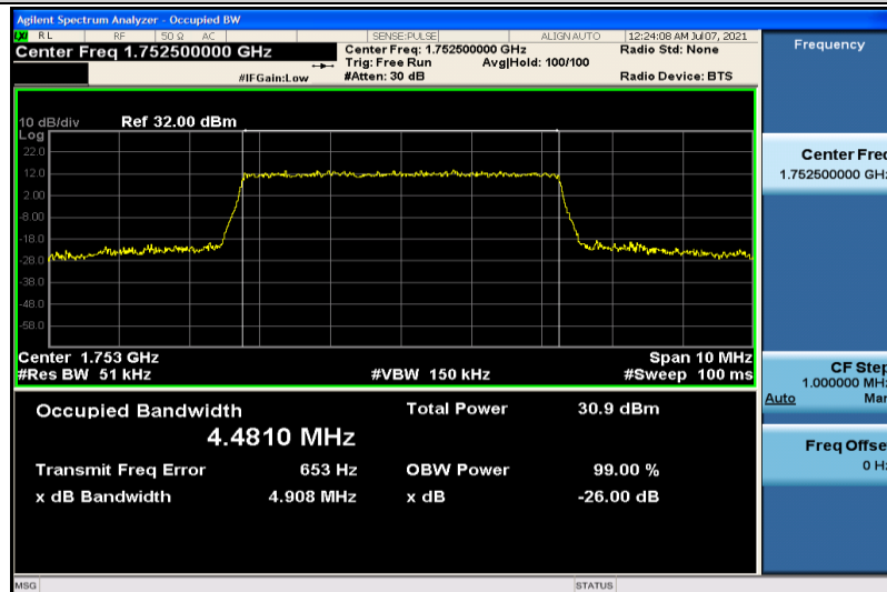
Band4-5MHz-QPSK-20375-25RB#0-4.4810
