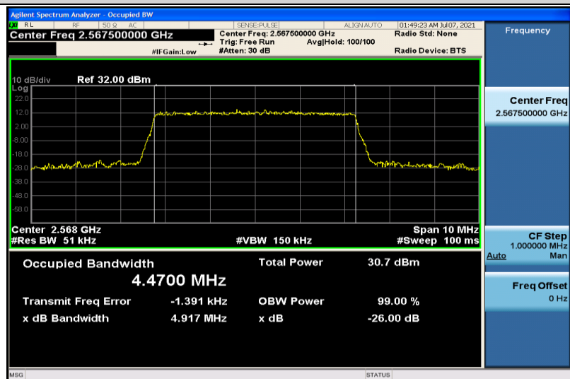
Band7-5MHz-16QAM-21425-25RB#0-4.4700
