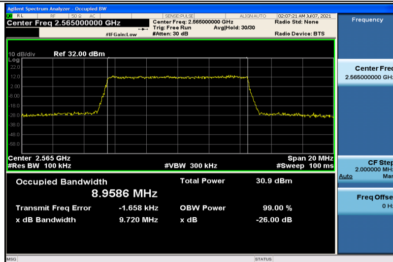
Band7-10MHz-QPSK-21400-50RB#0-8.9586
