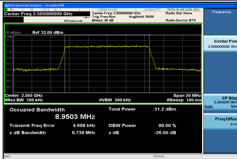
Band7-10MHz-QPSK-20800-50RB#0-8.9503
