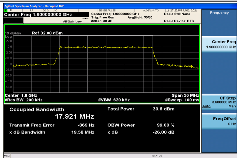
Band2-20MHz-16QAM-19100-100RB#0-17.921
