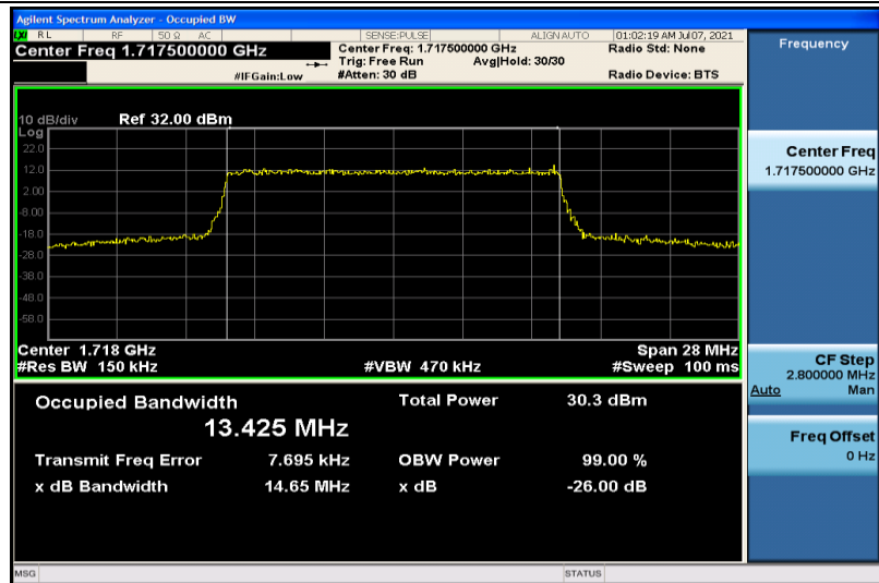
Band4-15MHz-16QAM-20025-75RB#0-13.425
