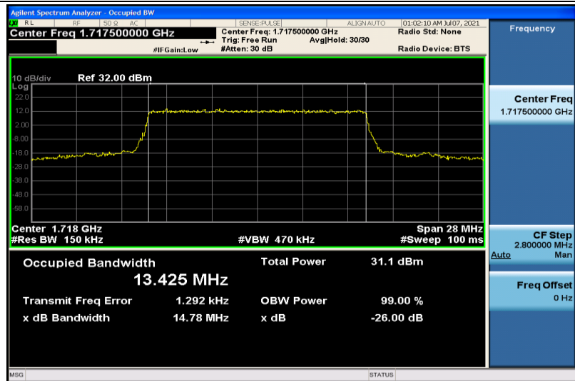
Band4-15MHz-QPSK-20025-75RB#0-13.425
