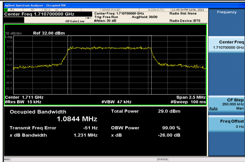
Band4-1.4MHz-16QAM-19957-6RB#0-1.0844
