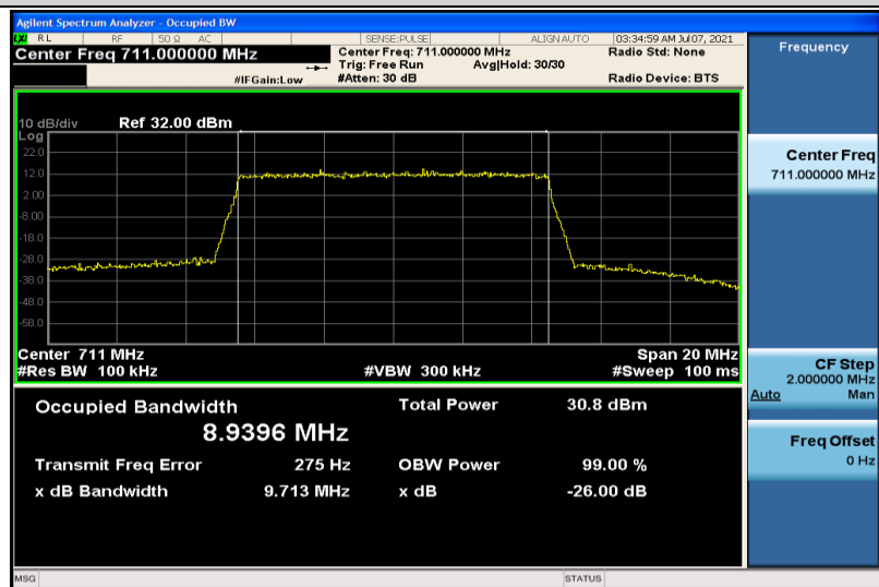
Band17-10MHz-QPSK-23800-50RB#0-8.9396
