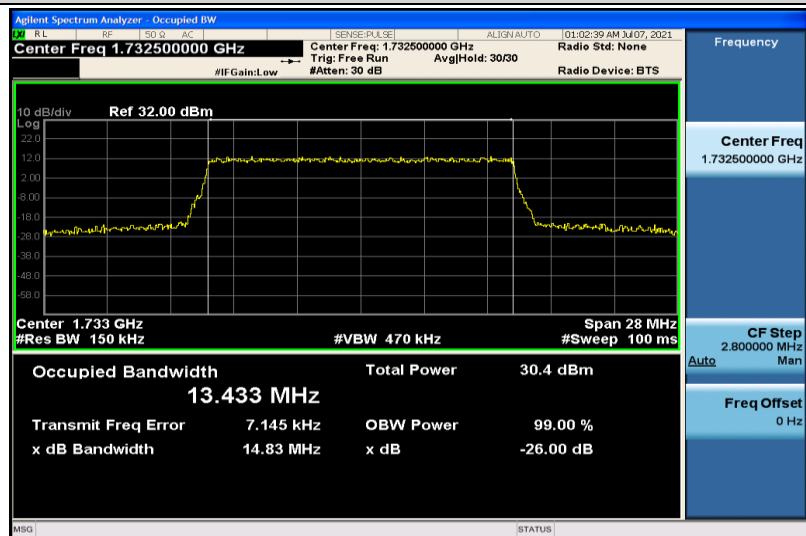
Band4-15MHz-16QAM-20175-75RB#0-13.433
