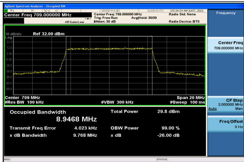
Band17-10MHz-16QAM-23780-50RB#0-8.9468
