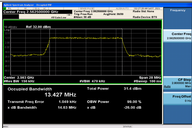
Band7-15MHz-QPSK-21375-75RB#0-13.427
