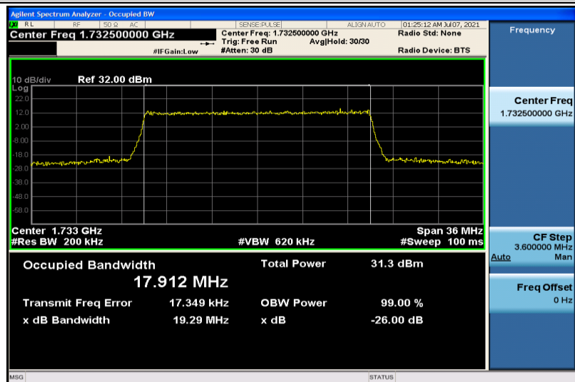
Band4-20MHz-QPSK-20175-100RB#0-17.912
