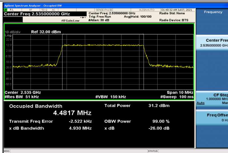
Band7-5MHz-QPSK-21100-25RB#0-4.4817
