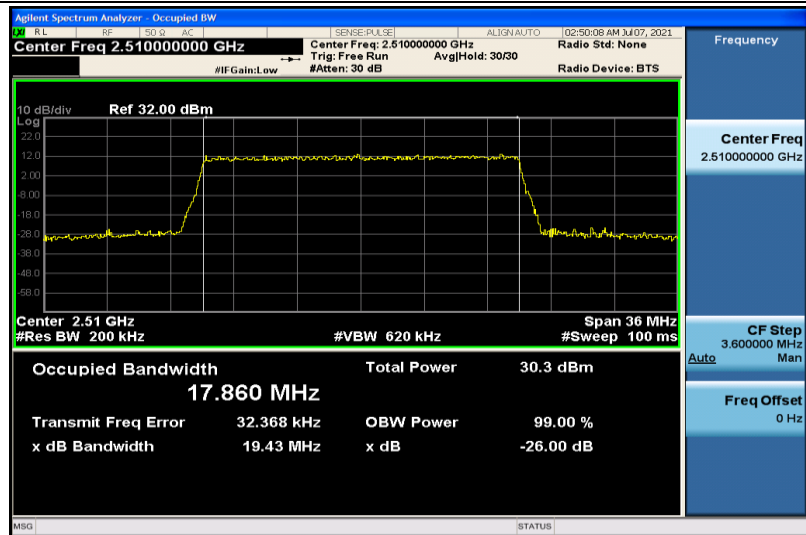
Band7-20MHz-16QAM-20850-100RB#0-17.860
