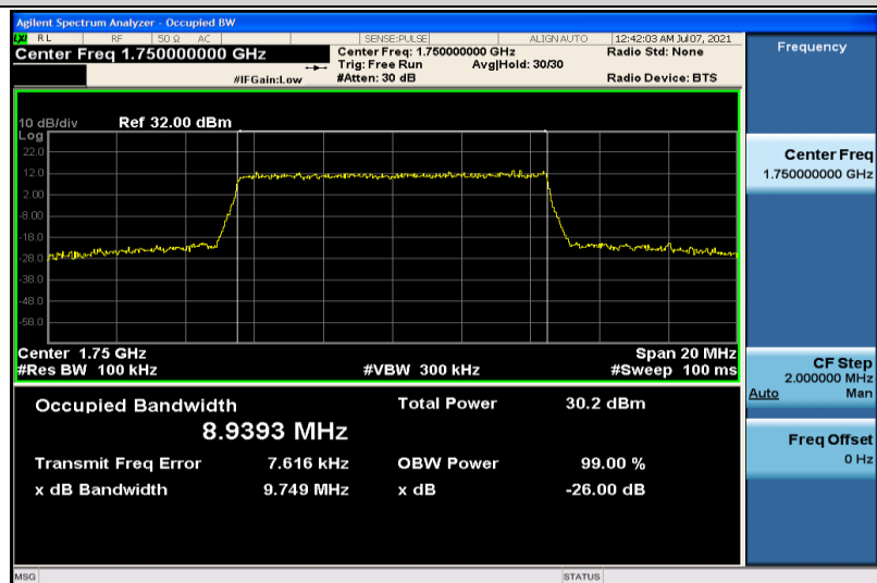
Band4-10MHz-16QAM-20350-50RB#0-8.9393
