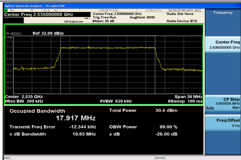
Band7-20MHz-16QAM-21100-100RB#0-17.917
