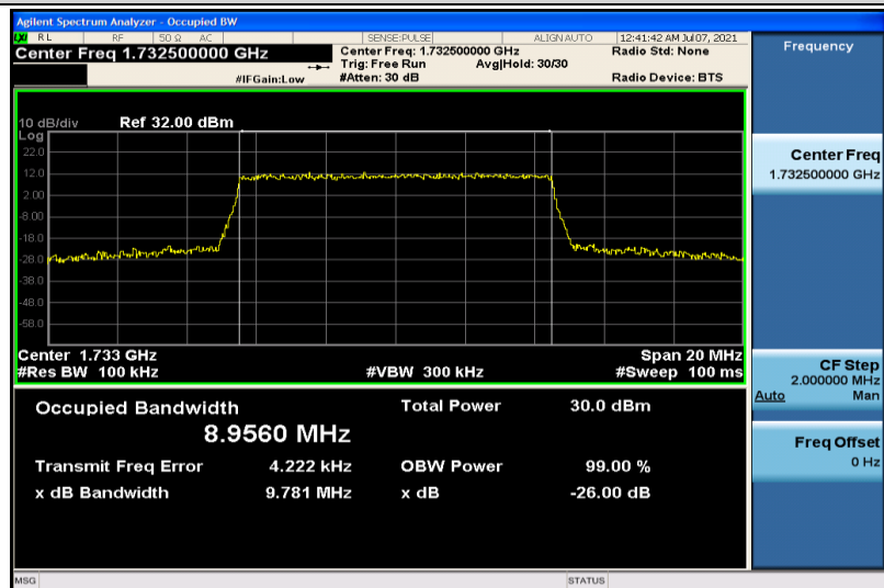
Band4-10MHz-16QAM-20175-50RB#0-8.9560
