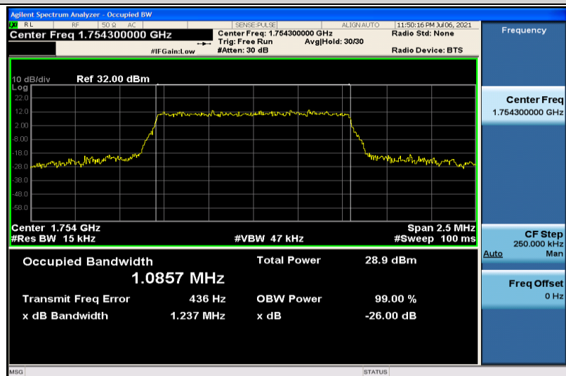
Band4-1.4MHz-16QAM-20393-6RB#0-1.0857
