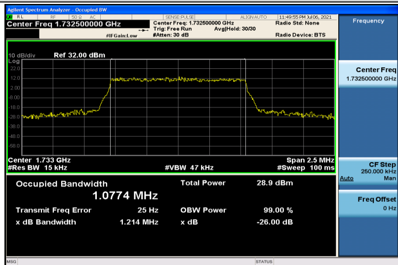
Band4-1.4MHz-16QAM-20175-6RB#0-1.0774
