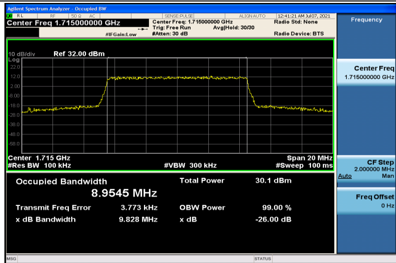
Band4-10MHz-16QAM-20000-50RB#0-8.9545
