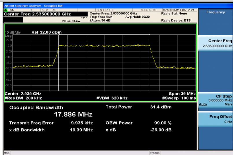
Band7-20MHz-QPSK-21100-100RB#0-17.886
