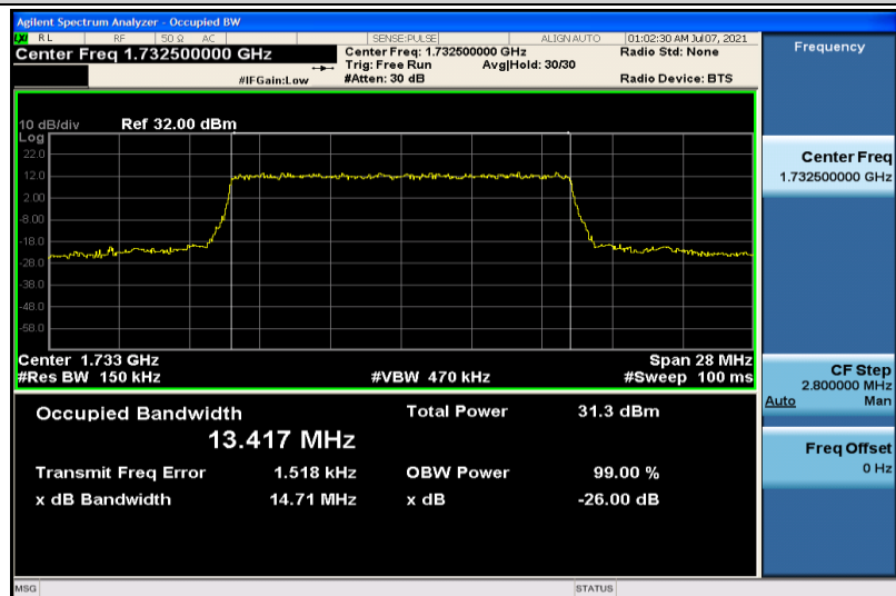
Band4-15MHz-QPSK-20175-75RB#0-13.417
