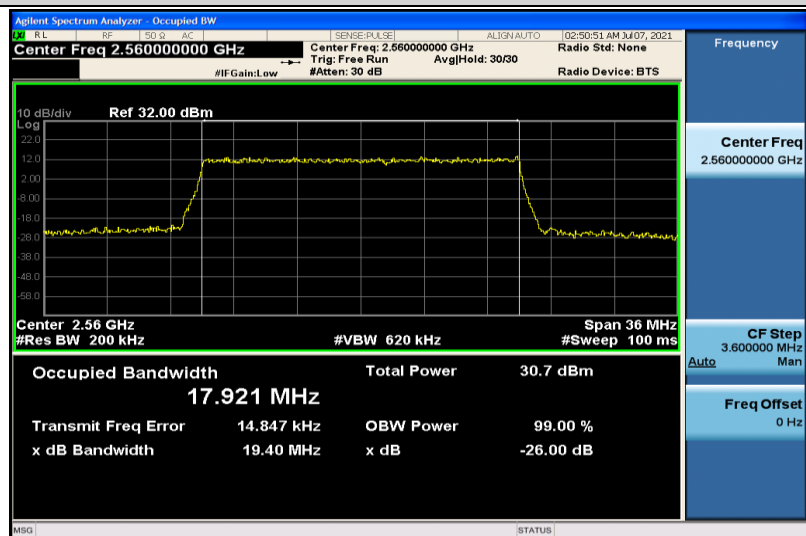
Band7-20MHz-16QAM-21350-100RB#0-17.921
