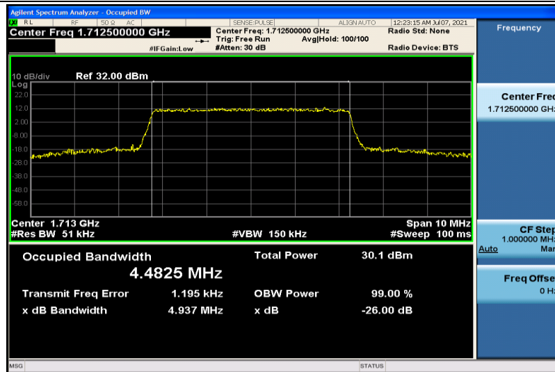
Band4-5MHz-16QAM-19975-25RB#0-4.4825
