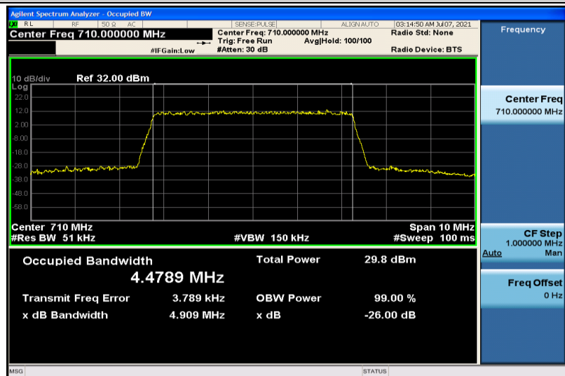
Band17-5MHz-16QAM-23790-25RB#0-4.4789
