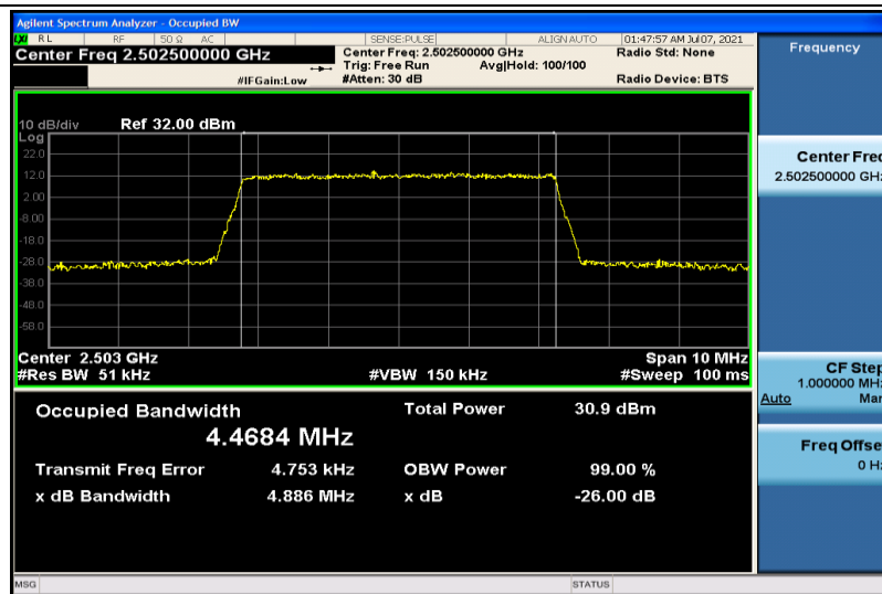
Band7-5MHz-QPSK-20775-25RB#0-4.4684
