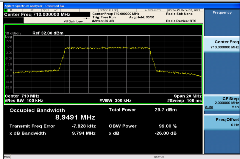
Band17-10MHz-16QAM-23790-50RB#0-8.9491
