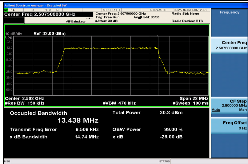
Band7-15MHz-QPSK-20825-75RB#0-13.438
