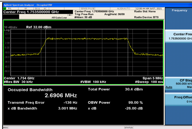
Band4-3MHz-QPSK-1753500000-15RB#0-2.6906
