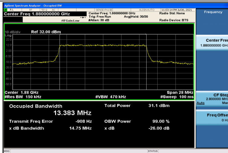
Band2-15MHz-QPSK-18900-75RB#0-13.383
