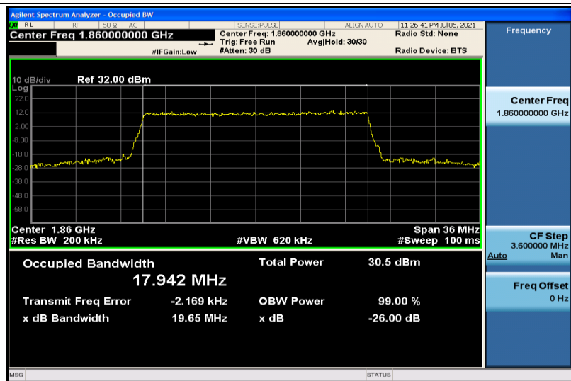
Band2-20MHz-16QAM-18700-100RB#0-17.942
