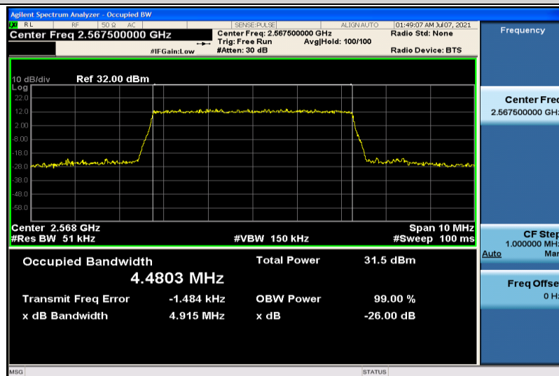
Band7-5MHz-QPSK-21425-25RB#0-4.4803
