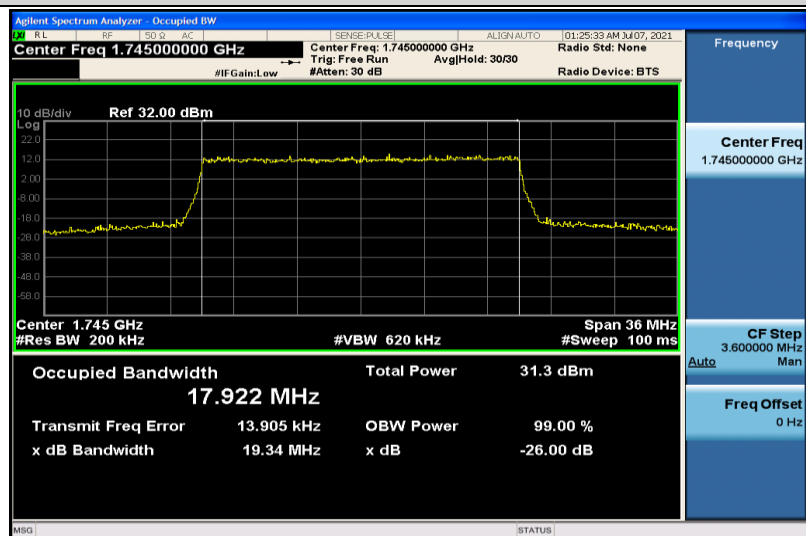
Band4-20MHz-QPSK-20300-100RB#0-17.922
