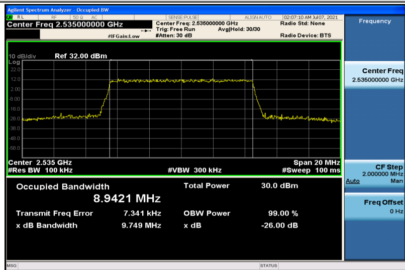
Band7-10MHz-16QAM-21100-50RB#0-8.9421
