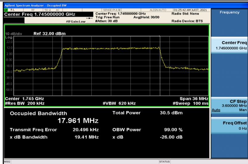
Band4-20MHz-16QAM-20300-100RB#0-17.961
