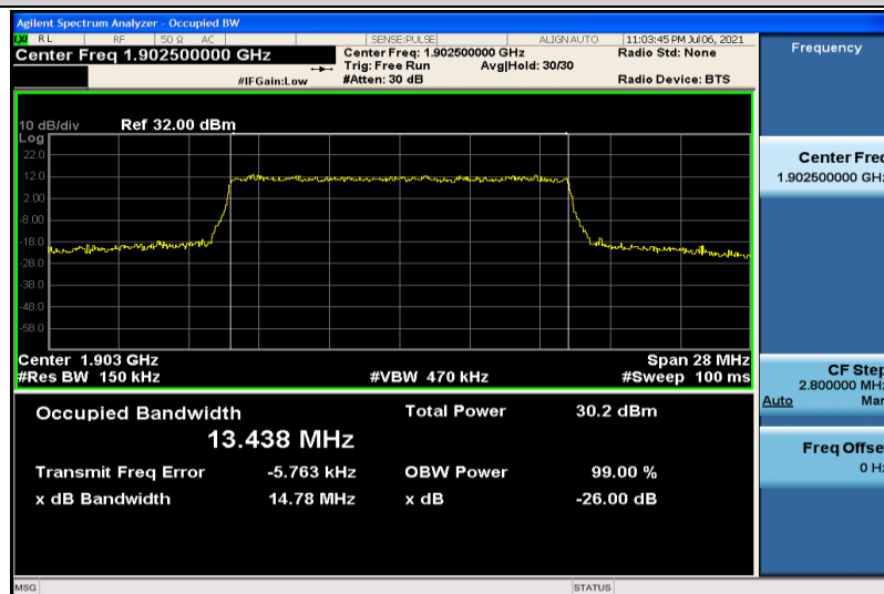
Band2-15MHz-16QAM-19125-75RB#0-13.438
