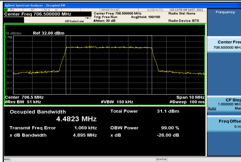
Band17-5MHz-QPSK-23755-25RB#0-4.4823
