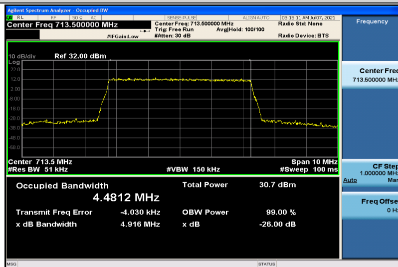
Band17-5MHz-QPSK-23825-25RB#0-4.4812
