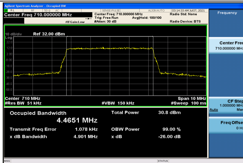
Band17-5MHz-QPSK-23790-25RB#0-4.4651
