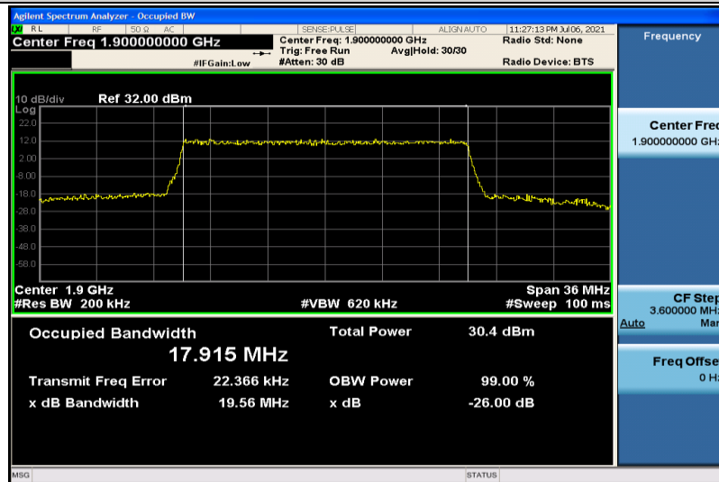
Band2-20MHz-QPSK-19100-100RB#0-17.915
