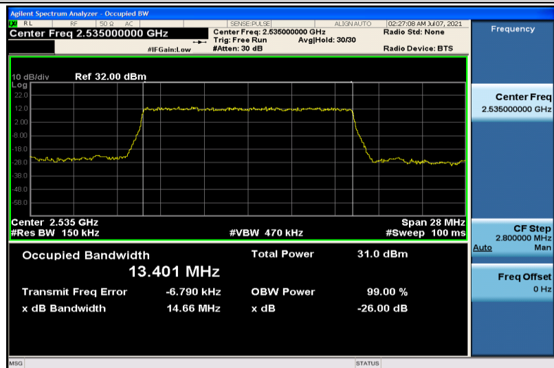
Band7-15MHz-QPSK-21100-75RB#0-13.401
