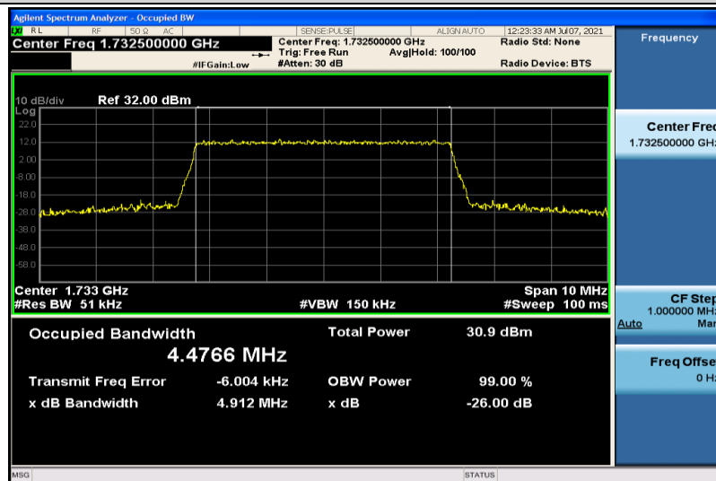
Band4-5MHz-QPSK-20175-25RB#0-4.4766
