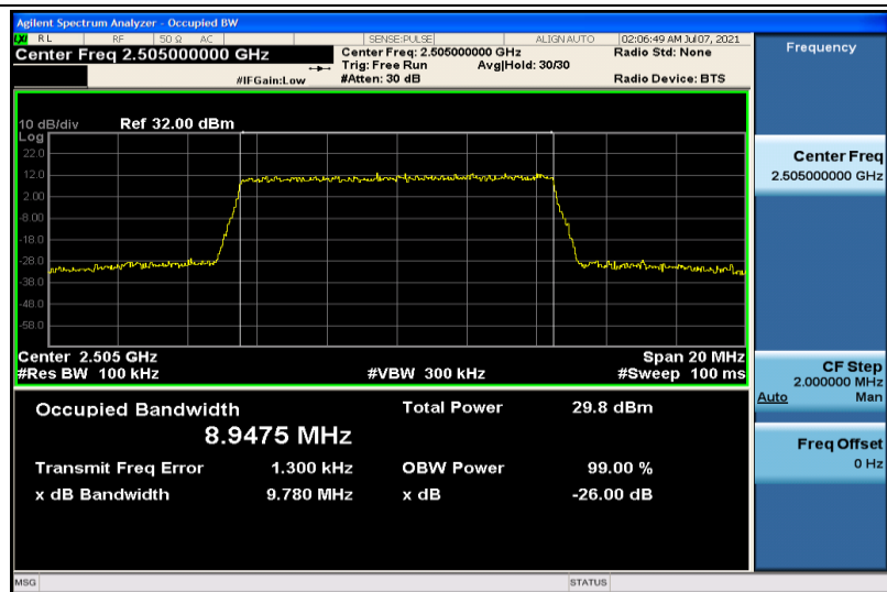
Band7-10MHz-16QAM-20800-50RB#0-8.9475
