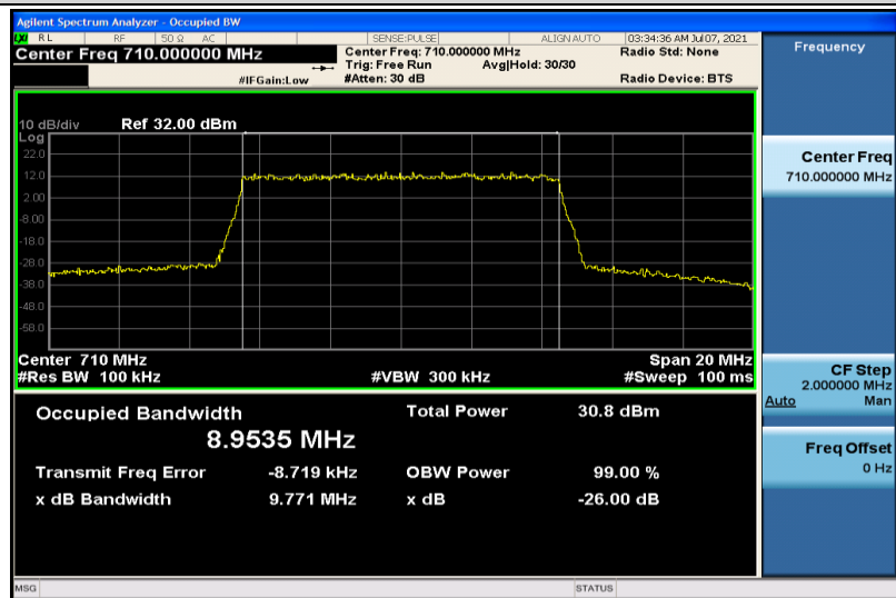
Band17-10MHz-QPSK-23790-50RB#0-8.9535
