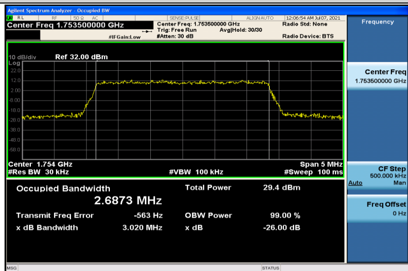
Band4-3MHz-16QAM-20385-15RB#0-2.6873
