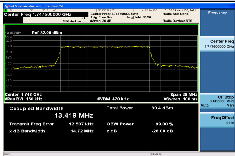
Band4-15MHz-16QAM-20325-75RB#0-13.419
