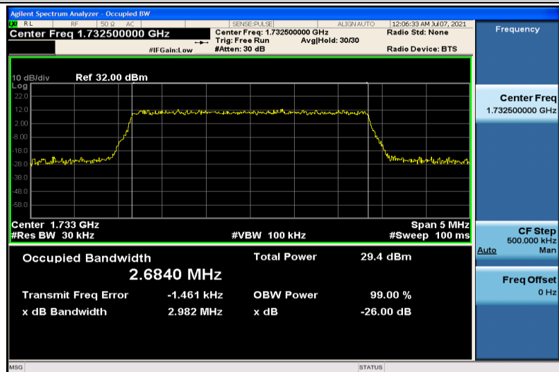
Band4-3MHz-16QAM-20175-15RB#0-2.6840
