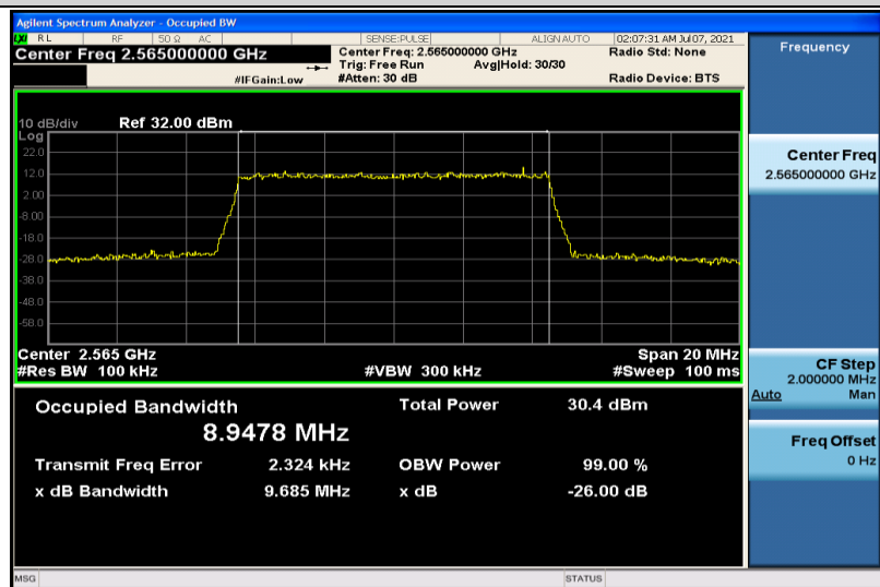
Band7-10MHz-16QAM-21400-50RB#0-8.9478
