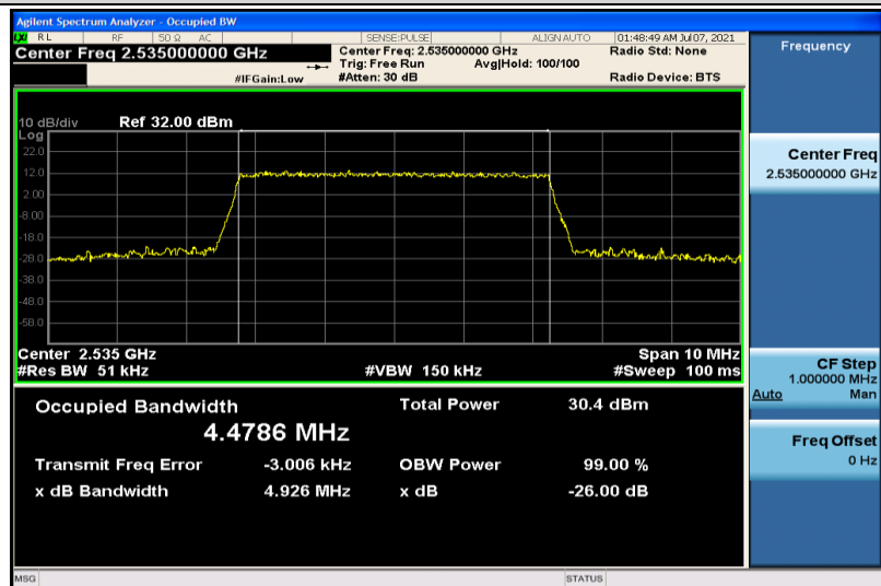
Band7-5MHz-16QAM-21100-25RB#0-4.4786
