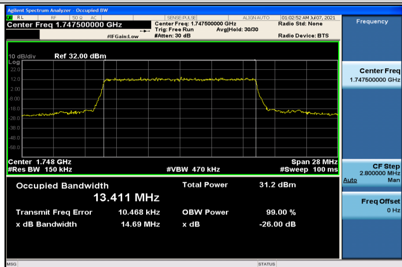
Band4-15MHz-QPSK-20325-75RB#0-13.411
