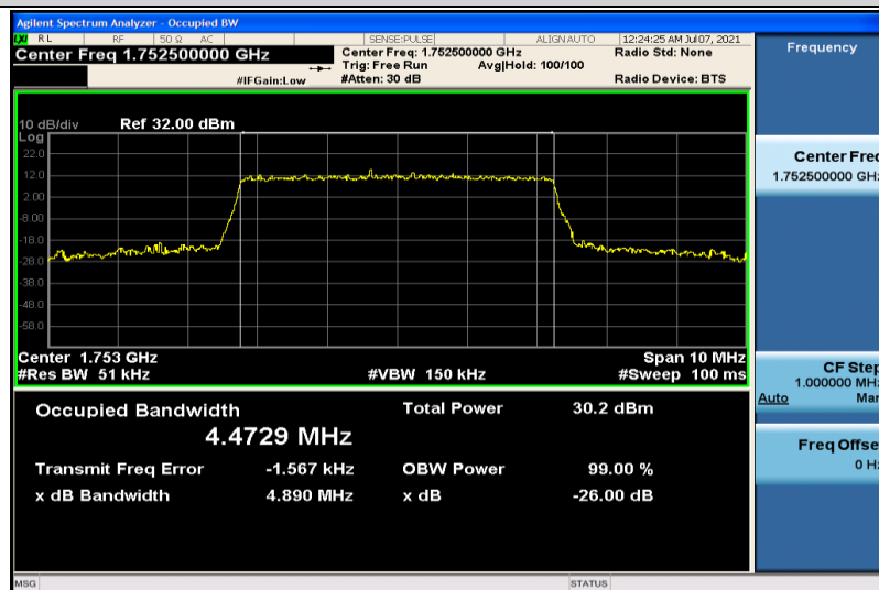
Band4-5MHz-16QAM-20375-25RB#0-4.4729
