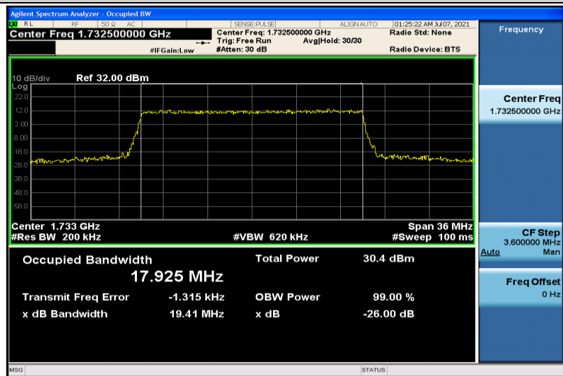
Band4-20MHz-16QAM-20175-100RB#0-17.925
