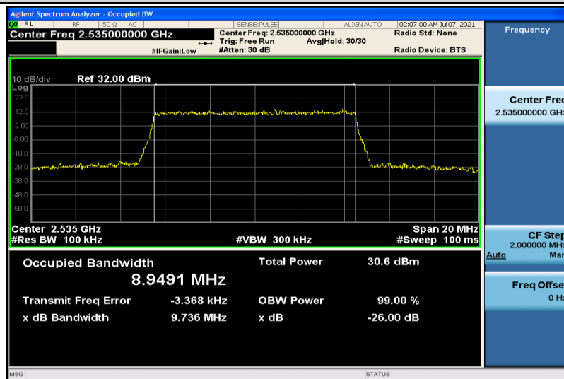
Band7-10MHz-QPSK-21100-50RB#0-8.9491
