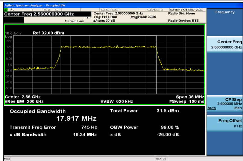
Band7-20MHz-QPSK-21350-100RB#0-17.917
