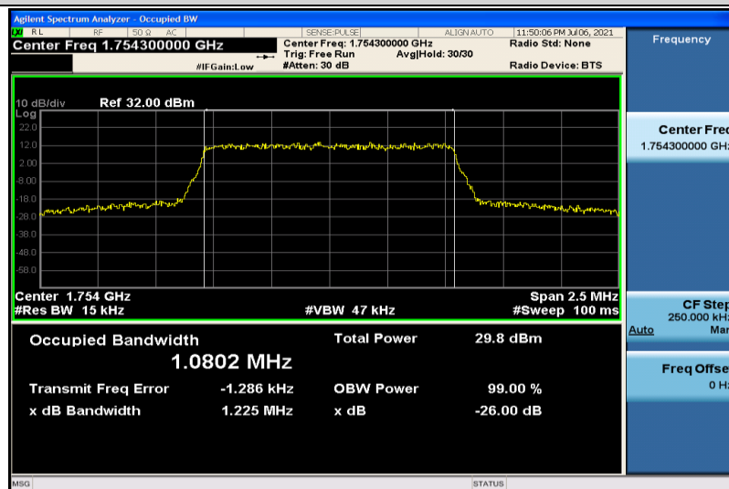
Band4-1.4MHz-QPSK-20393-6RB#0-1.0802
