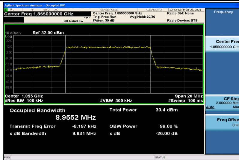
Band2-10MHz-16QAM-18650-50RB#0-8.9552
