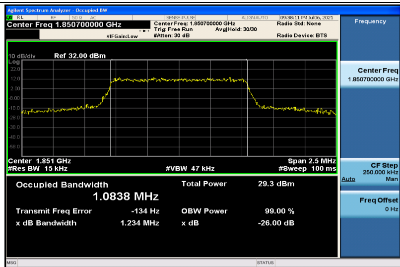
Band2-1.4MHz-16QAM-18607-6RB#0-1.0838
