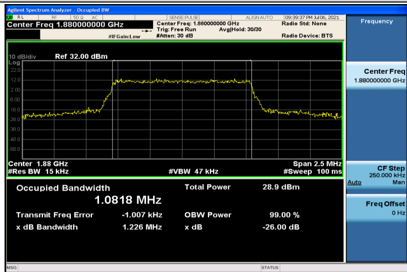
Band2-1.4MHz-16QAM-18900-6RB#0-1.0818
