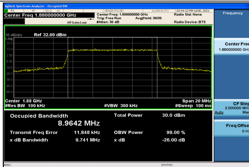
Band2-10MHz-16QAM-18900-50RB#0-8.9642
