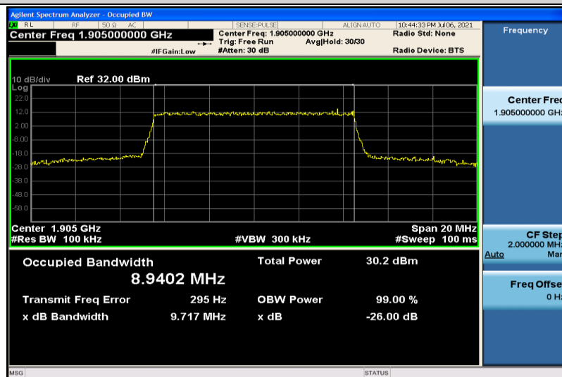
Band2-10MHz-16QAM-19150-50RB#0-8.9402
