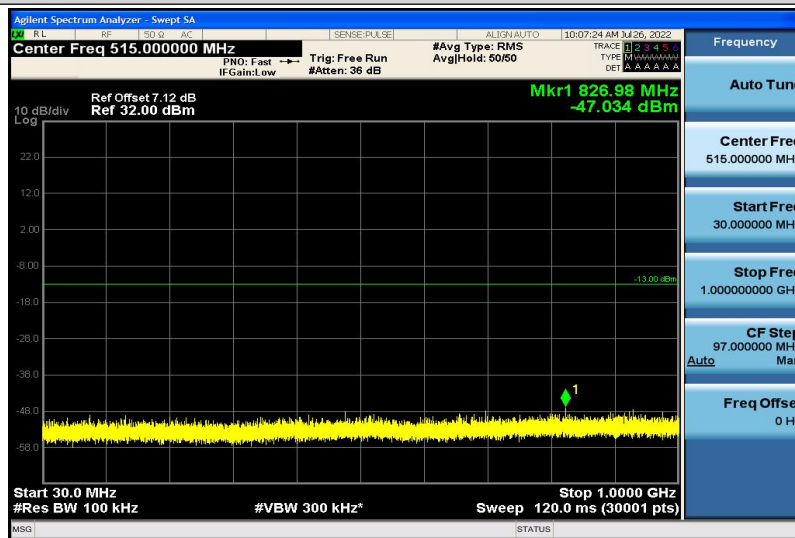
Band2-3MHz-16QAM-19185-1RB#0-30~1000MHz
