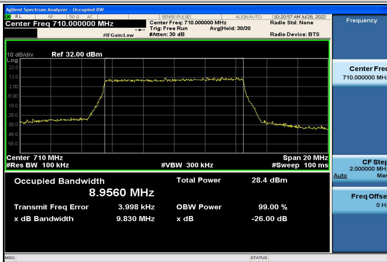
Band17-10MHz-16QAM-23790-50RB#0-8.9560
