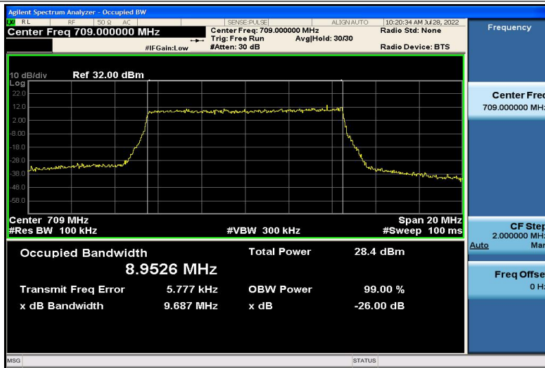
Band17-10MHz-16QAM-23780-50RB#0-8.9526
