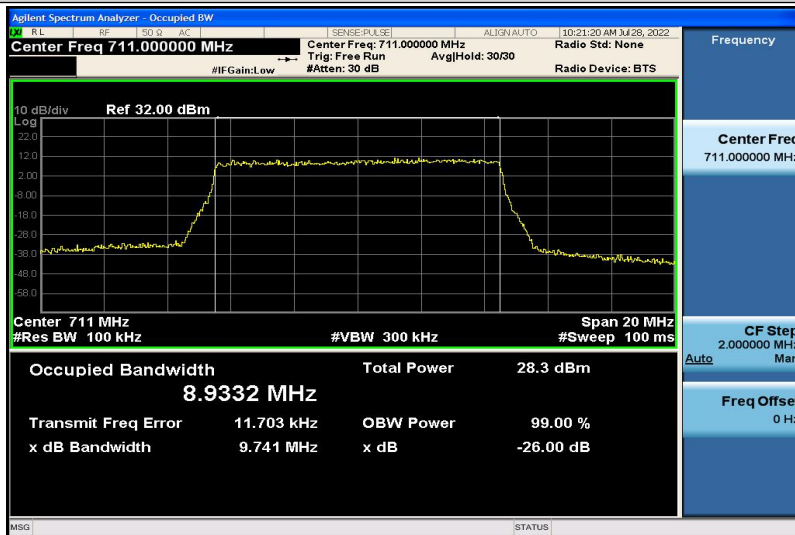
Band17-10MHz-16QAM-23800-50RB#0-8.9332
