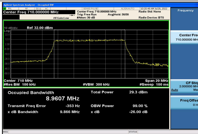
Band17-10MHz-QPSK-23790-50RB#0-8.9607
