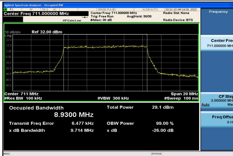
Band17-10MHz-QPSK-23800-50RB#0-8.9300
