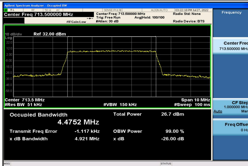
Band17-5MHz-QPSK-23825-25RB#0-4.4752
