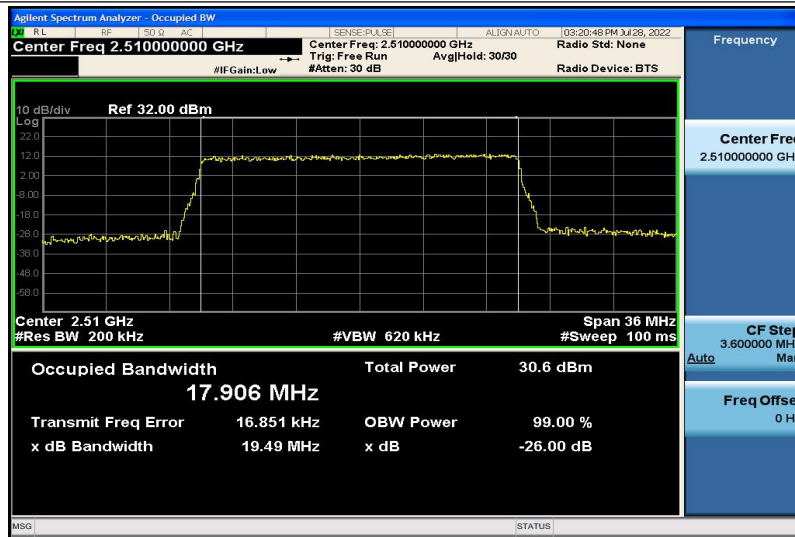
Band7-20MHz-QPSK-20850-100RB#0-17.906
