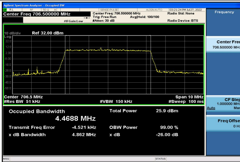
Band17-5MHz-16QAM-23755-25RB#0-4.4688
