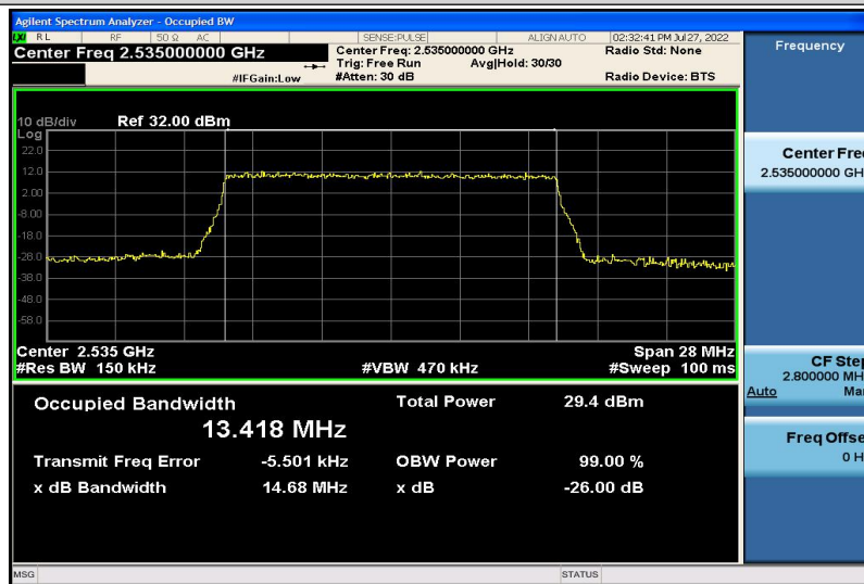
Band7-15MHz-QPSK-21100-75RB#0-13.418
