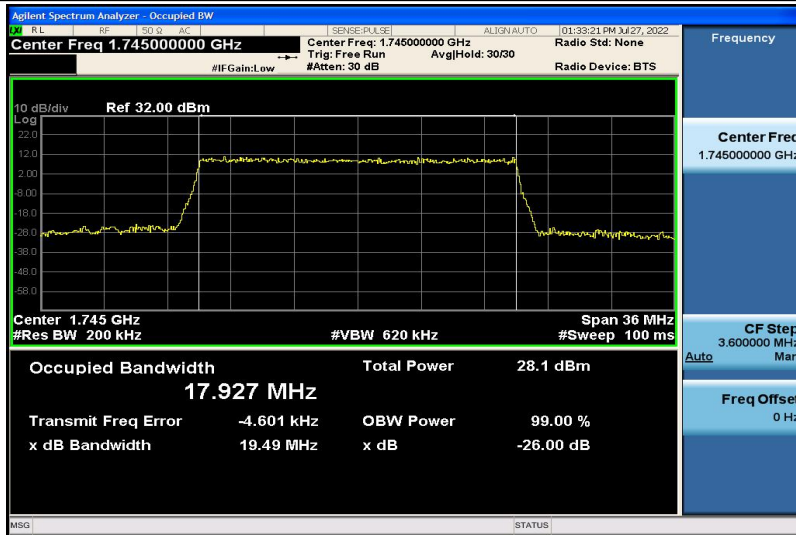
Band4-20MHz-16QAM-20300-100RB#0-17.927
