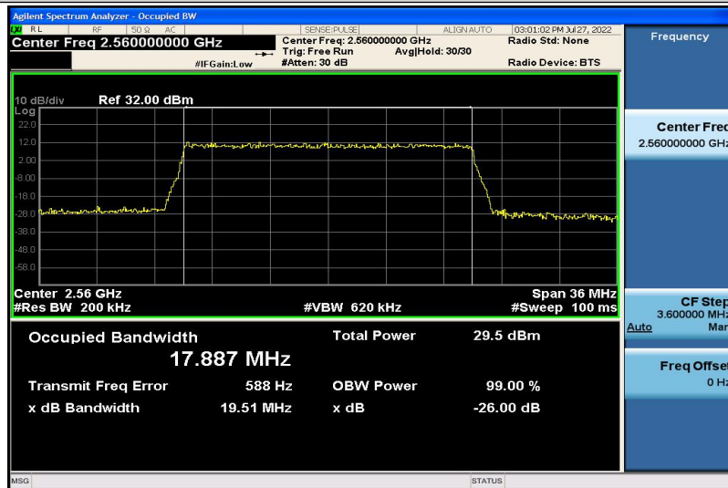
Band7-20MHz-16QAM-21350-100RB#0-17.887
