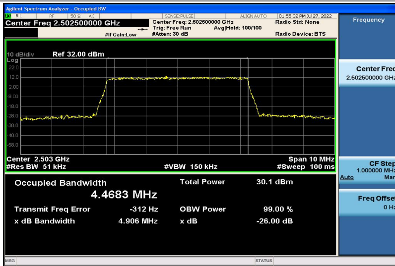
Band7-5MHz-QPSK-20775-25RB#0-4.4683
