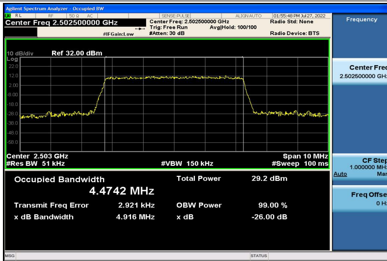
Band7-5MHz-16QAM-20775-25RB#0-4.4742
