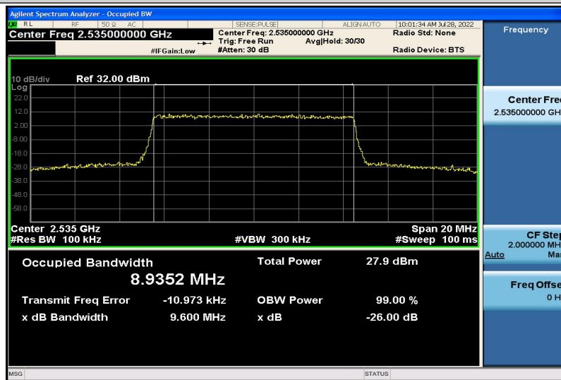
Band7-10MHz-16QAM-21100-50RB#0-8.9352
