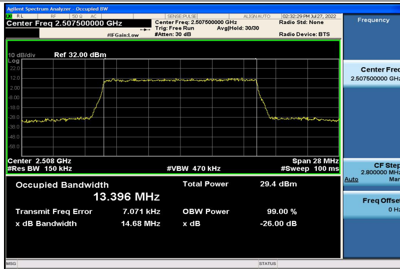
Band7-15MHz-16QAM-20825-75RB#0-13.396
