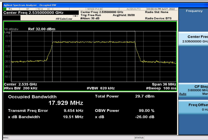
Band7-20MHz-16QAM-21100-100RB#0-17.929
