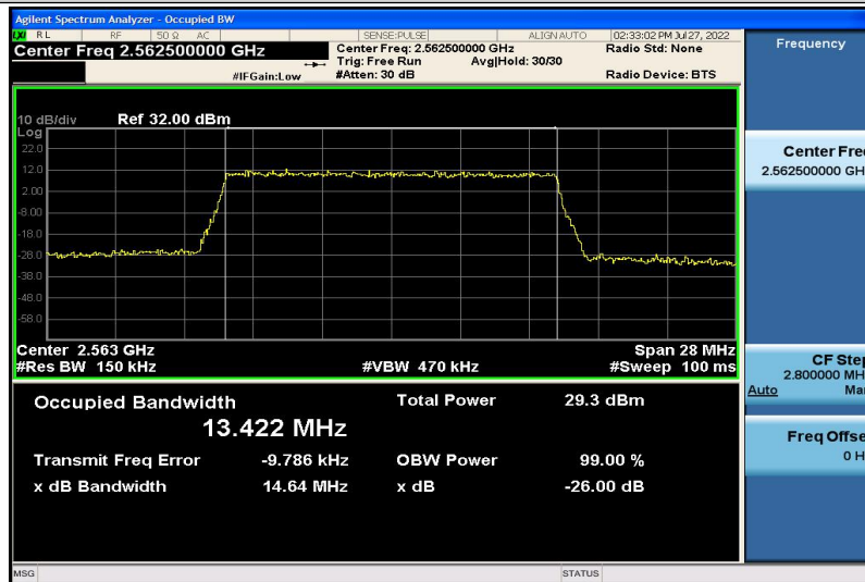
Band7-15MHz-QPSK-21375-75RB#0-13.422
