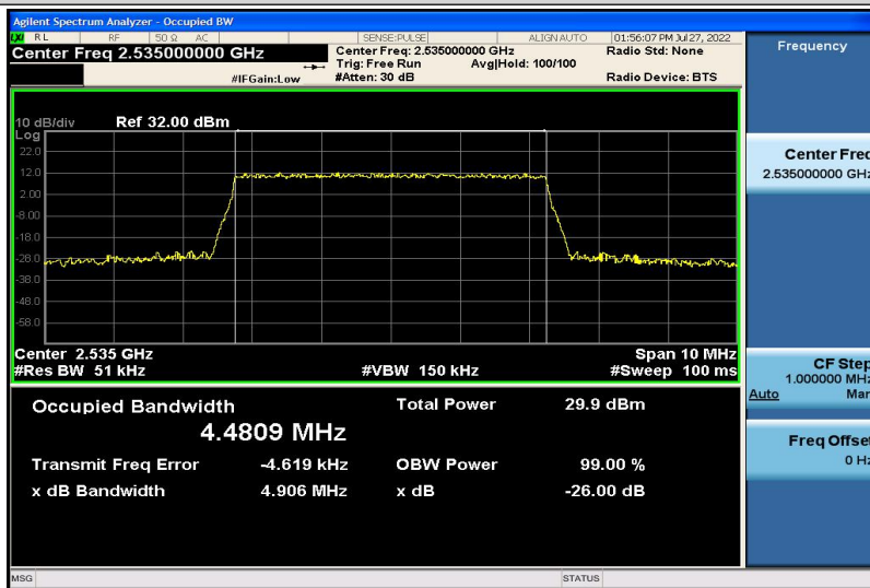
Band7-5MHz-QPSK-21100-25RB#0-4.4809
