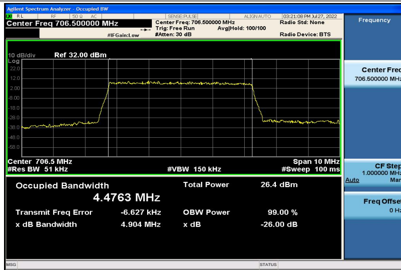
Band17-5MHz-QPSK-23755-25RB#0-4.4763
