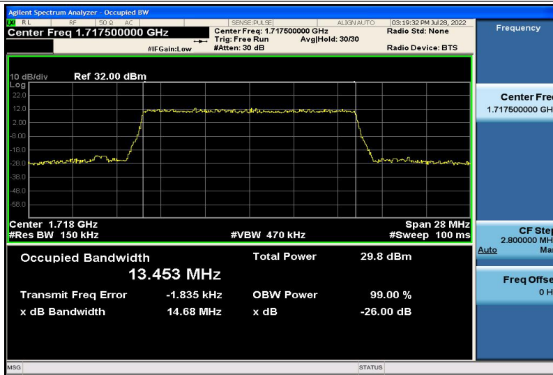
Band4-15MHz-QPSK-20025-75RB#0-13.453
