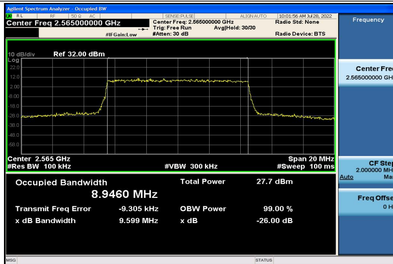
Band7-10MHz-16QAM-21400-50RB#0-8.9460
