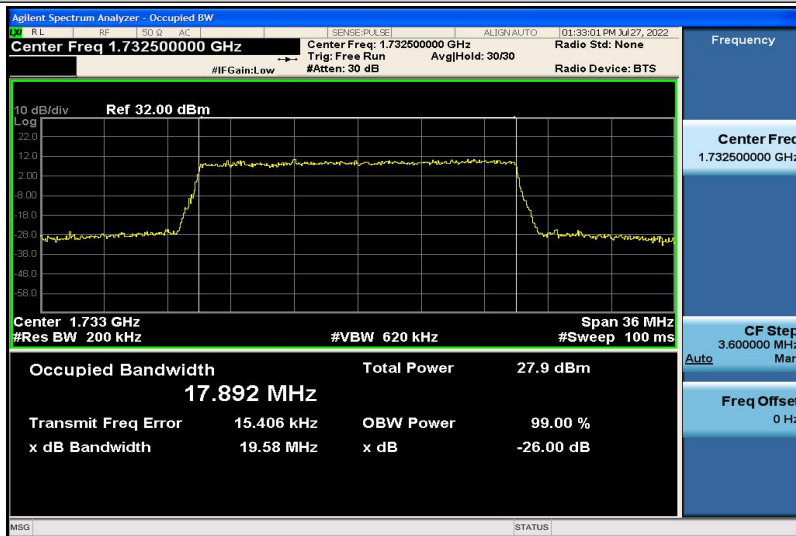
Band4-20MHz-16QAM-20175-100RB#0-17.892
