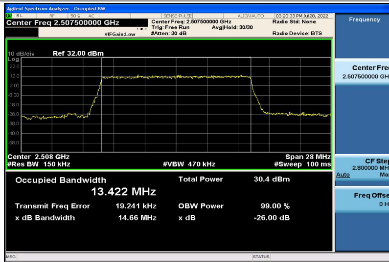
Band7-15MHz-QPSK-20825-75RB#0-13.422
