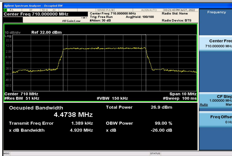
Band17-5MHz-QPSK-23790-25RB#0-4.4738
