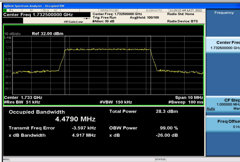
Band4-5MHz-QPSK-20175-25RB#0-4.4790
