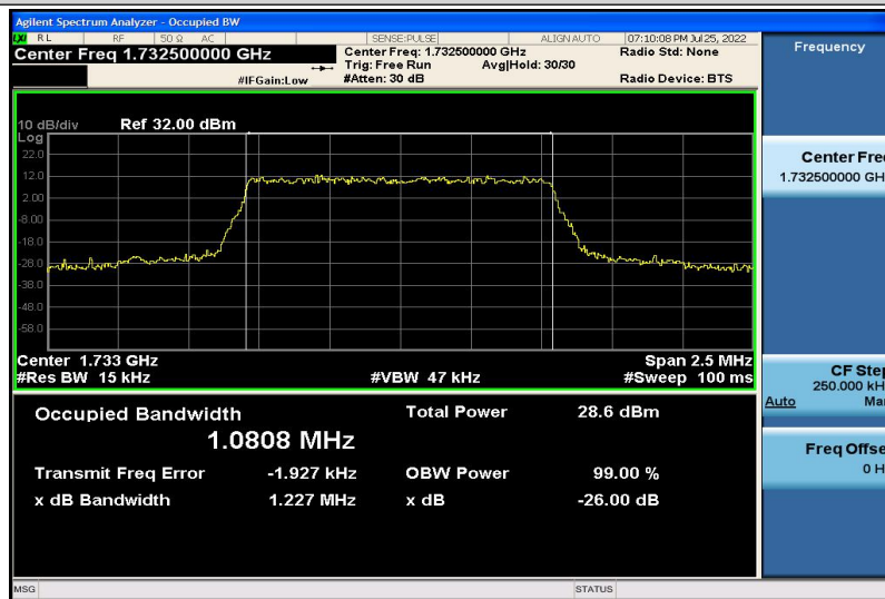
Band4-1.4MHz-QPSK-20175-6RB#0-1.0808
