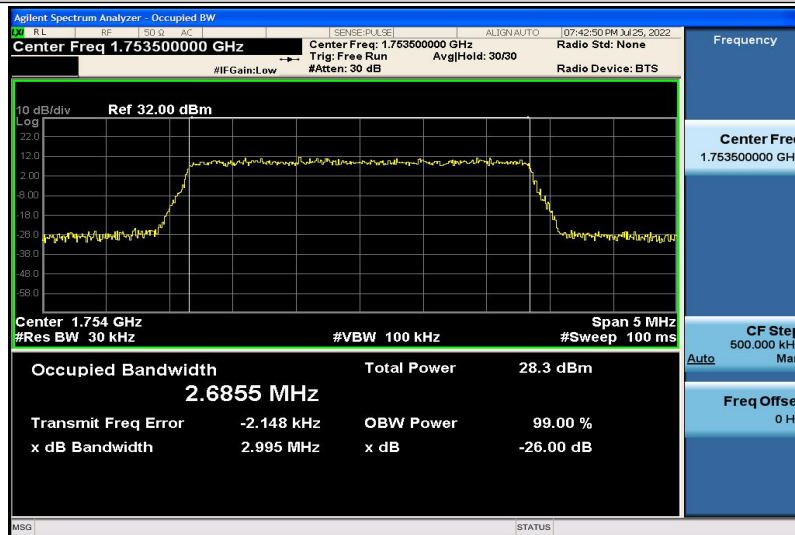
Band4-3MHz-QPSK-20385-15RB#0-2.6855
