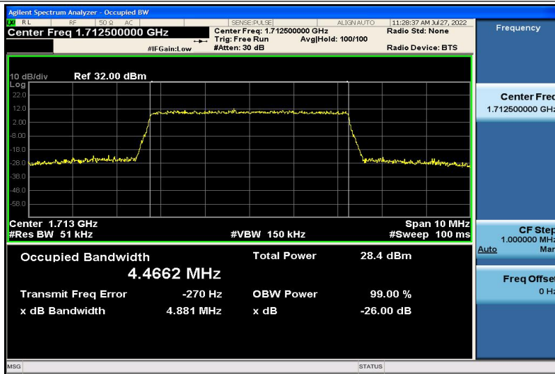
Band4-5MHz-QPSK-19975-25RB#0-4.4662
