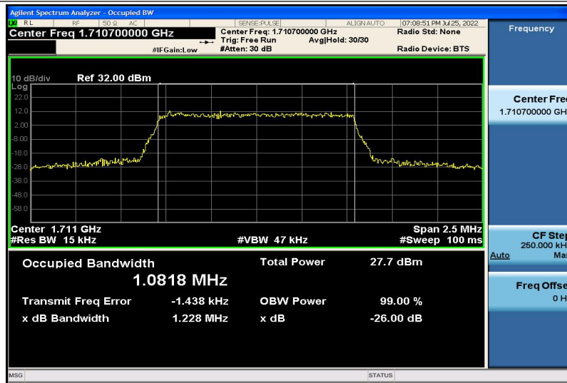
Band4-1.4MHz-16QAM-19957-6RB#0-1.0818
