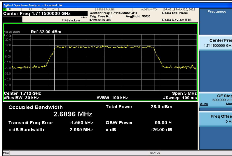
Band4-3MHz-16QAM-19965-15RB#0-2.6896
