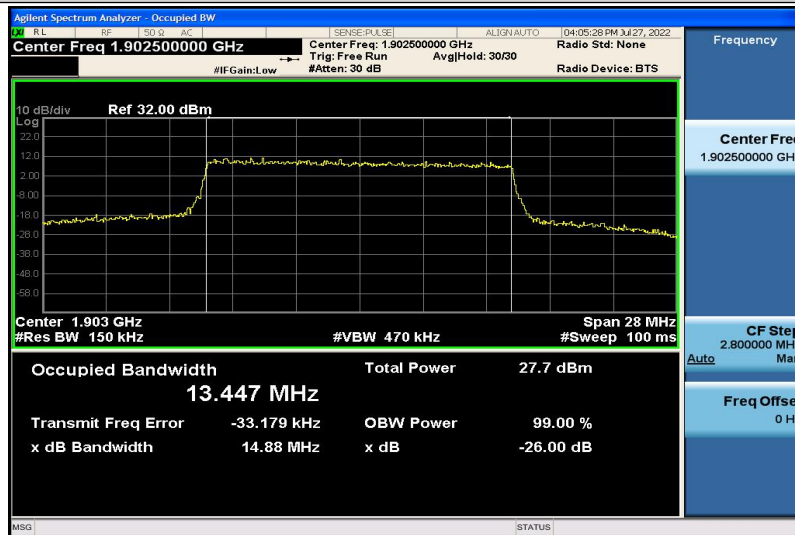
Band2-15MHz-QPSK-19125-75RB#0-13.447
