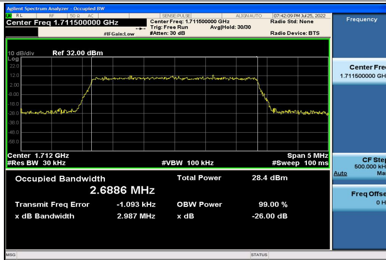
Band4-3MHz-QPSK-19965-15RB#0-2.6886
