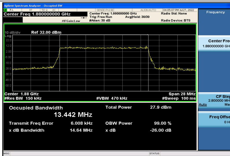
Band2-15MHz-QPSK-18900-75RB#0-13.442
