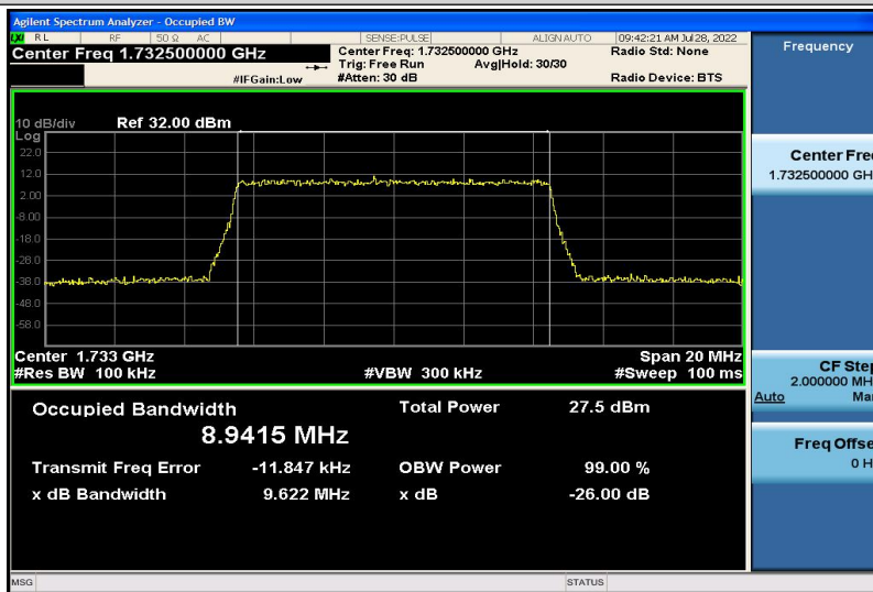
Band4-10MHz-16QAM-20175-50RB#0-8.9415
