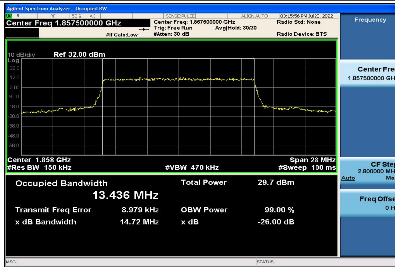
Band2-15MHz-QPSK-18675-75RB#0-13.436
