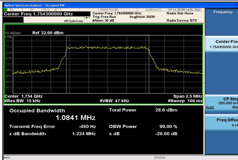
Band4-1.4MHz-QPSK-20393-6RB#0-1.0841
