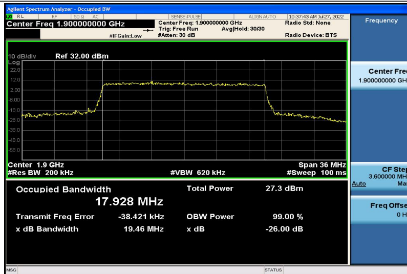
Band2-20MHz-16QAM-19100-100RB#0-17.928
