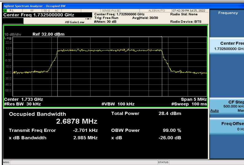
Band4-3MHz-16QAM-20175-15RB#0-2.6878
