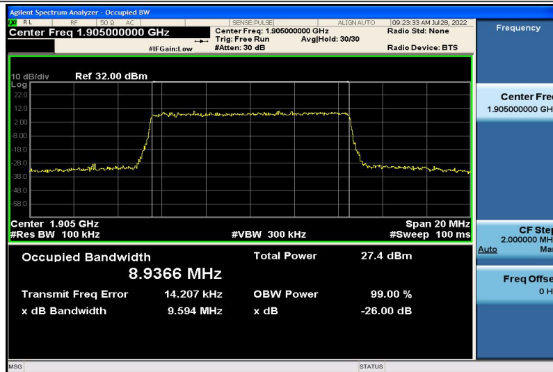
Band2-10MHz-16QAM-19150-50RB#0-8.9366
