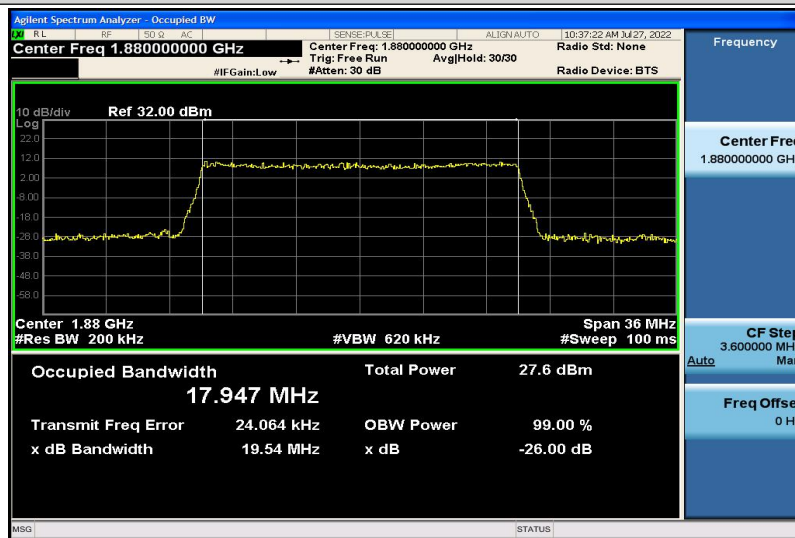
Band2-20MHz-16QAM-18900-100RB#0-17.947
