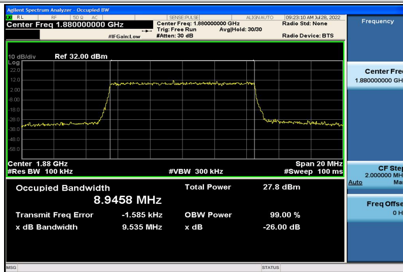
Band2-10MHz-16QAM-18900-50RB#0-8.9458
