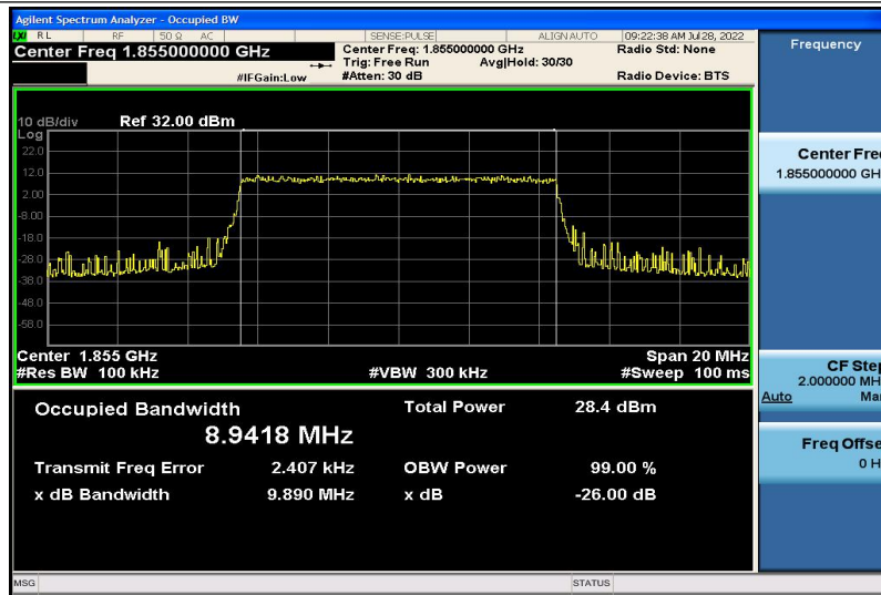
Band2-10MHz-QPSK-18650-50RB#0-8.9418
