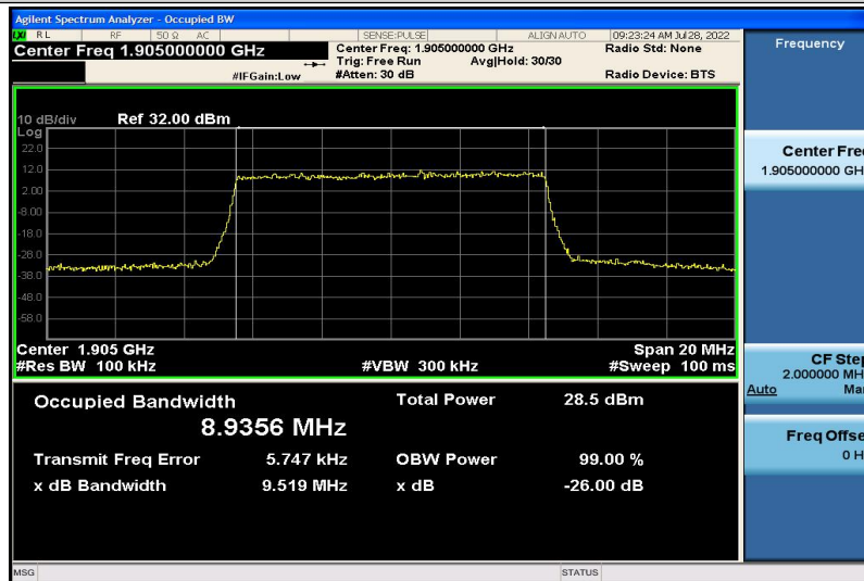
Band2-10MHz-QPSK-19150-50RB#0-8.9356
