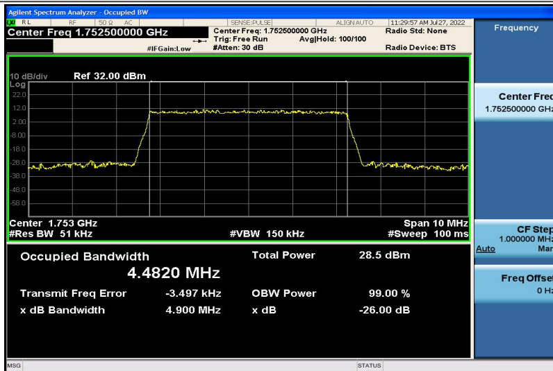
Band4-5MHz-QPSK-20375-25RB#0-4.4820
