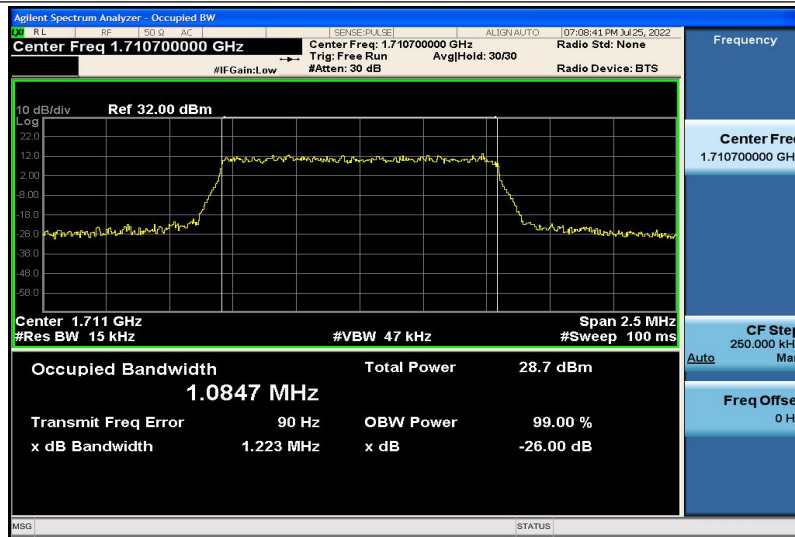
Band4-1.4MHz-QPSK-19957-6RB#0-1.0847
