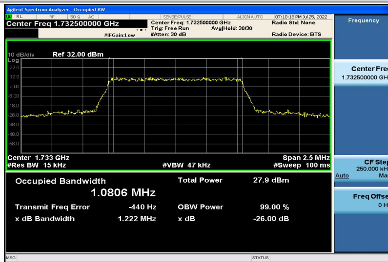
Band4-1.4MHz-16QAM-20175-6RB#0-1.0806
