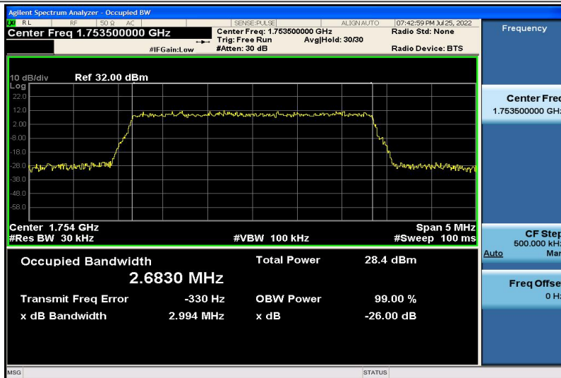
Band4-3MHz-16QAM-20385-15RB#0-2.6830
