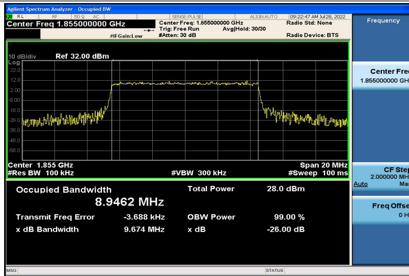
Band2-10MHz-16QAM-18650-50RB#0-8.9462
