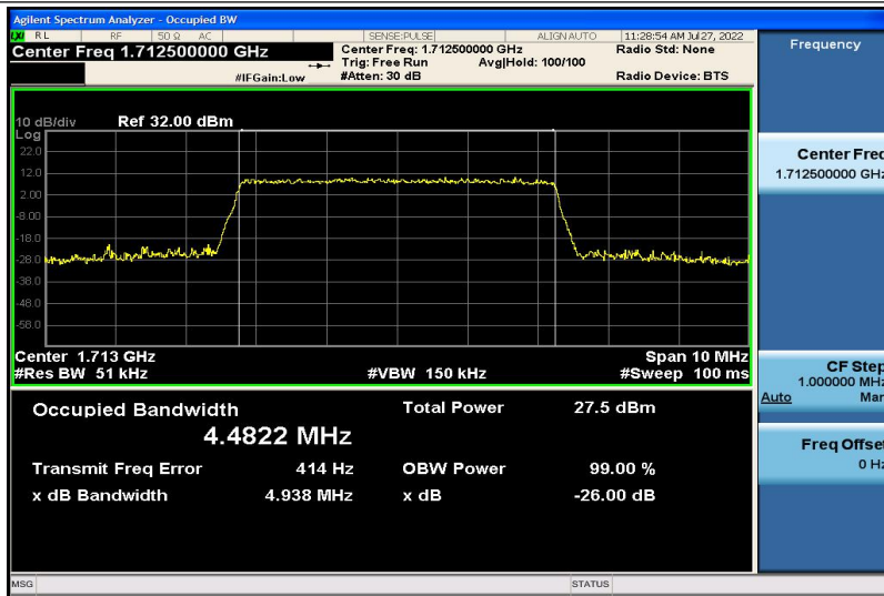
Band4-5MHz-16QAM-19975-25RB#0-4.4822
