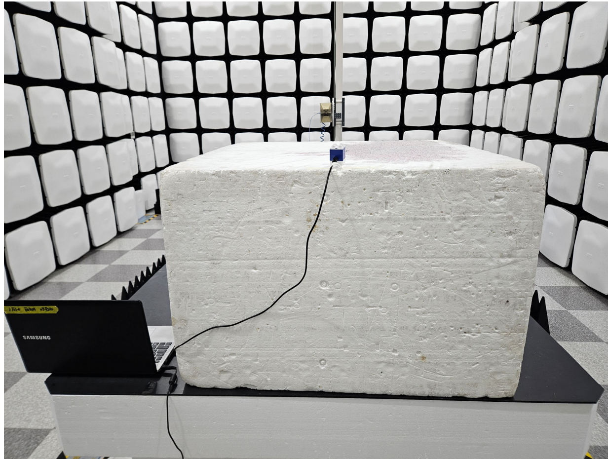
Radiated RF measurement (1 GHz ~ 40 GHz)
