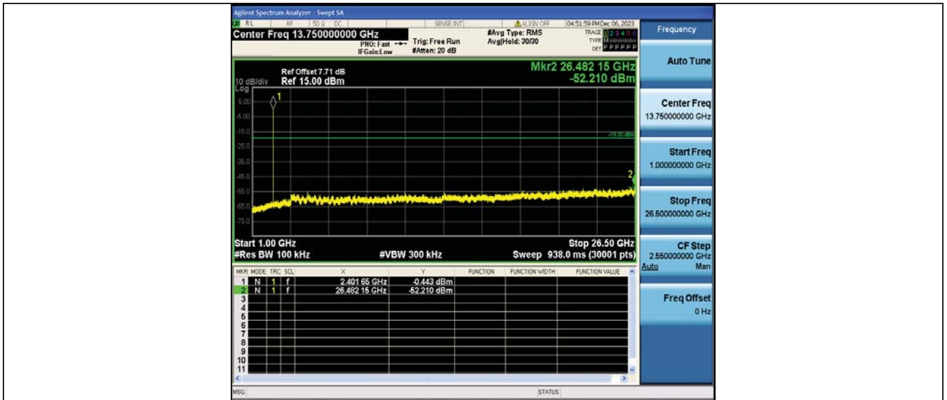
DH5_Ant2_2402_0~Reference
