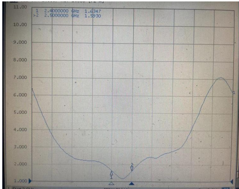
stationary wave pattern
