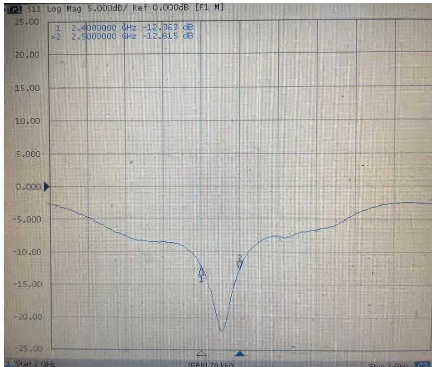
Return Loss
