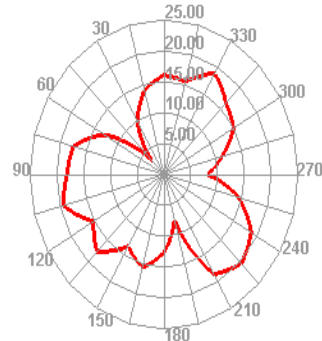
Wifi 11 TRP Phi=45
