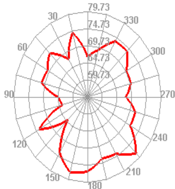
Wifi 36 TIS Phi=45
