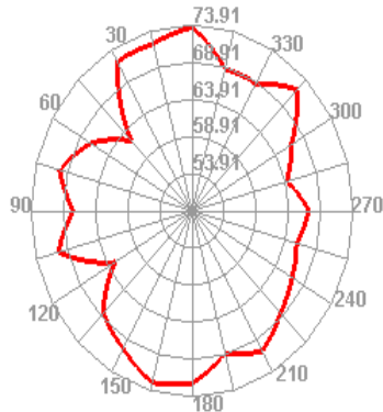
Wifi 64 TIS Phi=45
