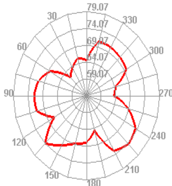
Wifi 6 TIS Phi=45
