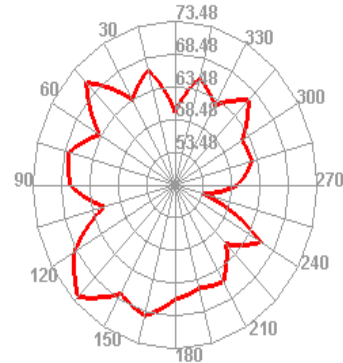
Wifi 165 TIS Phi=45
