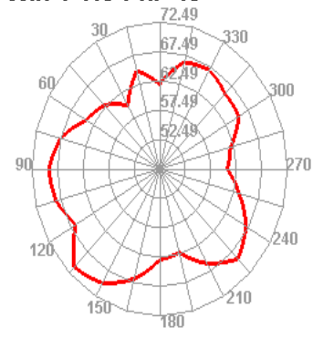
Wifi 1 TIS Phi=45
