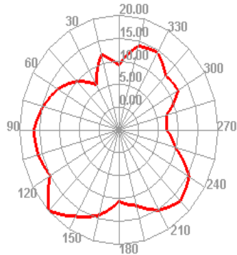
Wifi 1 TRP Phi=45
