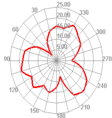
Wifi 1 TIS Phi=45
