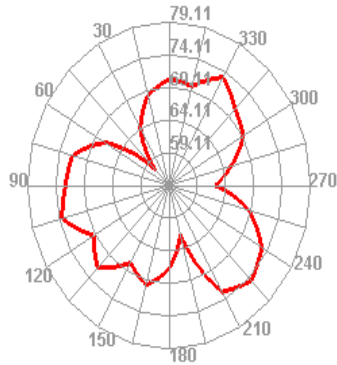
Wifi 11 TIS Phi=45
