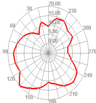
Wifi 1 TRP Phi=45
