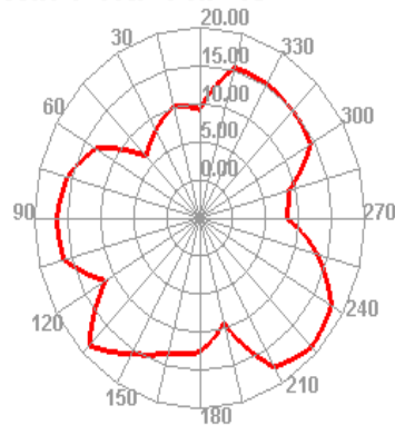
Wifi 6 TRP Phi=45
