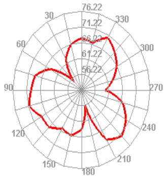
Wifi 11 TIS Phi=45
