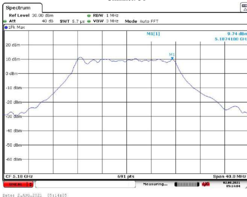
802.11a Channel: 36
