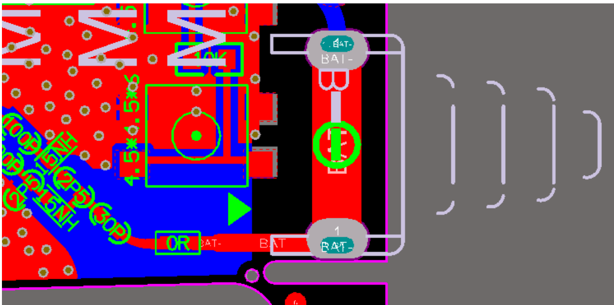
Antenna pictures
