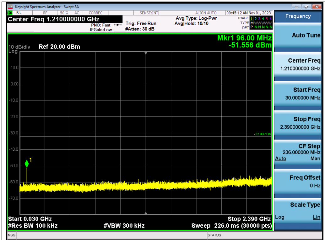
Test_Graph_π /4-DQPSK_ANT1_2402_Lower Band Emissions
