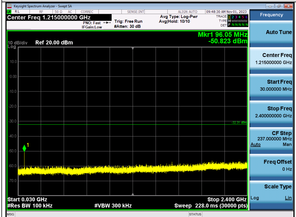
Test_Graph_π /4-DQPSK_ANT1_2441_Lower Band Emissions
