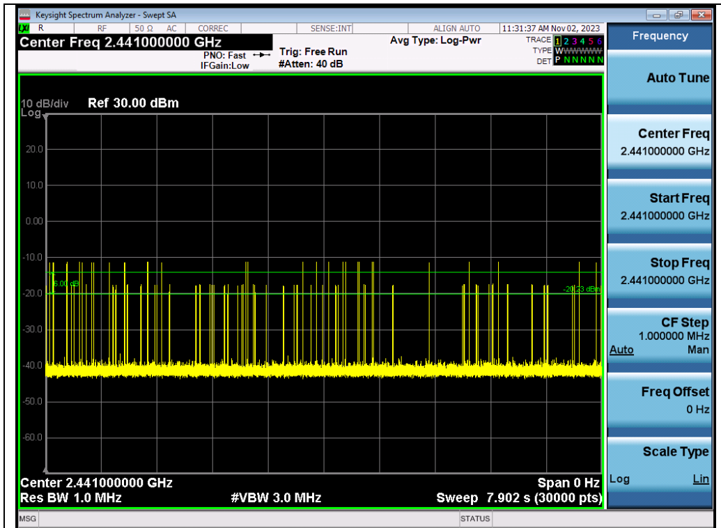
Test_Graph_π /4-DQPSK_HOP_ANT1_NA_1Mbps_2441_Number of Burst
