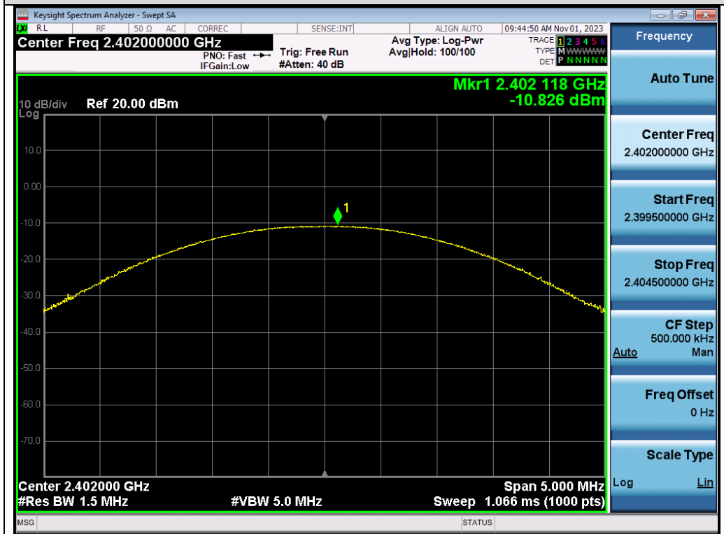
Test_Graph_π/4-DQPSK_ANT1_2402_Peak Power
