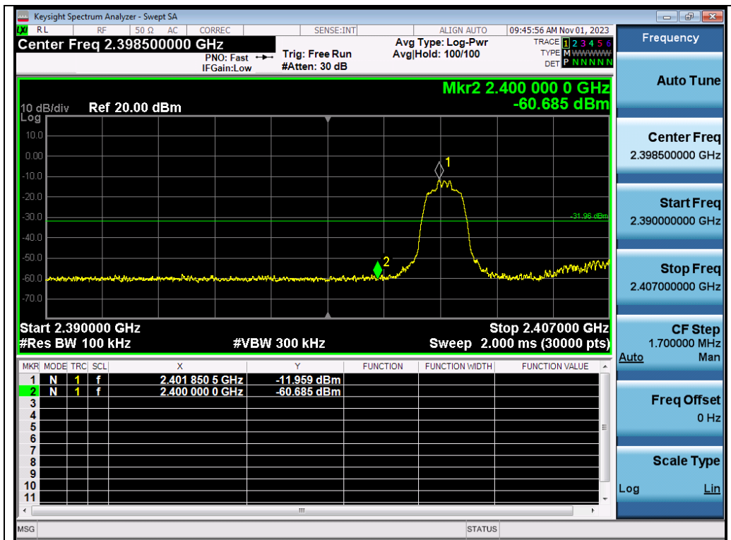
Test_Graph_pi /4-DQPSK_ANT1_2402_Lower Band Edge Emissions
