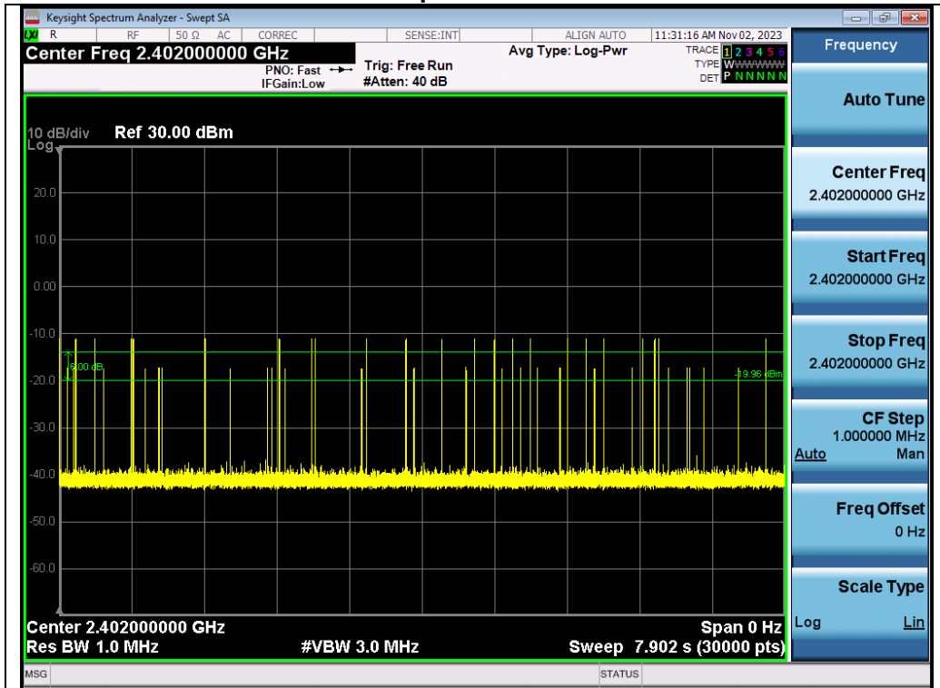
Test_Graph_π /4-DQPSK_HOP_ANT1_NA_1Mbps_2402_Number of Burst
