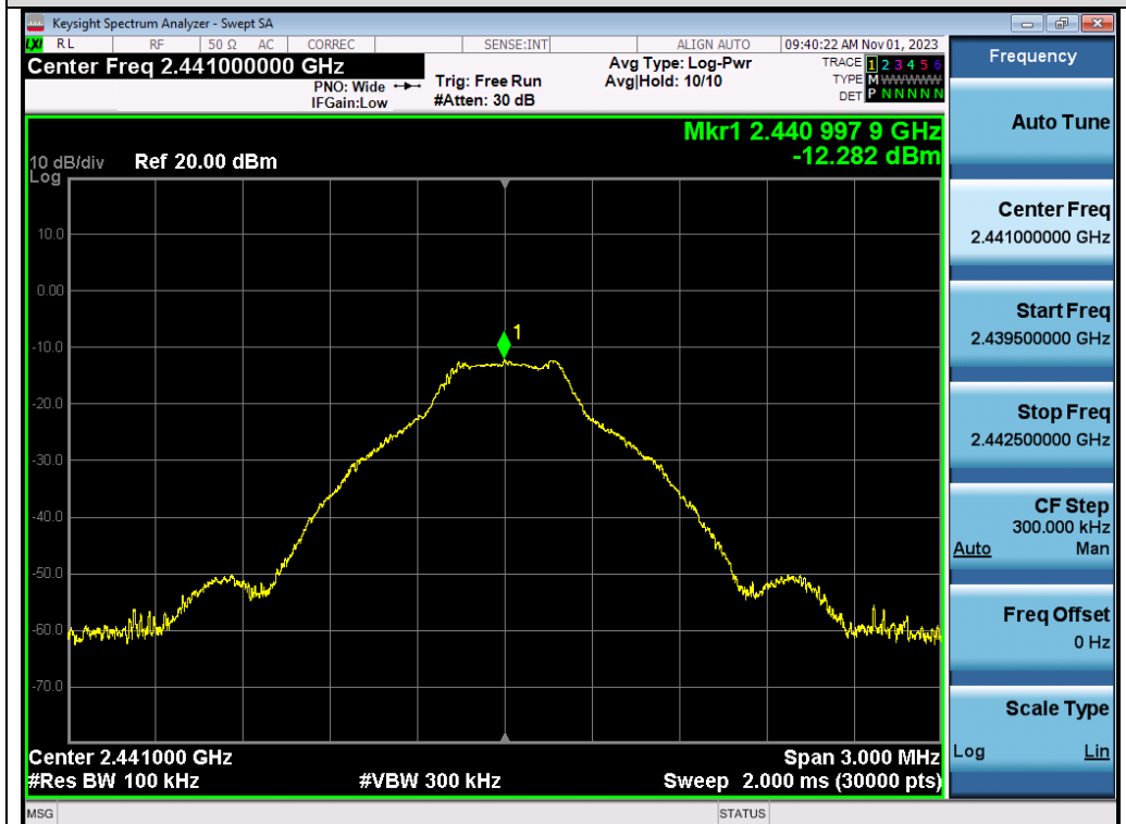
Test_Graph_GFSK_ANT1_2441_Reference Level
