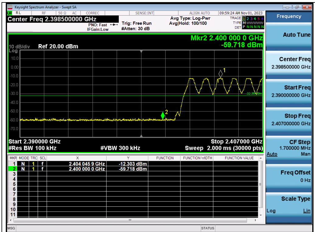
Test_Graph_GFSK_HOP_ANT1_NA_Lower Band Edge Emissions
