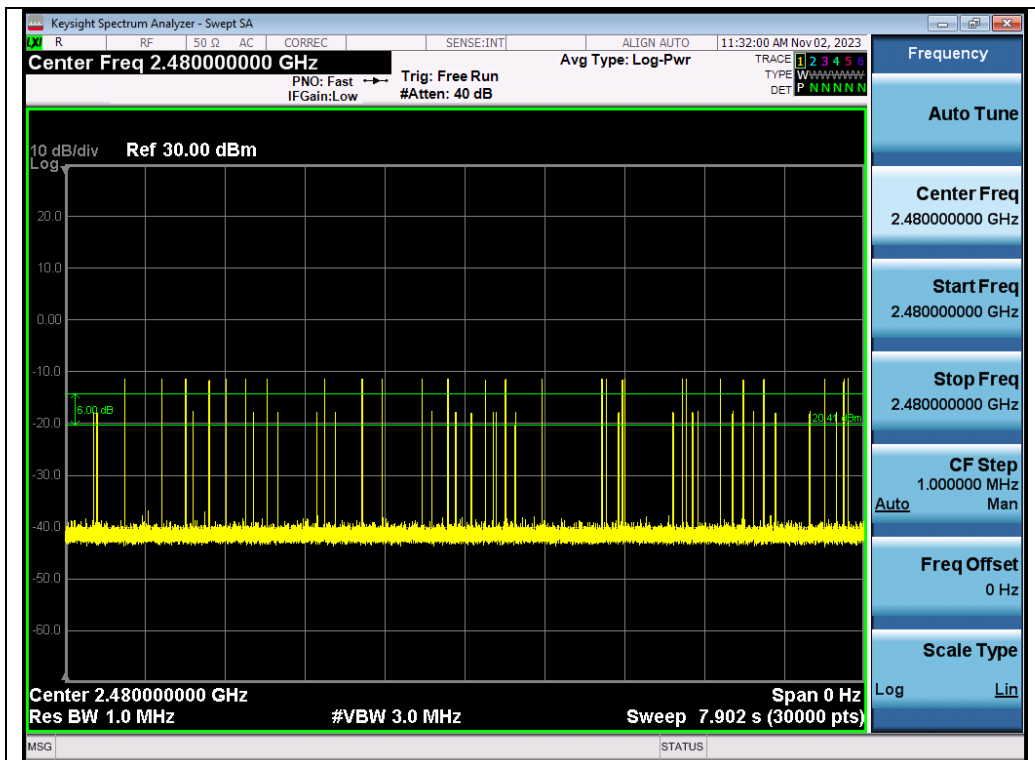
Test_Graph_π /4-DQPSK_HOP_ANT1_NA_1Mbps_2480_Number of Burst
