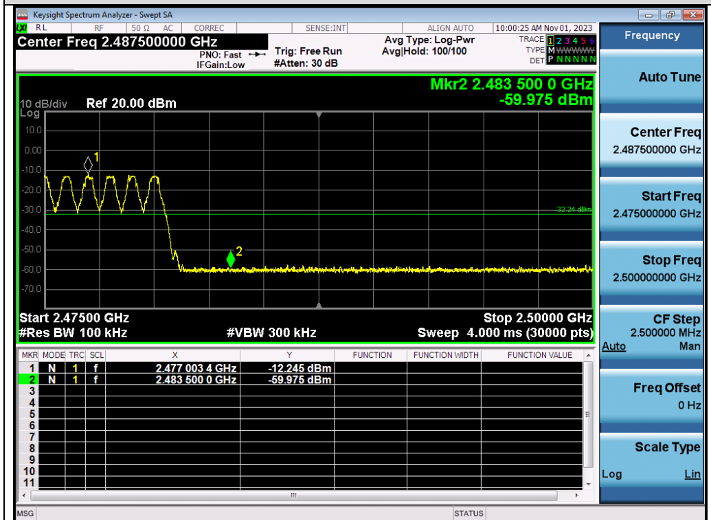
Test_Graph_GFSK_HOP_ANT1_NA_Higher Band Edge Emissions
