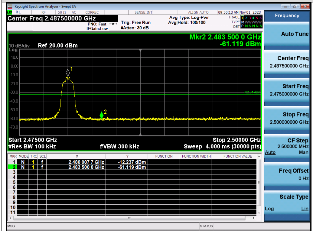
Test_Graph_pi /4-DQPSK_ANT1_2480_Higher Band Edge Emissions
