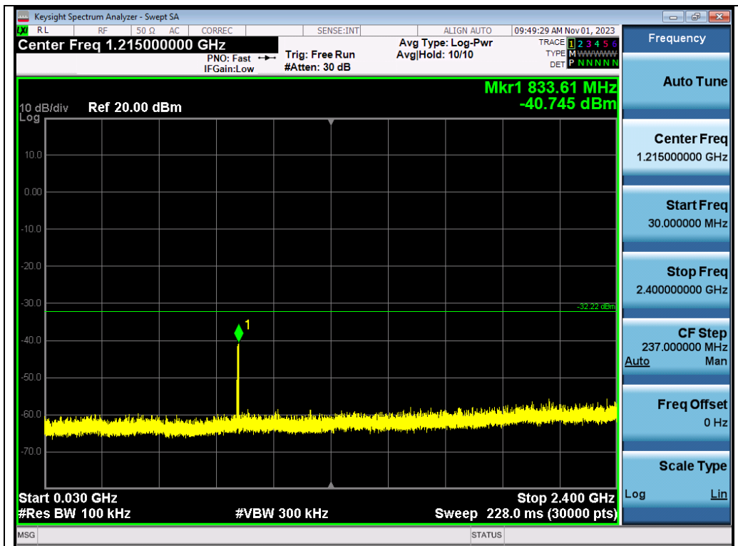
Test_Graph_π /4-DQPSK_ANT1_2480_Lower Band Emissions
