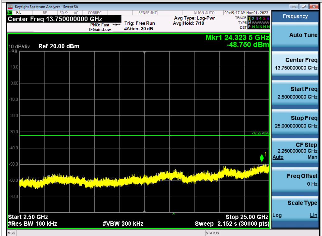
Test_Graph_π /4-DQPSK_ANT1_2480_Higher Band Emissions
