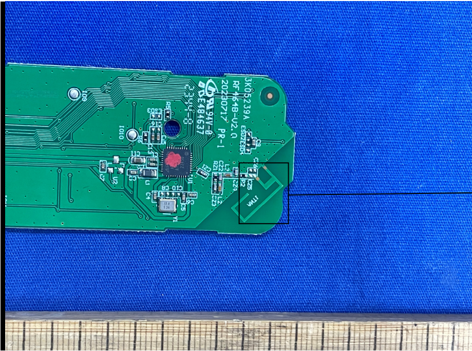
PCB Antenna
