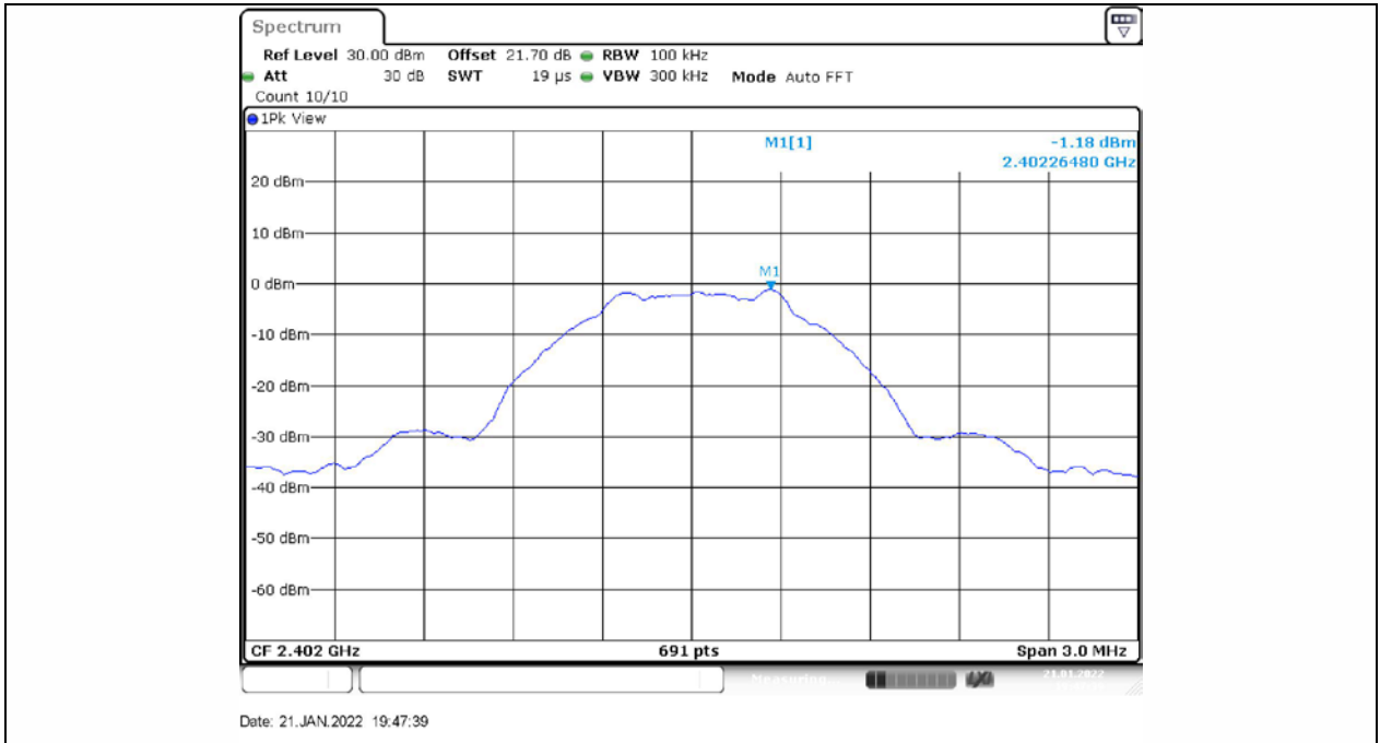
BLE_1M_Ant1_2402_0~Reference
