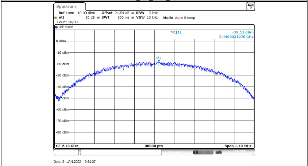
BLE_1M_Ant1_2440
