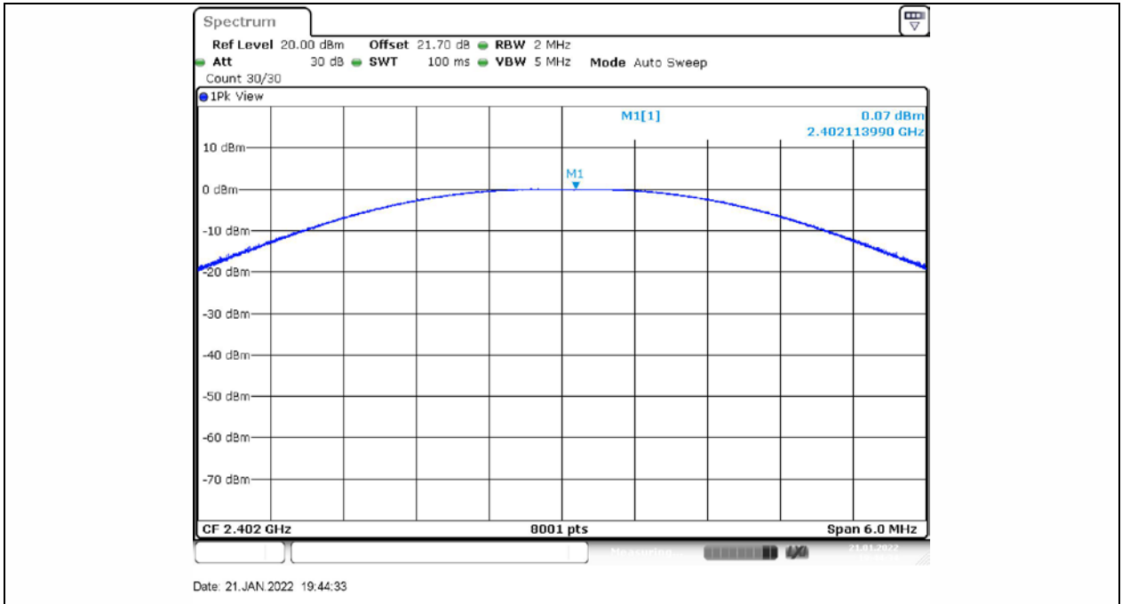
BLE_1M_Ant1_2402
