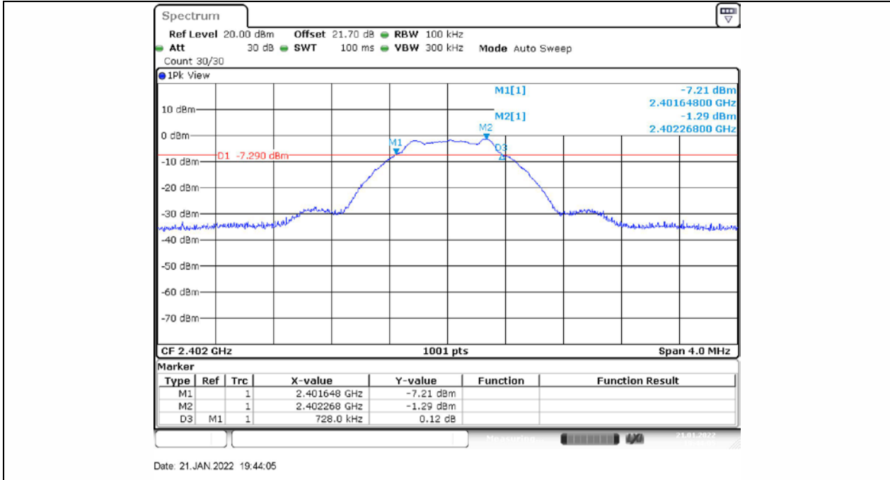
BLE_1M_Ant1_2402
