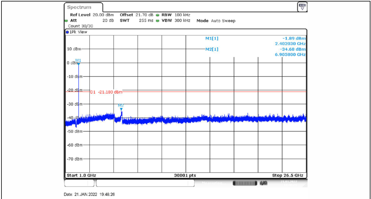
BLE_1M_Ant1_2402_1000~26500
