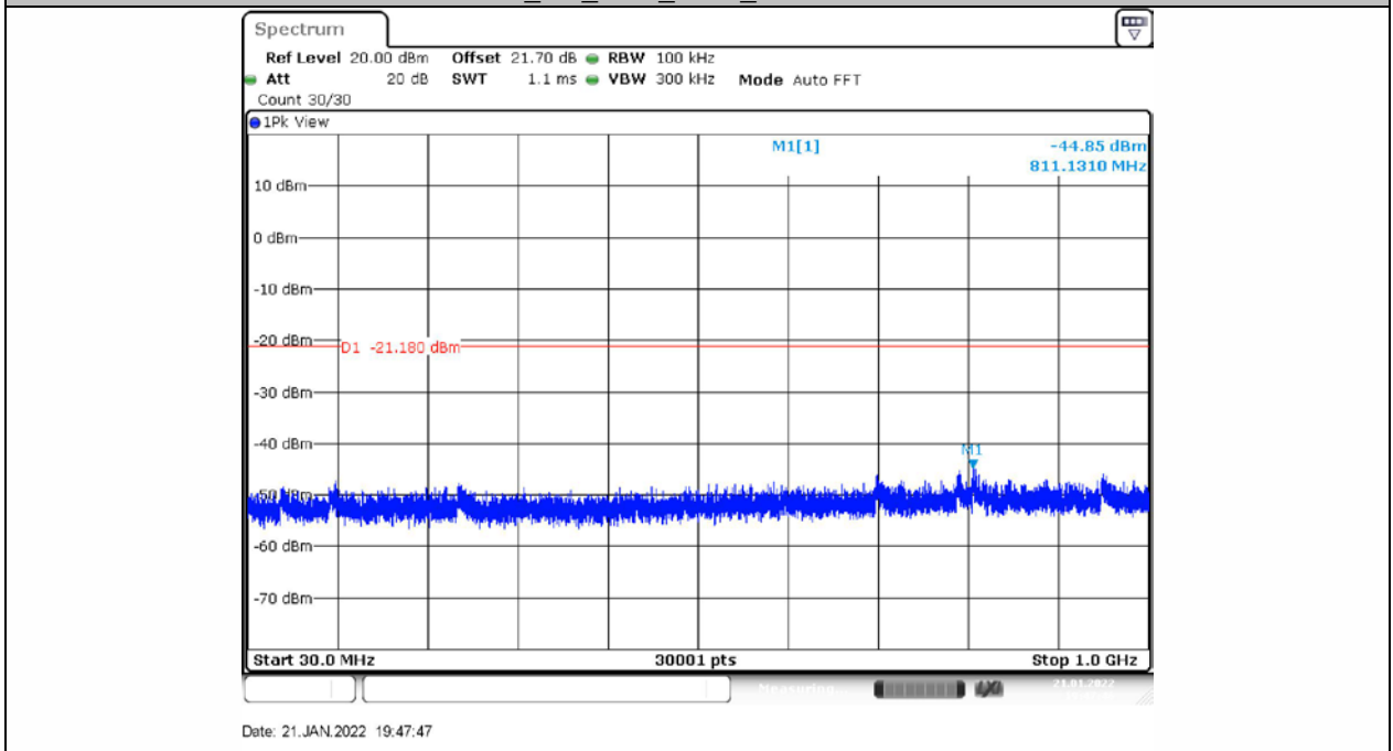
BLE_1M_Ant1_2402_30~1000
