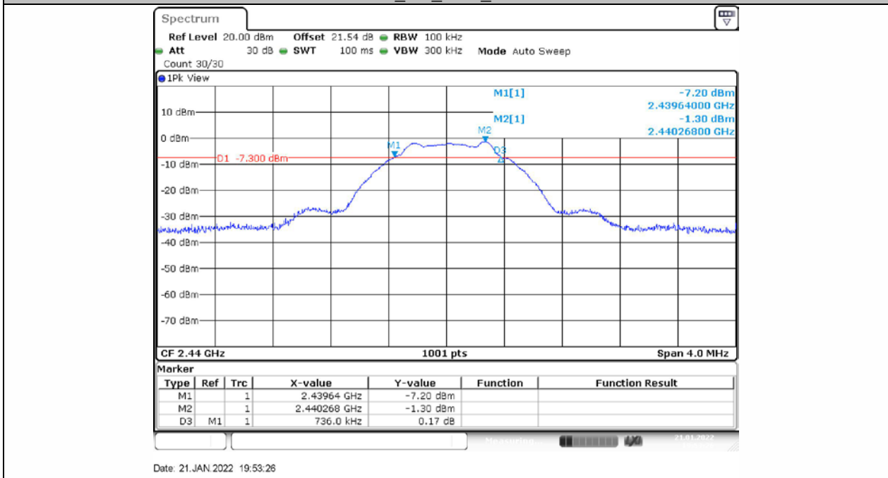
BLE_1M_Ant1_2440
