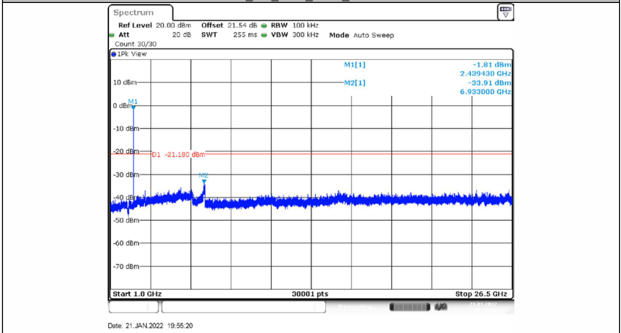
BLE_1M_Ant1_2440_1000~26500
