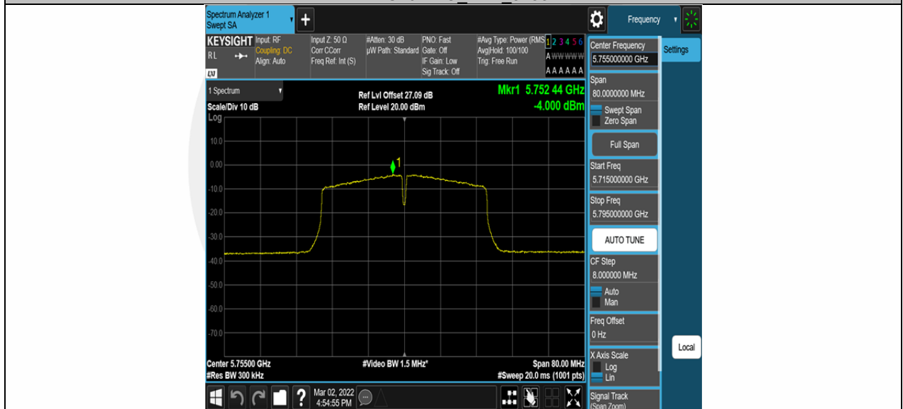
11AC40SISO_Ant1_5755
