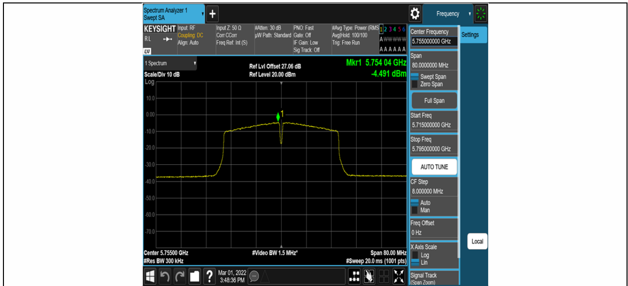
11AC40SISO_Ant2_5755
