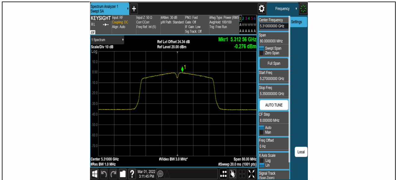
11AC40SISO_Ant2_5310
