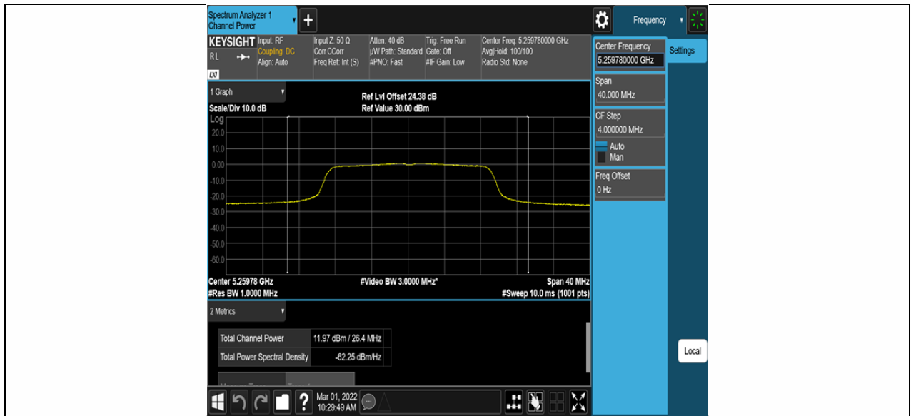
11N20SISO_Ant2_5260
