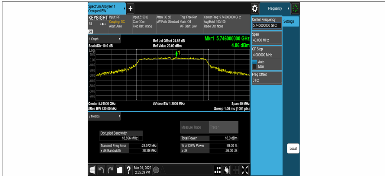
11AC20SISO_Ant2_5745
