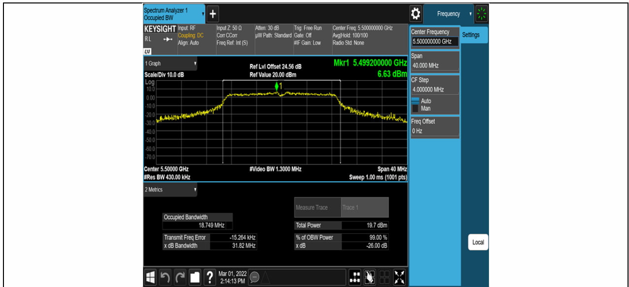
11AC20SISO_Ant2_5500
