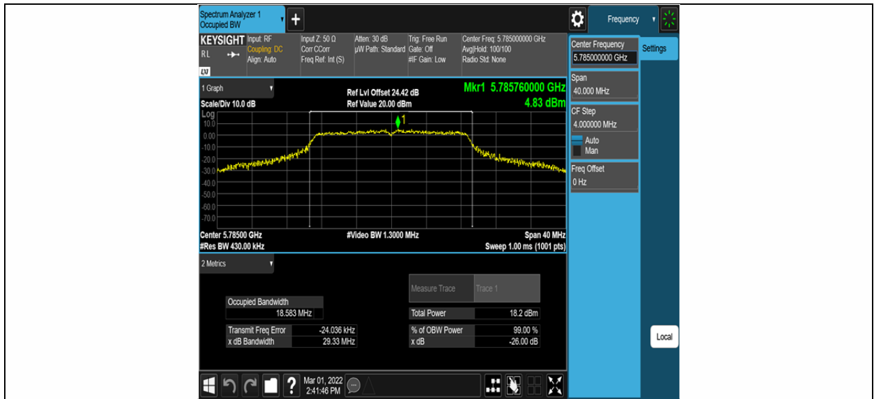
11AC20SISO_Ant2_5785
