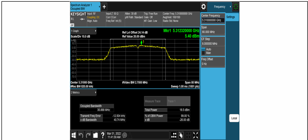
11N40SISO_Ant2_5310
