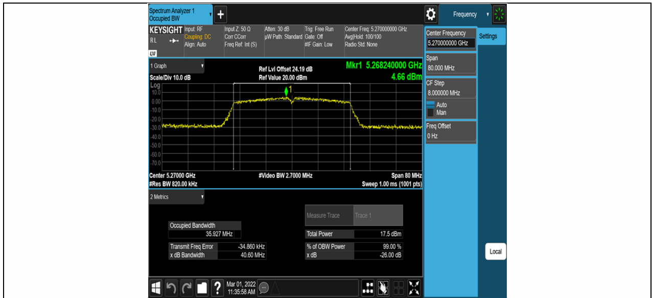
11N40SISO_Ant2_5270
