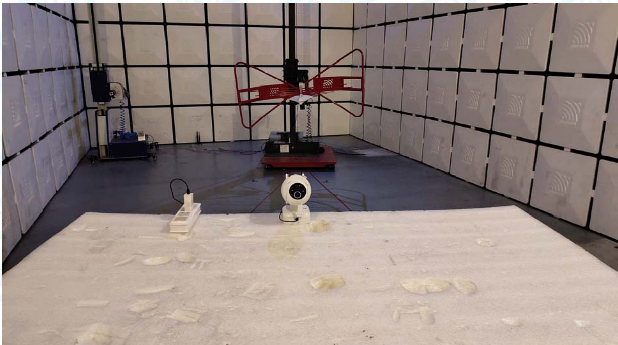
Photo of Setup for Radiated Emission (Below 1 GHz)
