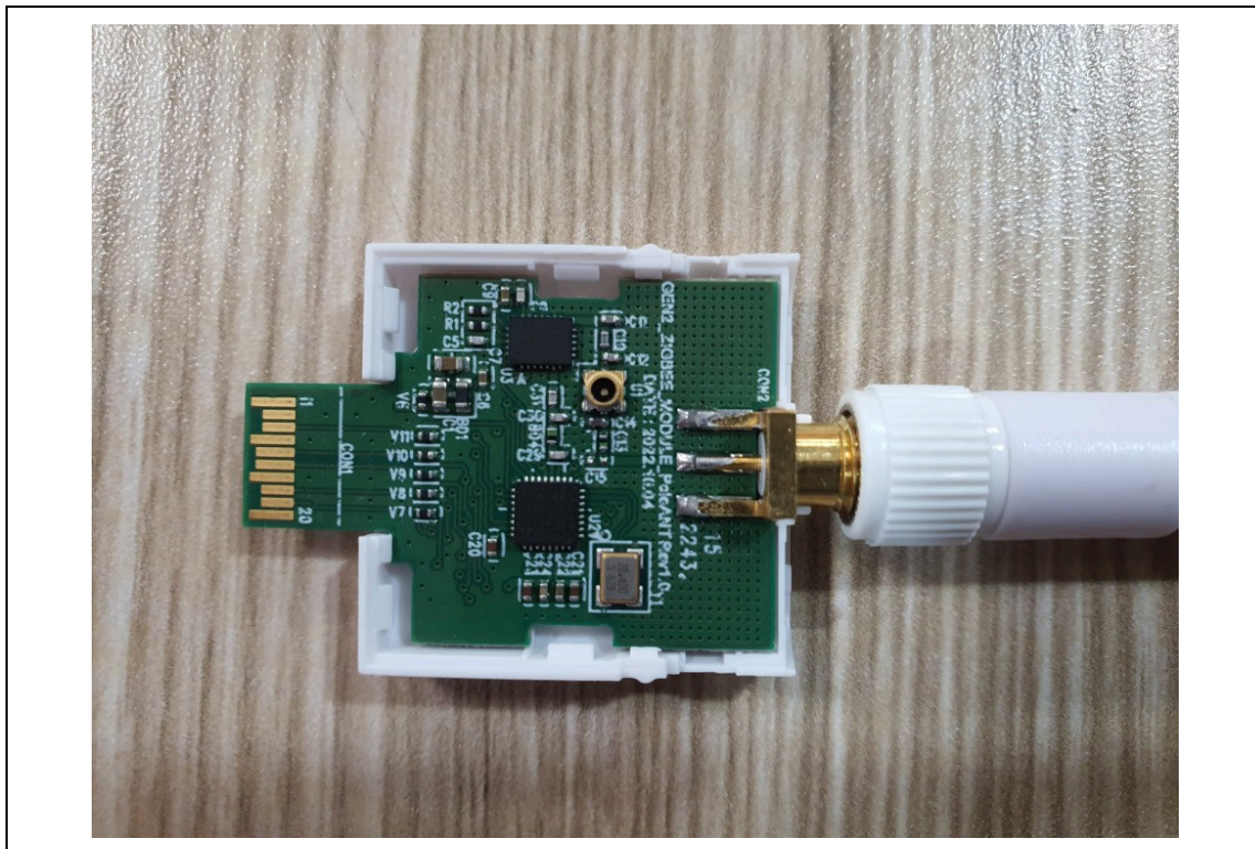
Board-Rear
