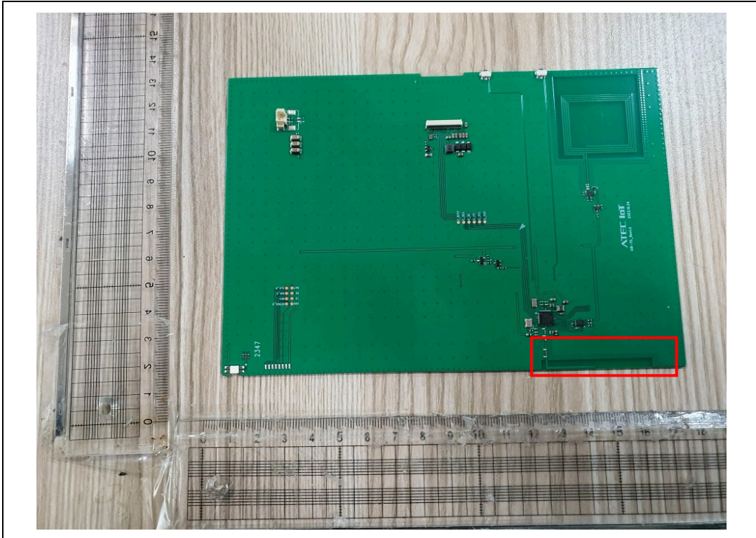
Antenna(2.4GHz ANT)
