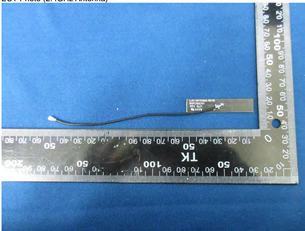
(50) EUT Photo (2.4GHz Antenna)
