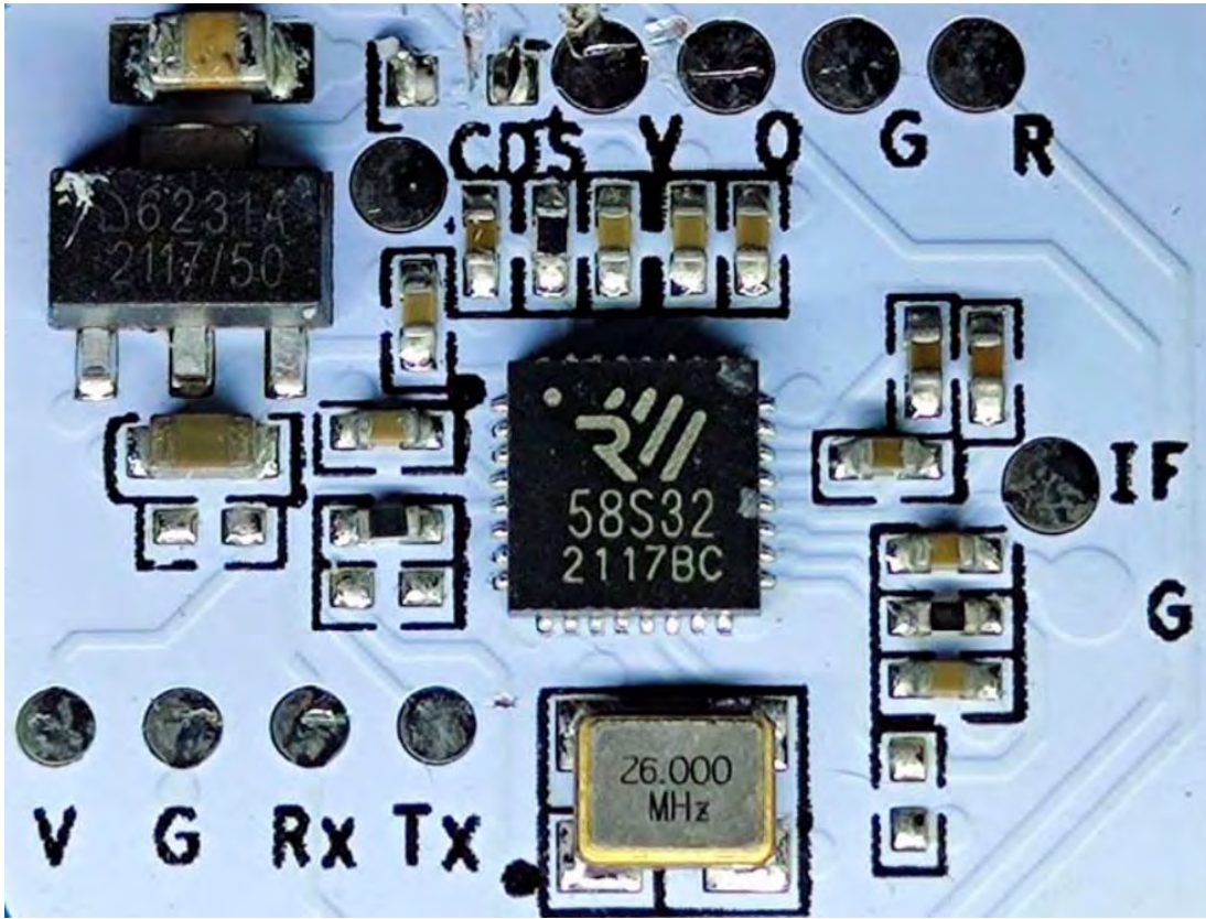
SRD Antenna
