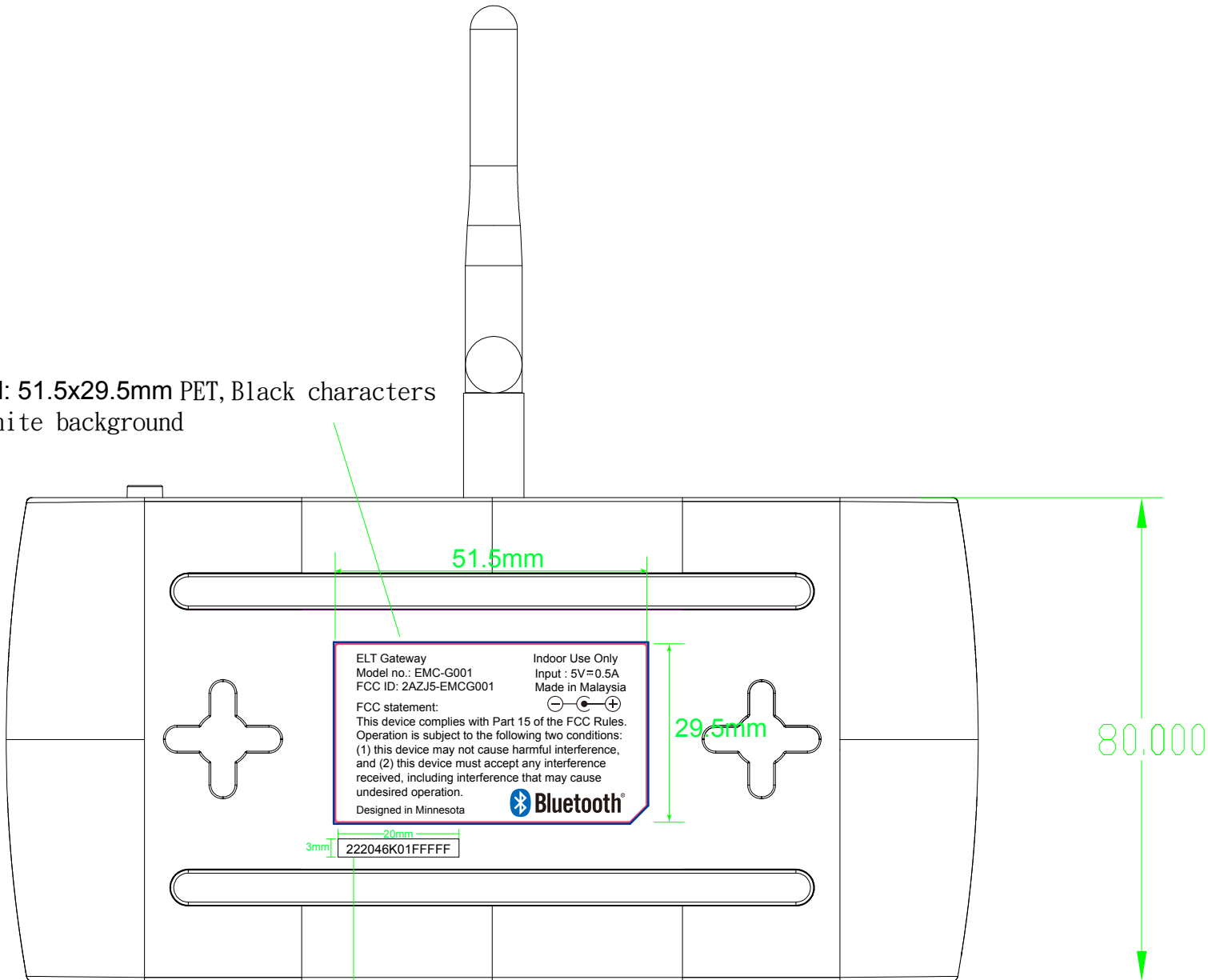
Label size : 20x3mm Material: PET,Black characters on white background 222046K01FFFFF
