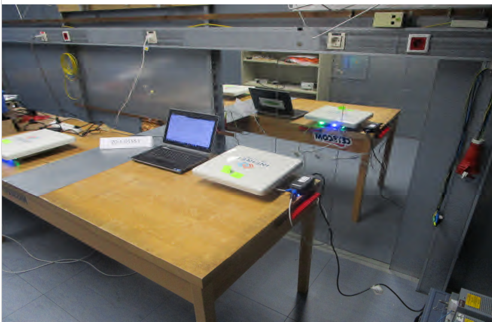
Photograph 5: EUT Test Setup, AC-Power Lines Conducted Emissions measurement
