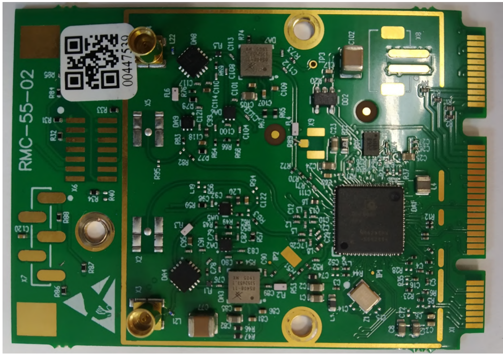
View of board radio module RMC 55-02
