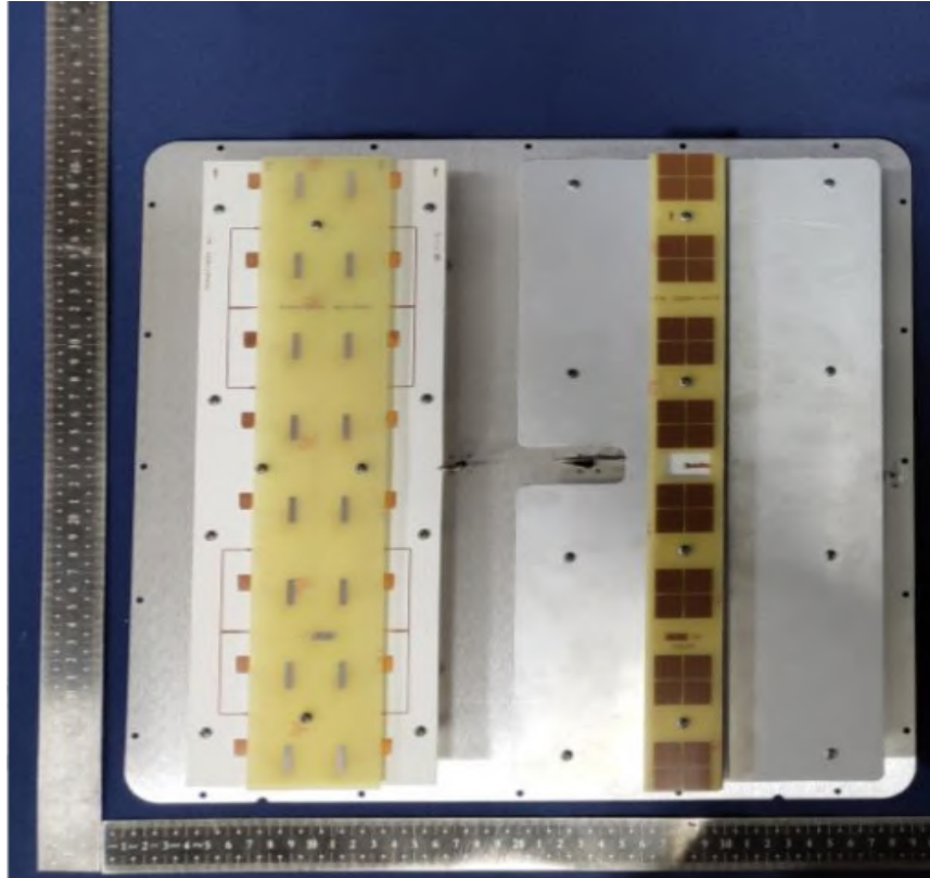
Internal view of integrated antenna model of MT – 464047/SVH
