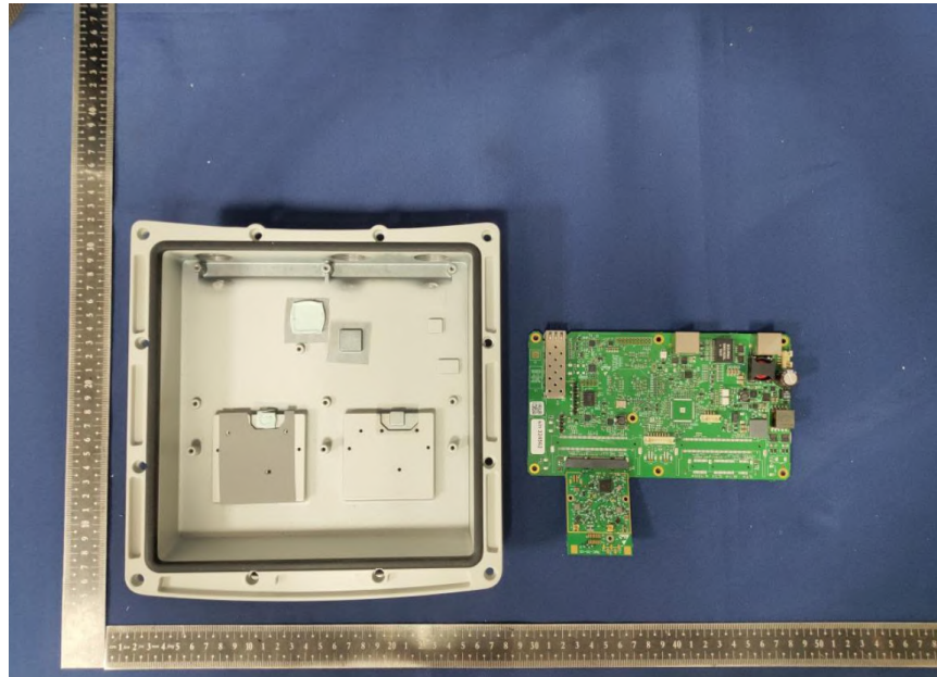
Internal view enclosure of equipment
