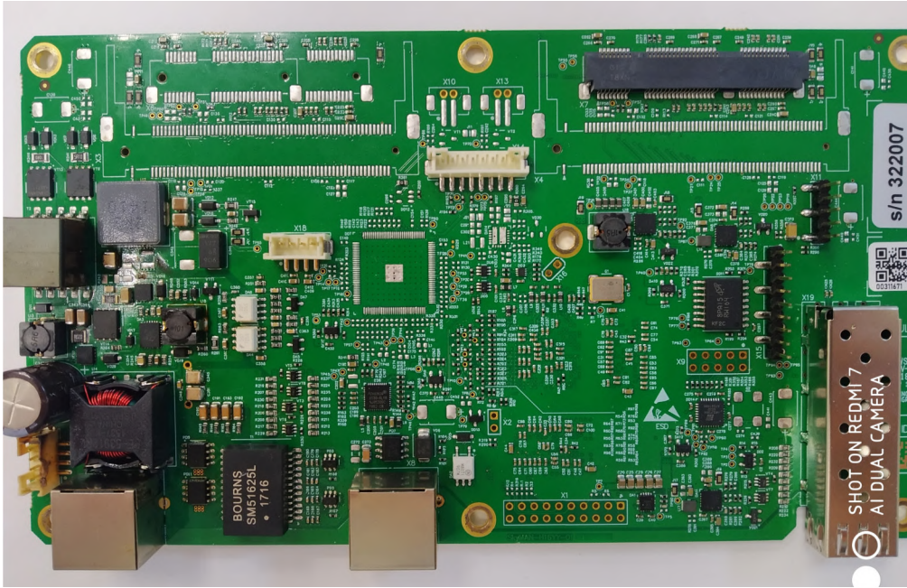
View of main board H16
