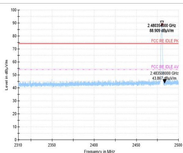
Bandedge:Ch39
