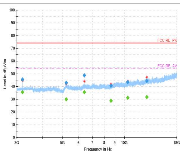
Radiated emission: Ch39, 3GHz~18GHz
