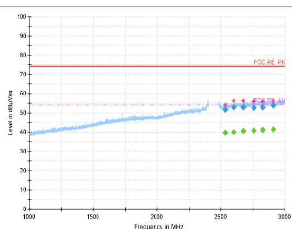
Bandedge:Ch39
