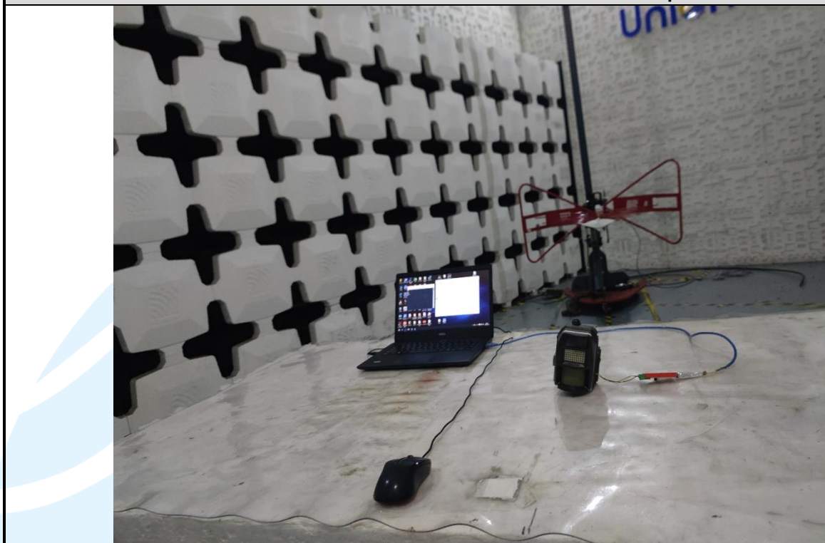
Radiated emission 30MHz to 1GHz Test Setup
