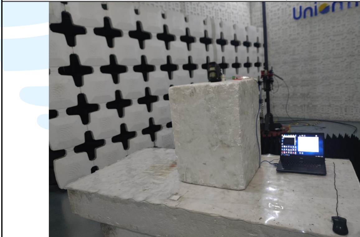
Radiated emission Above 1GHz Test Setup
