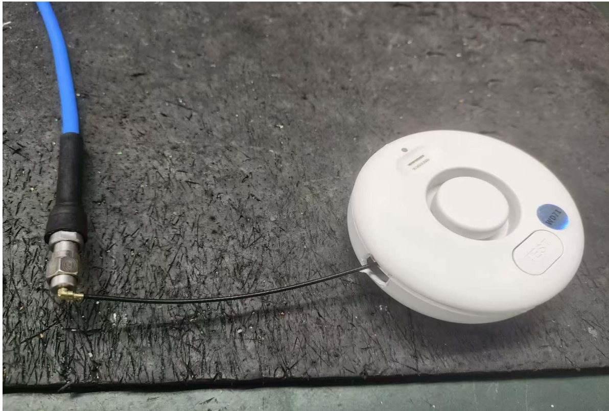
monopole antenna
