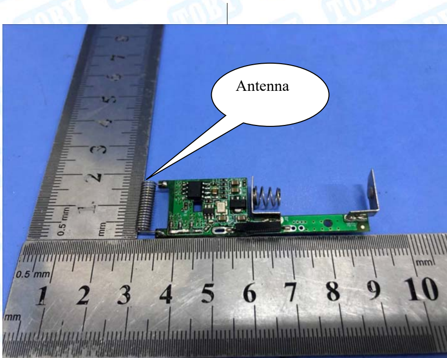
Photo 7 Appearance of PCB
