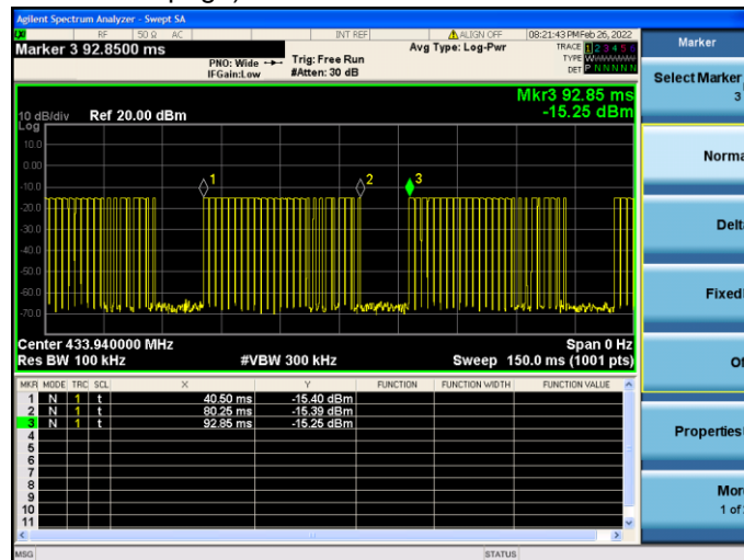
(Transmit cycle 52.35ms)
