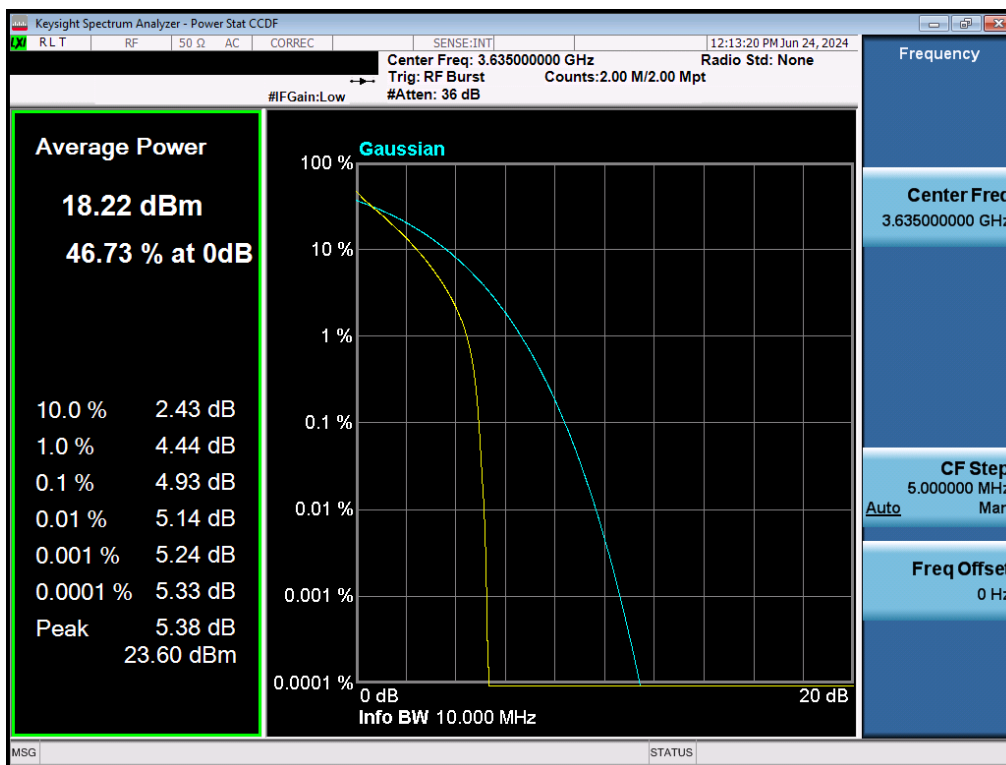
Plot 7.41. Peak to Average Power Ratio Plot (10MHz, QPSK – Mid Channel)
