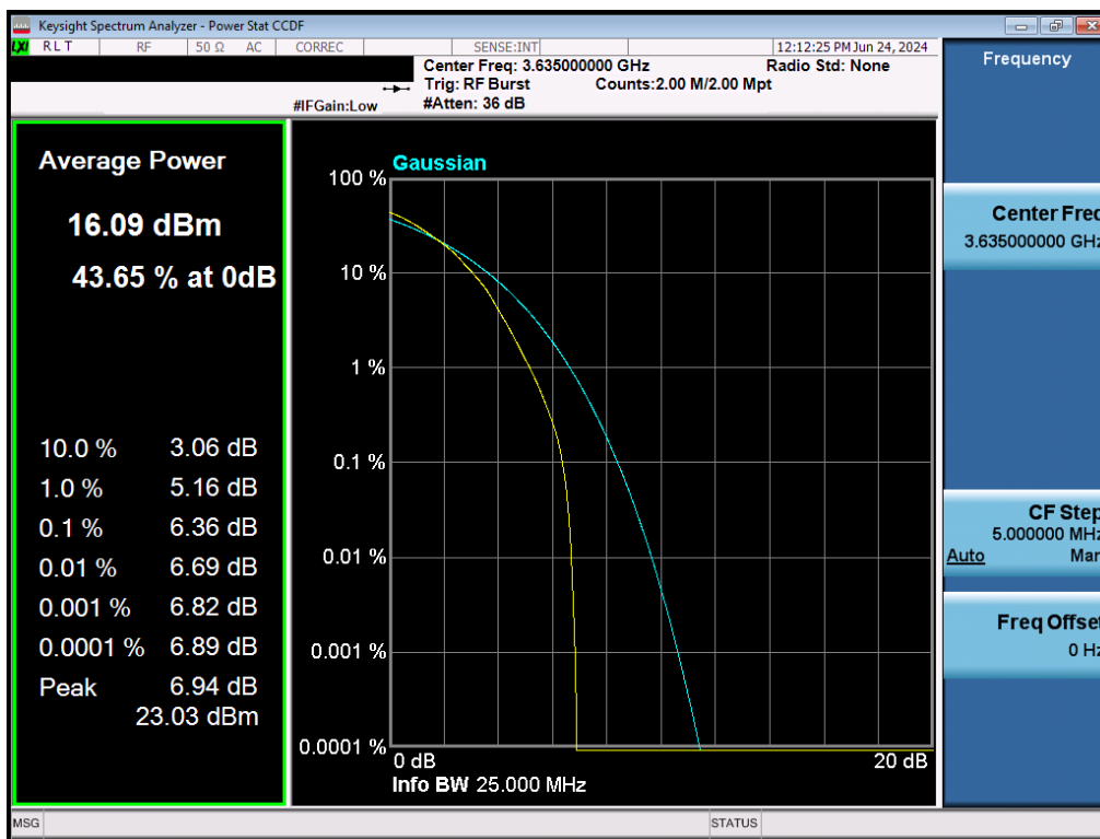
Plot 7.38. Peak to Average Power Ratio Plot (20MHz, 256QAM – Mid Channel)
