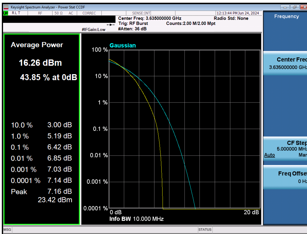
Plot 7.42. Peak to Average Power Ratio Plot (10MHz, 256QAM – Mid Channel)
