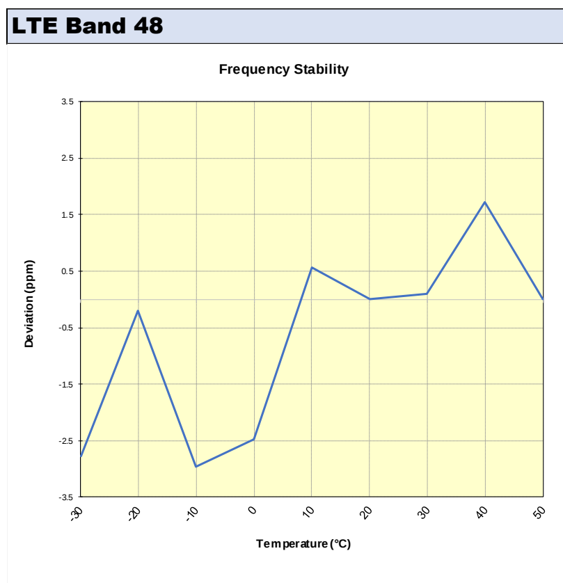
Plot 7.55. Frequency Stability Chart
