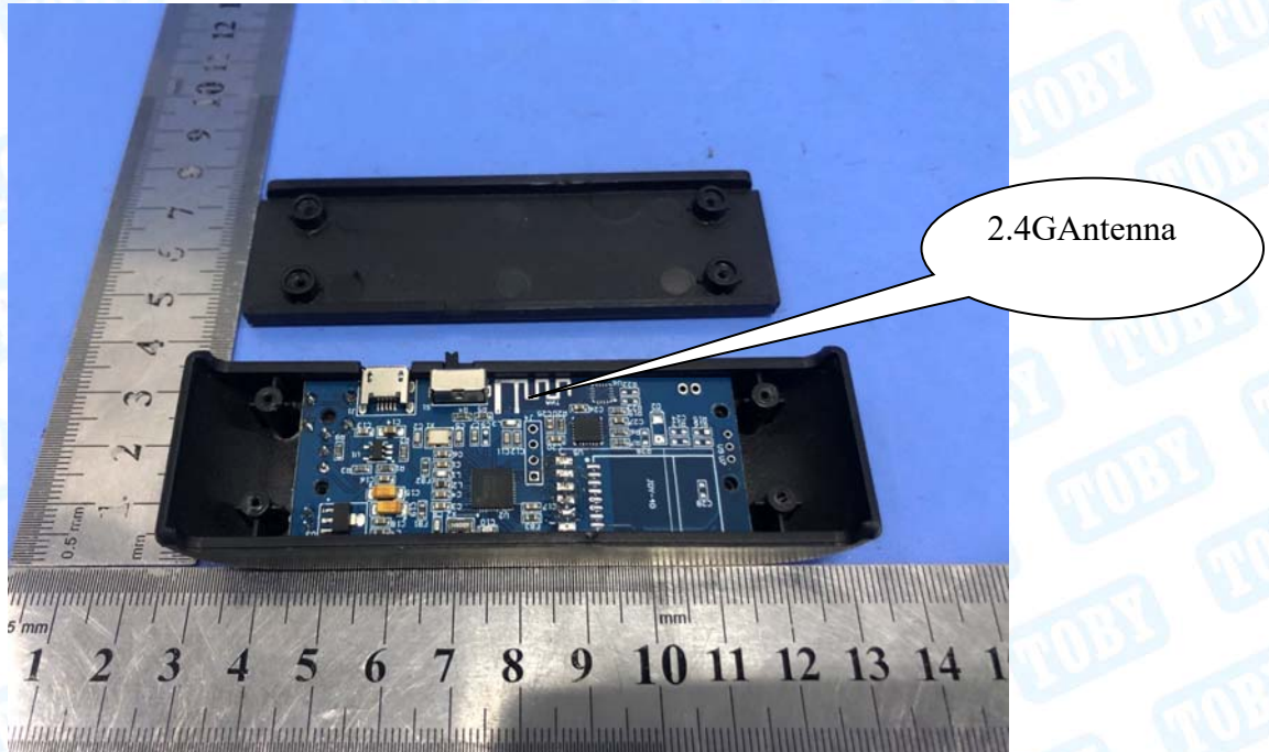
Photo 9 Appearance of PCB&Batttery
