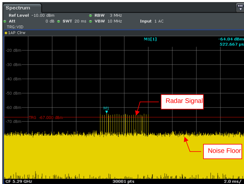
Radar Signal 2
