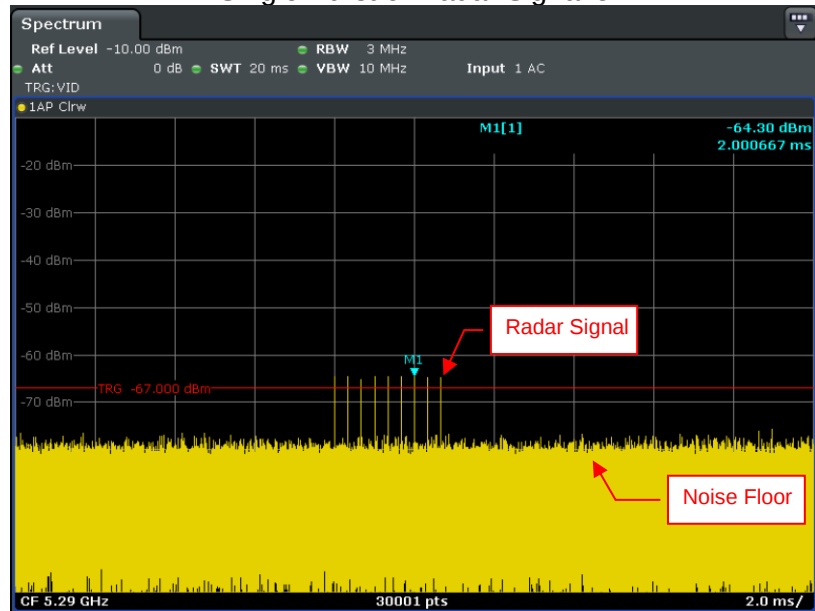
Radar Signal 6
