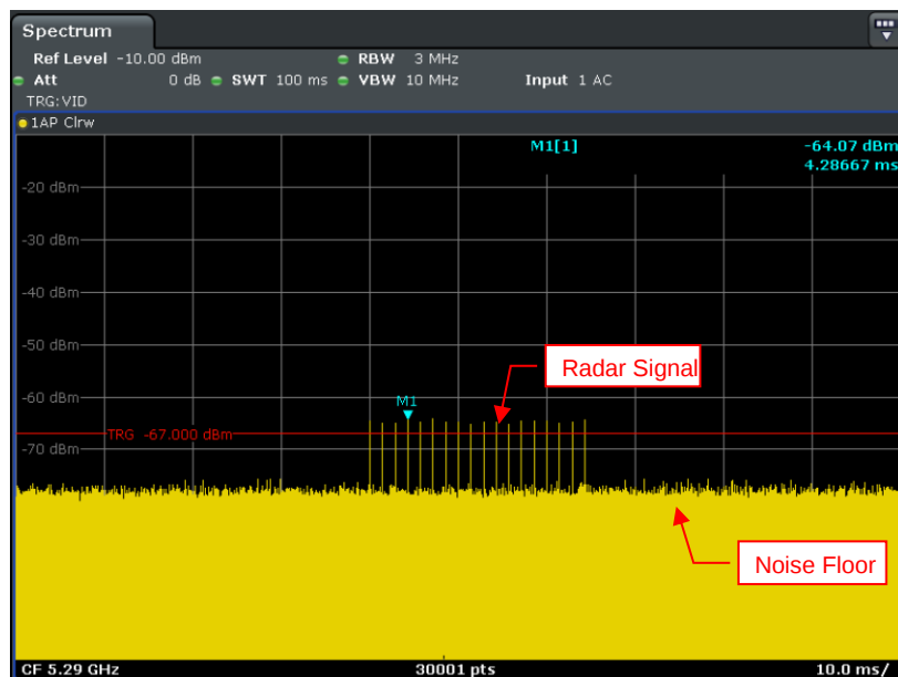
Radar Signal 0
