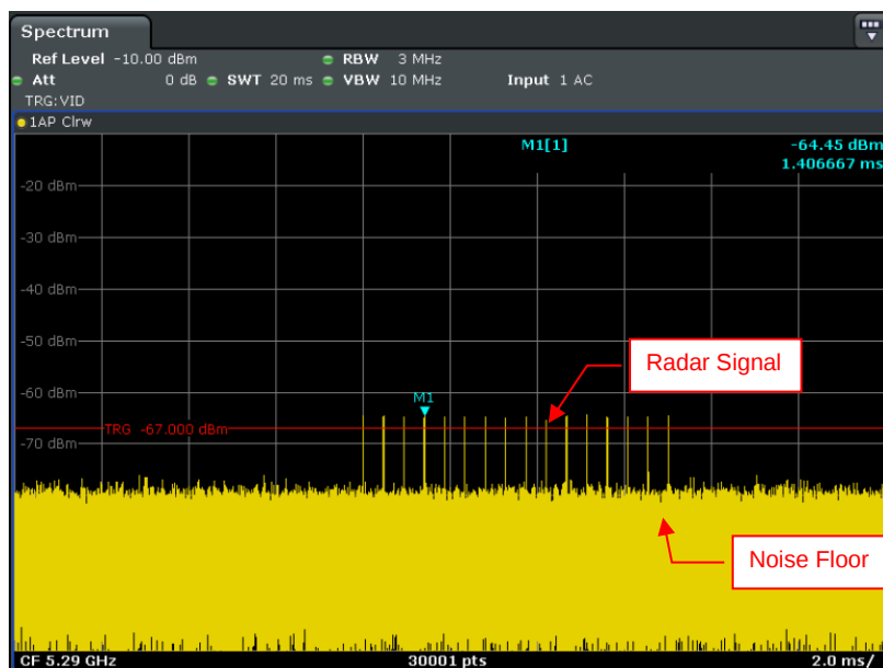
Radar Signal 2
