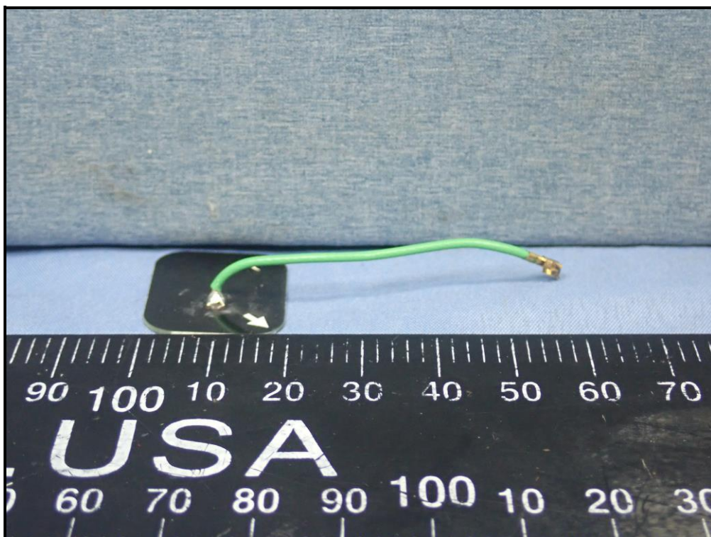
Ant 8:5G (High Band) Chain0
