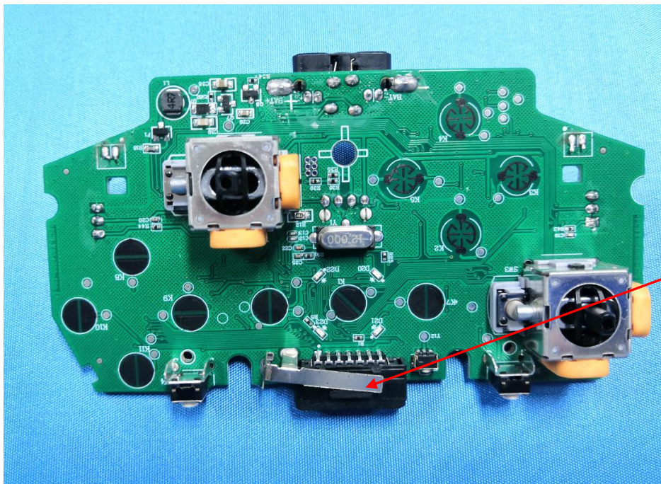
Metal Antenna
