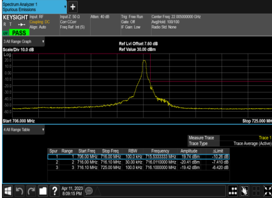
N12(10M)_DFT-s- OFDM_QPSK_Edge_1RB_Right_High_CH
