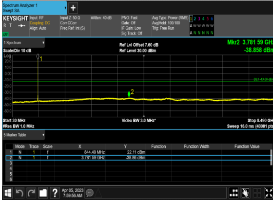
N5(5M)_DFT-s-OFDM_QPSK_Edge_1RB_Left_High_CH
