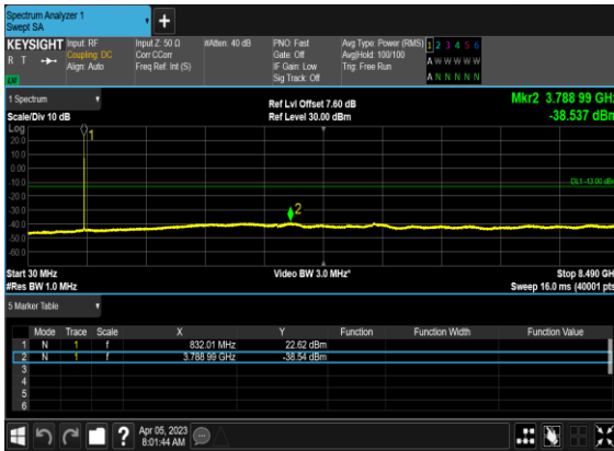
N5(10M)_DFT-s-OFDM_QPSK_Edge_1RB_Left_Mid_CH
