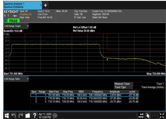
N12(15M)_DFT-s- OFDM_QPSK_Outer_Full_High_CH
