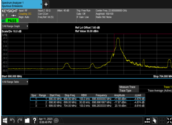
N12(5M)_DFT-s-OFDM_QPSK_Edge_1RB_Left_Low_CH
