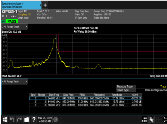
N5(5M)_DFT-s-OFDM_QPSK_Edge_1RB_Right_High_CH
