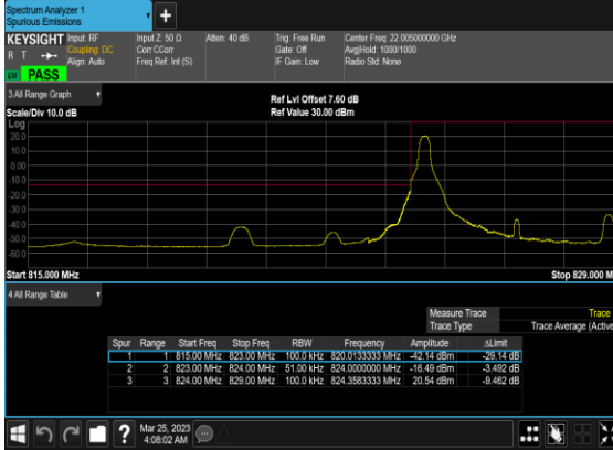
N5(5M)_DFT-s-OFDM_QPSK_Edge_1RB_Left_Low_CH
