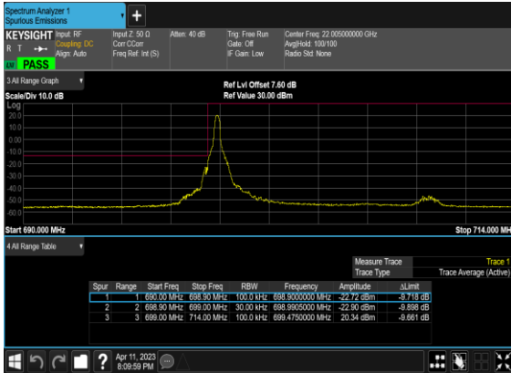
N12(15M)_DFT-s- OFDM_QPSK_Edge_1RB_Left_Low_CH
