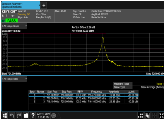
N12(15M)_DFT-s- OFDM_QPSK_Edge_1RB_Right_High_CH
