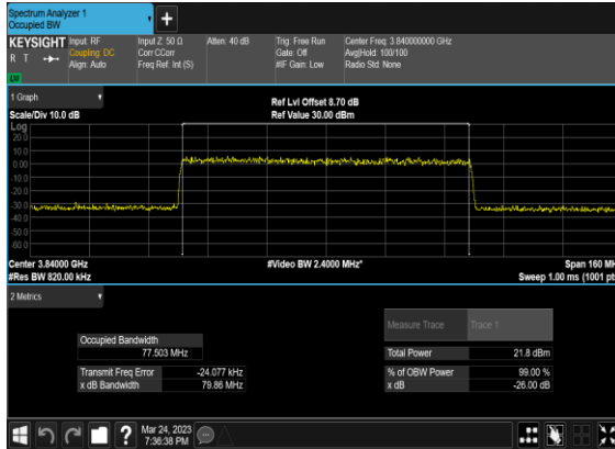
N77(80M)_CP-OFDM_256 QAM_Outer_Full_Mid_CH
