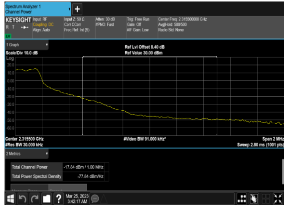
N30(10M)_DFT-s- OFDM_QPSK_Edge_1RB_Right_Low_CH_CHP_P ASS
