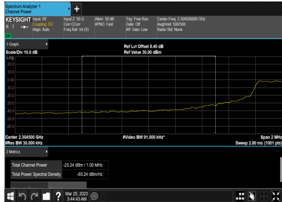
N30(10M)_DFT-s- OFDM_QPSK_Outer_Full_Low_CH_CHP_PASS
