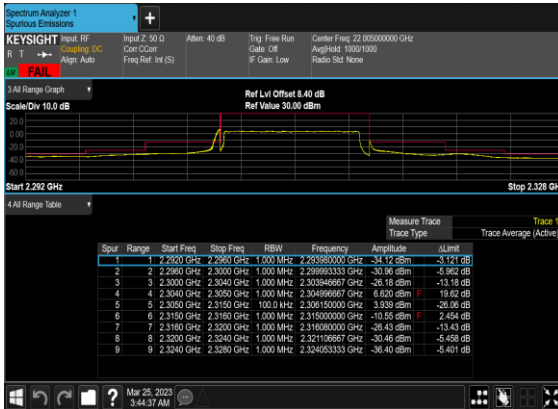
N30(10M)_DFT-s- OFDM_QPSK_Outer_Full_Low_CH
