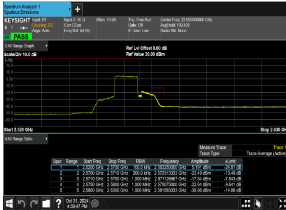
B5_N7(10M)_DFT-s-OFDM_QPSK_Outer_Full_High_CH
