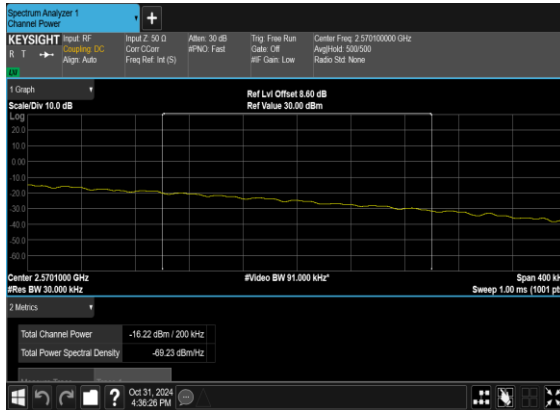
B5_N7(10M)_DFT-s-OFDM_BPSK _Edge_1RB_Right_High_CH_CHP_PASS
