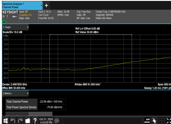
B5_N7(20M)_DFT-s-OFDM_QPSK Edge_1RB_Left_Low_CH_CHP_PASS
