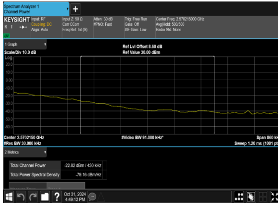
B5_N7(20M)_DFT-s-OFDM_BPSK _Edge_1RB_Right_High_CH_CHP_PASS
