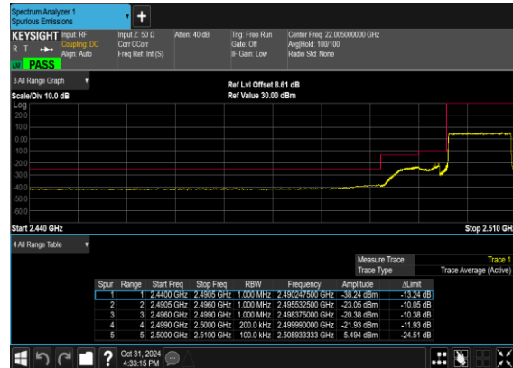
B5_N7(10M)_DFT-s- OFDM_BPSK_Outer_Full_Low_CH
