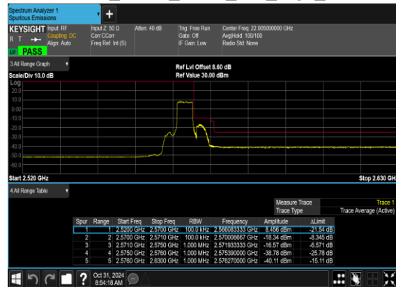
B5_N7(5M)_DFT-s- OFDM_BPSK_Outer_Full_High_CH
