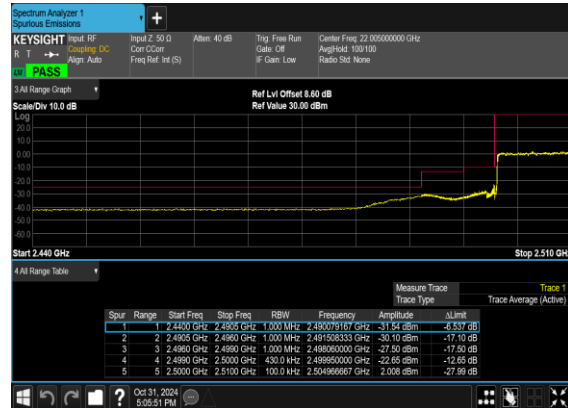
B5_N7(20M)_DFT-s-OFDM_BPSK_Outer_Full_Low_CH
