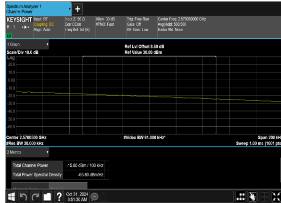
B5_N7(5M)_DFT-s-OFDM_BPSK _Edge_1RB_Right_High_CH_CHP_PASS
