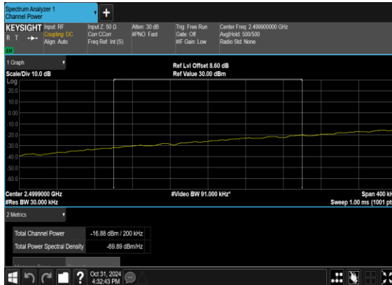
B5_N7(10M)_DFT-s-OFDM_QPSK Edge_1RB_Left_Low_CH_CHP_PASS
