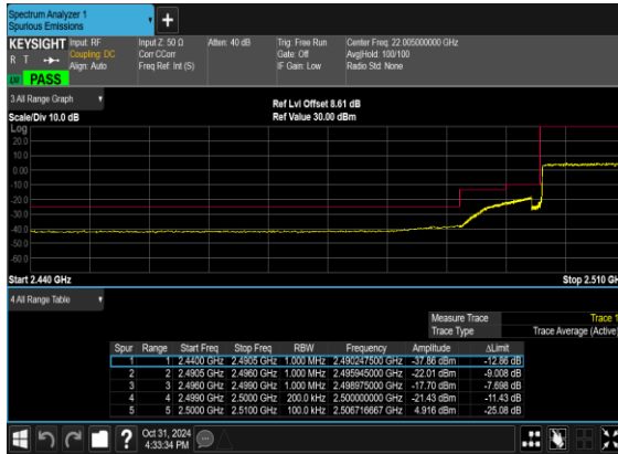
B5_N7(10M)_DFT-s- OFDM_QPSK_Outer_Full_Low_CH
