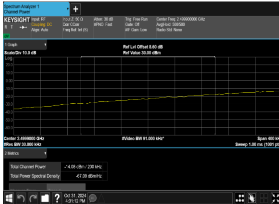
B5_N7(10M)_DFT-s-OFDM_BPSK Edge_1RB_Left_Low_CH_CHP_PASS
