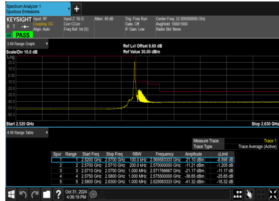
B5_N7(10M)_DFT-s- OFDM_BPSK_Edge_1RB_Right_High_CH
