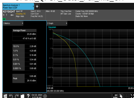
B2_N5(20M)_DFT-s-OFDM_QPSK_Outer_Full_Mid_CH
