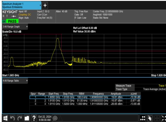
N2(5M)_DFT-s- OFDM_QPSK_Edge_1RB_Right_High_CH
