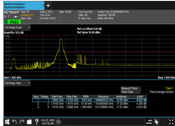
N2(5M)_DFT-s- OFDM_BPSK_Edge_1RB_Right_High_CH
