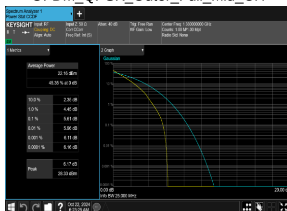
N2(20M)_DFT-s-OFDM_QPSK_Outer_Full_Mid_CH
