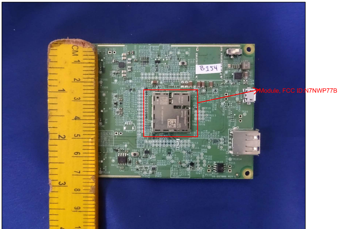
PCB Dimensional View
