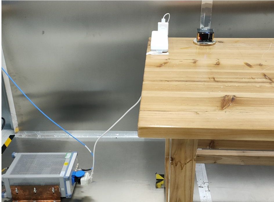
Photograph 4: Set-up for Radiated Emissions, below 1GHz
